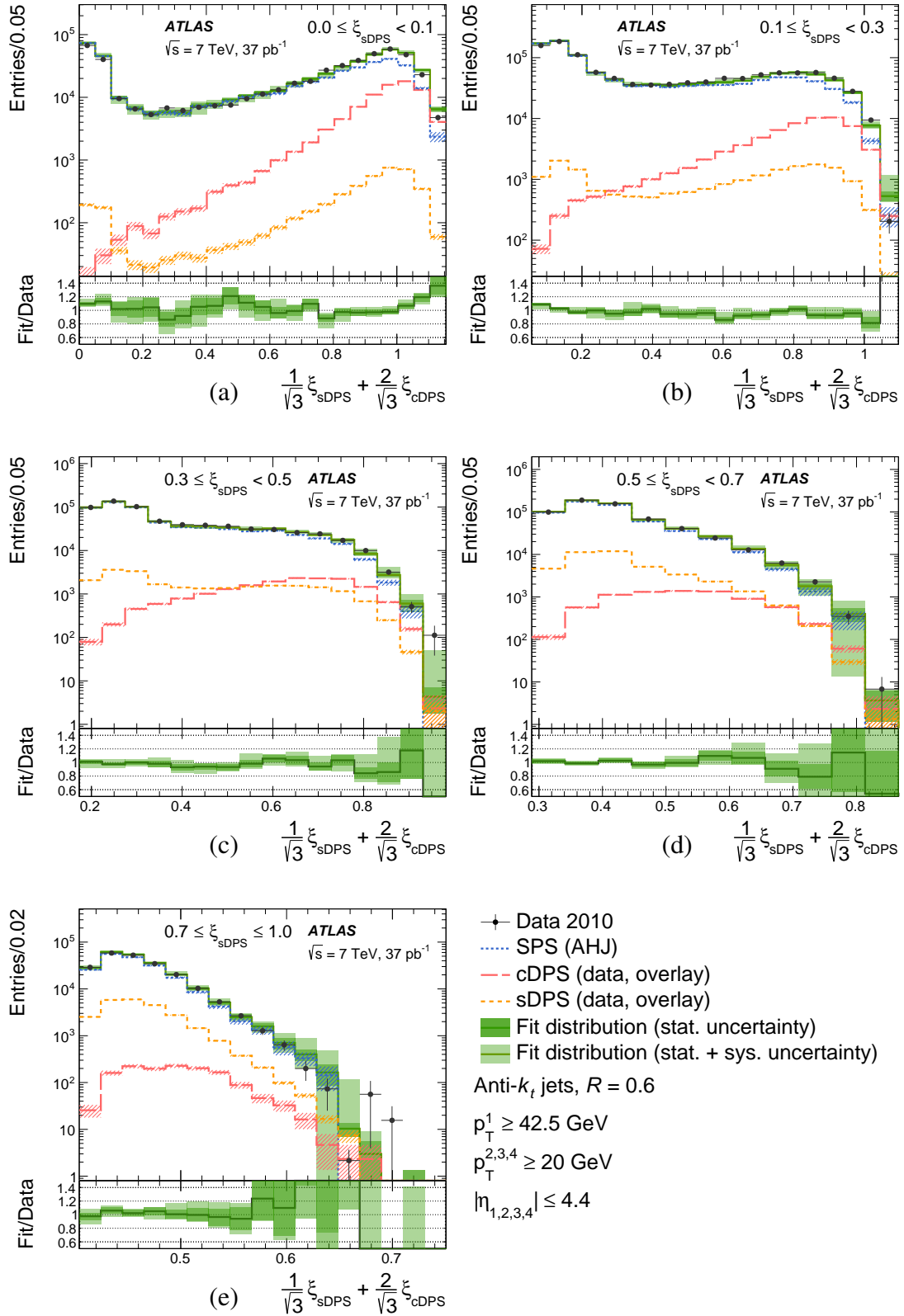
Figure 6: Distributions of the NN outputs, \frac{1}{\sqrt{3}} \xi_{\text{sDPS}} + \frac{2}{\sqrt{3}} \xi_{\text{cDPS}} , in the \xi_{\text{sDPS}} ranges indicated in the panels, for four-jet events in data, selected in the phase space defined in the legend, compared to the result of fitting a combination of the SPS, cDPS and sDPS contributions, the sum of which is shown as the solid line. In the fit distribution, statistical uncertainties are shown as the dark shaded area and the light shaded area represents the sum in quadrature of the statistical and systematic uncertainties. The ratio of the fit distribution to the data is shown in the bottom panels.
