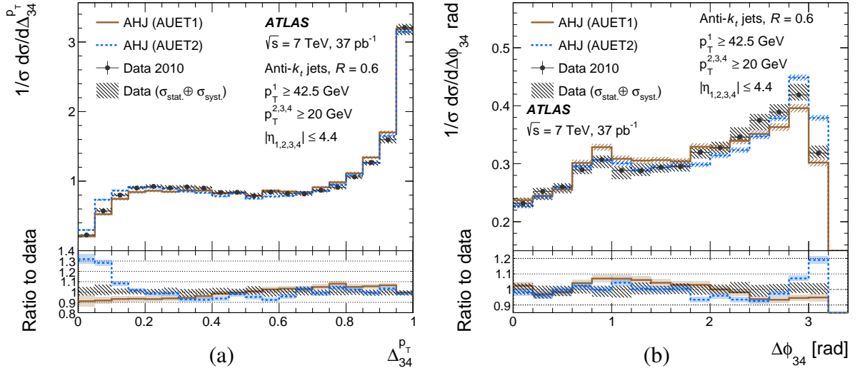
Figure 10: Distributions of the variables (a) \Delta_{34}^{p_T} and (b) \Delta\phi_{34} , defined in Eq. (16), in data after unfolding to particle level, compared to the MC prediction from AHJ at the particle level, generated using the AUET1 and AUET2 tunes, as indicated in the legend. The hatched area represents the sum in quadrature of the statistical and systematic uncertainties in the normalized differential cross-sections and all histograms are normalized to unity. The ratio of the particle-level distribution to the normalized differential cross-section is shown in the bottom panels, where the shaded areas represent statistical uncertainties.
