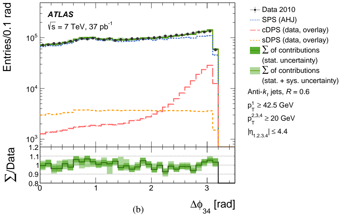
Figure 7: Comparison between the distributions of the variables (a) \Delta_{34}^{p_T} and (b) \Delta\phi_{34} , defined in Eq. (16), in four-jet events in data and the sum of the SPS, cDPS and sDPS contributions, as indicated in the legend. The sum of the contributions is normalized to the cross-section measured in data and the various contributions are normalized to their respective fractions obtained from the fit. In the sum of contributions, statistical uncertainties are shown as the dark shaded area and the light shaded area represents the sum in quadrature of the statistical and systematic uncertainties. The ratio of the sum of contributions to the data is shown in the bottom panels.
