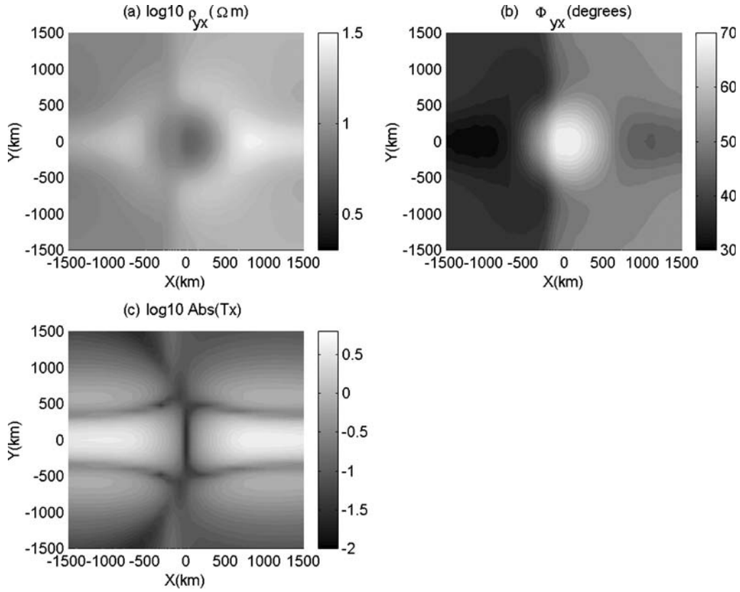
Figure 9. Response to the external field \vec{H}^{(ext1)} 3-D+.
