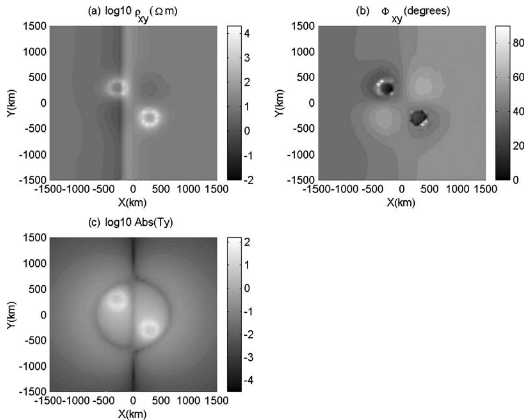
Figure 15. Response to the external field \vec{H}^{(ext2)} 3-D–.
