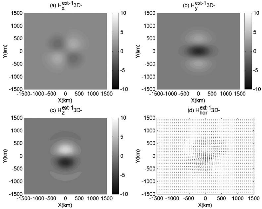
Figure 8. Spatial dependence of the second 3-D \vec{H}^{(ext1)} 3-D-, at the Earth's surface. The x component is an odd function of x and y plus a constant, and its value outside the anomalous zone has been normalized to 1.
