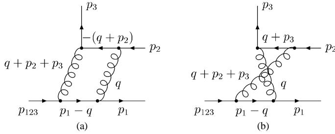
Fig. 1. One-loop diagrams contributing to the antisymmetric component of the splitting matrix S_{p_{q_1 \bar{q}_2 Q_3}} .
