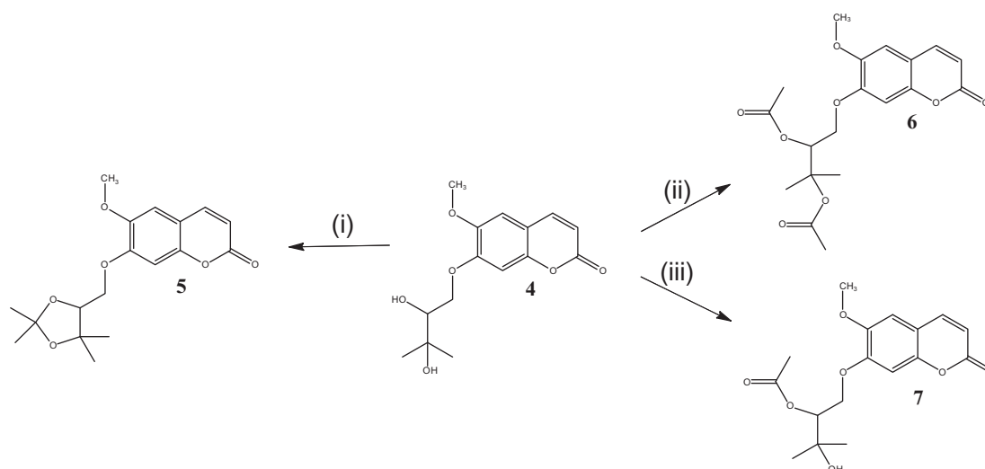
Scheme 1. Reagents and conditions: (i) \text{H}_2\text{SO}_4 , acetone, rt; (ii) 2.3 equiv \text{Ac}_2\text{O} , Py, DMAP, rt; (iii) 1.0 equiv \text{Ac}_2\text{O} , Py, 0 °C–rt.
