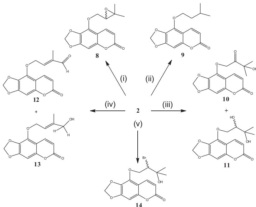
Scheme 2. Reagents and conditions: (i) m -CPBA, K_2CO_3 , Cl_2CH_2 , 0^\circ C and dark conditions; (ii) H_2 , Pd/C, Cl_2CH_2 , rt; (iii) 1.1 equiv KMnO_4 , THF/ H_2O (7:3), diethyl-ammonium fluoride, rt; (iv) 0.75 equiv SeO_2 , Cl_2CH_2 , 2.0 equiv TBHP, 0-4^\circ C ; (v) 2.2 equiv NBS, Cl_2CH_2 , 0-4^\circ C .
