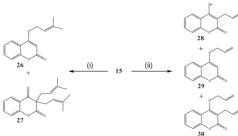
Scheme 5. Reagents and conditions: (i) 2.0 equiv \gamma,\gamma -dimethylallyl bromide, 1.5 equiv NaH, DMF, rt; (ii) 2.0 equiv allyl bromide, 1.5 equiv NaH, DMF, -20^\circ\text{C} .
