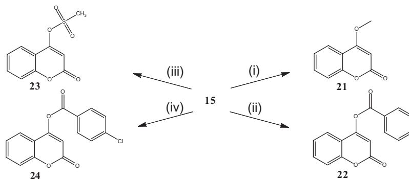
Scheme 3. Reagents and conditions: (i) Me_2SO_4 , K_2CO_3 , acetone, 56^\circ C ; (ii) BzOCl , TEA, Cl_2CH_2 , rt; (iii) 1.3 equiv MsCl , 1.2 equiv Py, 0.6 equiv DMAP, Cl_2CH_2 , rt; (iv) 4-chlorobenzoyl chloride, TEA, Cl_2CH_2 , rt.
