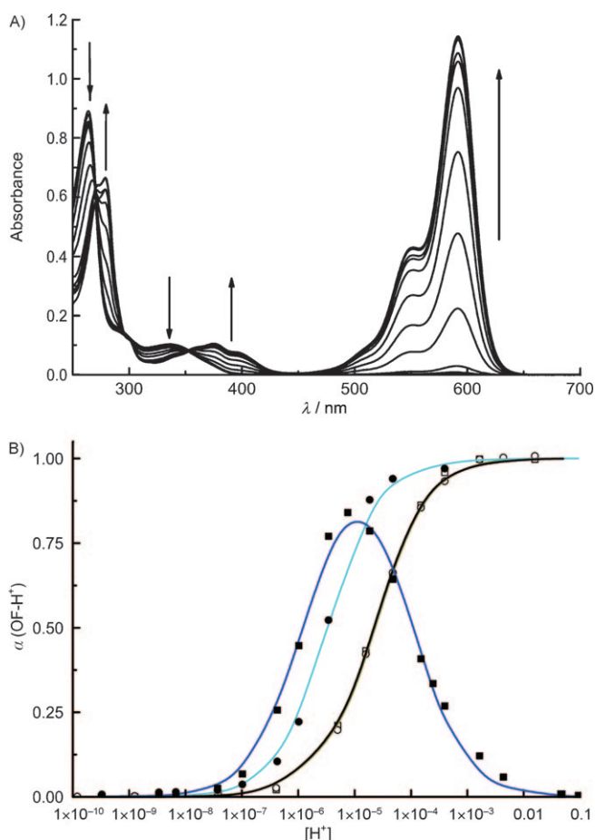
Figure 4. A) Effect of pH on the equilibrium shown in Scheme 6 for compound 1g . The arrows display the direction of the changes as the proton concentration was increased (the pH was decreased from 12 to 2). B) pH speciation diagram for the colored forms of compound 1a ( \square , —), 1d ( \blacksquare , —), 1e ( \bullet , —), and 1g ( \circ , —). The symbols correspond to measured data and the lines are best fits obtained by considering one (compound 1e ) or two equilibrium constants (compounds 1a , 1d and 1g ).
