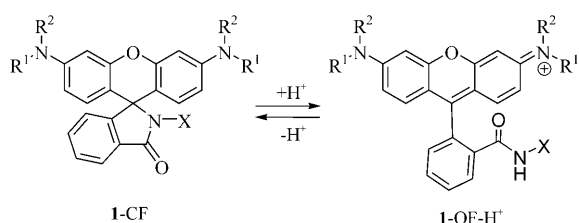
Scheme 6. Protonation-mediated ring-opening reaction of RSAs in water.
