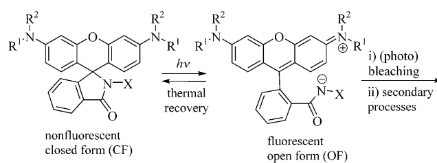
Scheme 1. Photochromic (caged) RSAs in the colorless CF and colored OF forms.
