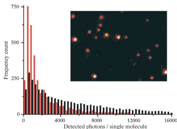
Figure 5. Histograms of the number of photons per single-molecule event for compound 1c (black bars) and compound 1f (red bars). The inset shows a typical frame from the CCD camera, from which single-molecule events were localized.
