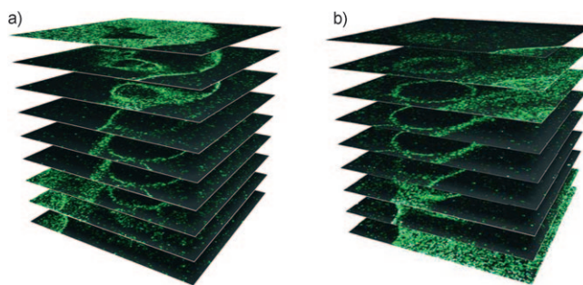
Figure 6. Optical sections of lamin proteins in the nucleus of a U373MG cell imaged by using 2PA with \lambda=747 nm light; field of view: 12.5\times 12.5 \mu\text{m} ; pixel size: 30 nm; distance between z stacks \approx 600 nm. Nuclear lamina of whole fixed human glioma cells, U373M, were stained with antilamin A mouse IgG as a primary antibody and sheep anti-mouse IgG labeled with N -hydroxysulfosuccinimidyl ester 20d ( n=1 ) as a secondary antibody.
