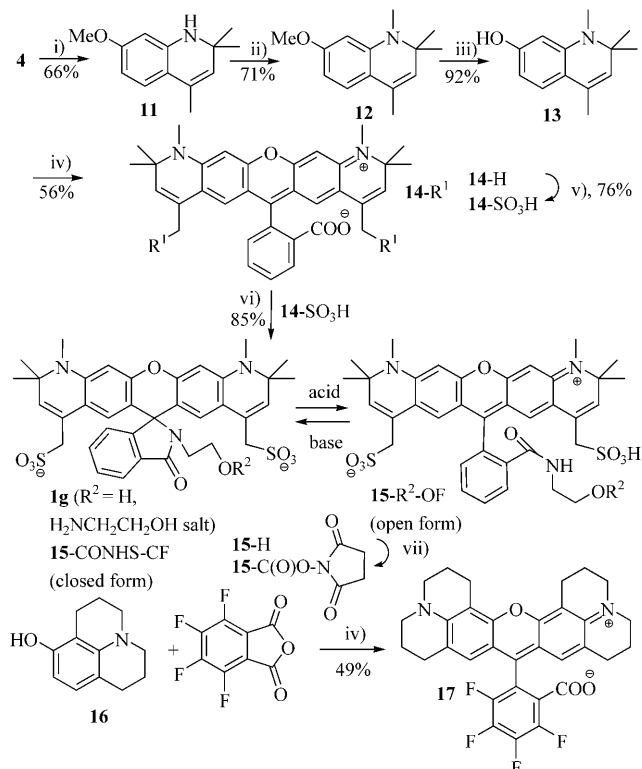
Scheme 4. Synthesis of rhodamines 1g (15) and 17 , which absorb at \lambda \approx 600 nm and emit at \lambda \approx 620 nm. Conditions: i) acetone, Y(OTf) 3 (5 mol %), 24 h, RT; ii) MeI, Cs 2 CO 3 , DMF, 90 °C, 3 h; iii) 48% aqueous HBr, AcOH, reflux, 6 h; iv) p -TosOH, EtCOOH, 160 °C, 24 h; v) 96% H 2 SO 4 , 0 °C to RT, overnight; vi) H 2 NCH 2 CH 2 OH; HATU, Et 3 N, DMF, 40–50 °C, overnight; vii) di( N -succinimidyl)carbonate, Et 3 N, MeCN, CH 2 Cl 2 , 50 °C, 2 h.
