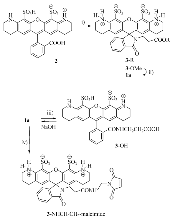
Scheme 2. Synthesis of primary aliphatic amides of sulfonated rhodamines with a rigidized xanthene fragment. Conditions: i) N,N,N',N' -tetramethyl- O -( N -succinimidyl)uronium·BF 4 - (TSTU), Et 3 N, DMF ( N,N -dimethylformamide), RT, overnight; HCl·H 2 NCH 2 CH 2 COOMe, Et 3 N, DMF, RT, overnight, 38–66%; ii) aqueous NaOH (0.1–0.15 M), RT, 2 h, 100%; iii) Amberlite IR-120 (H + form); iv) N -(2-aminoethyl)maleimide trifluoroacetate, O -(7-azabenzotriazol-1-yl)- N,N,N',N' -tetramethyluronium·PF 6 - (HATU), DMF, RT, overnight, 26%.
