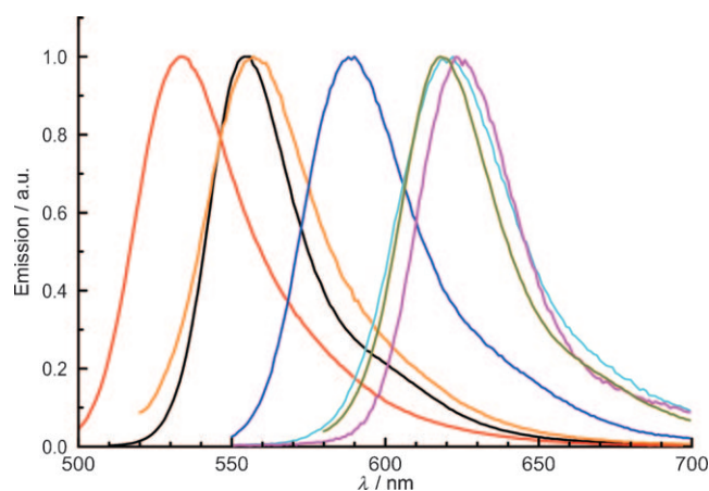
Figure 3. Emission spectra of the OFs ( 1-OF-H + in Scheme 6) of compounds 1a–g in aqueous solutions: 1a : —; 1b : —; 1c : —; 1d : —; 1e : —; 1f : —; 1g : —.
