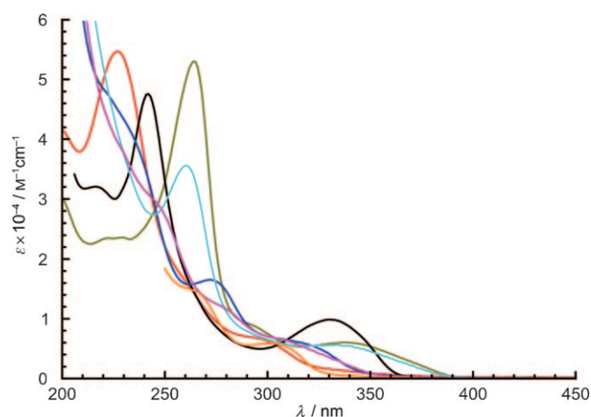
Figure 2. Absorption spectra of compounds 1a–g in water. 1a : —; 1b : —; 1c : —; 1d : —; 1e : —; 1f : —; 1g : —.
