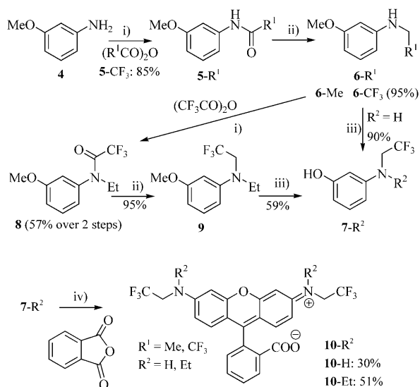
Scheme 3. Synthesis of rhodamines 10-R 2 with N,N' -bis(2,2,2-trifluoroethyl) groups. Conditions: i) pyridine, CH 2 Cl 2 , RT, overnight; ii) BH 3 ·THF (1M), THF, reflux, overnight; iii) 48% aqueous HBr, AcOH, reflux, 6 h; iv) 160 °C, 3 h, then portion 2 of 7-R 2 , 85% aqueous H 3 PO 4 , 160 °C, 3 h.
