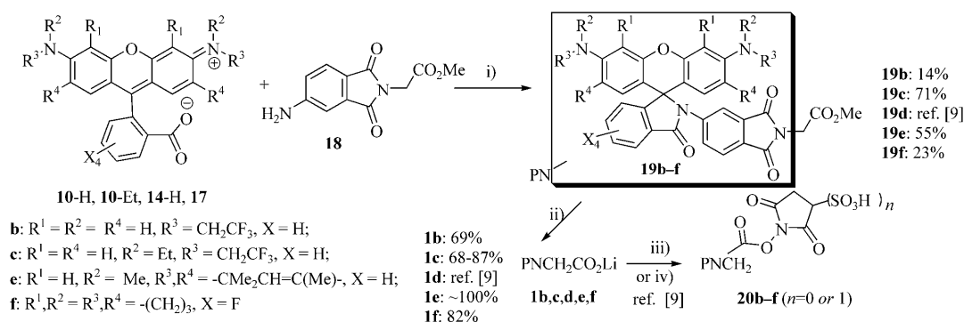
Scheme 5. Synthesis of methyl esters 19b–f and the corresponding lithium salts 1b–f . Conditions: i) \text{POCl}_3 , 1,2-dichloroethane, reflux, 4 h, then 18 , MeCN, \text{Et}_3\text{N} , reflux, overnight; ii) LiI, EtOAc or THF, reflux, 2 or 4 d; iii) N,N,N',N' -tetramethyl- O -( N -succinimidyl)uronium- \text{BF}_4^- , \text{Et}_3\text{N} , DMF, RT, overnight; iv) N -hydroxysulfosuccinimide, HATU, DMF, RT.
