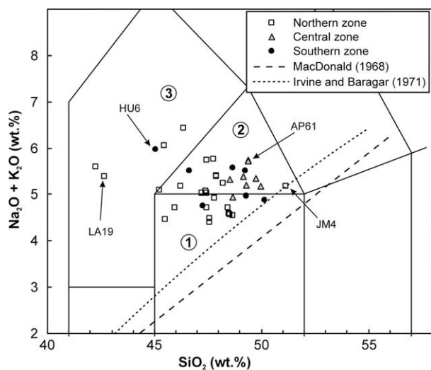
Fig. 3. Total alkali-silica diagram (Le Maitre et al., 1989) for the studied rocks. Fields: 1, basalts; 2, trachybasalts; 3, basanites/tefrites. Boundary line between alkaline and subalkaline fields after Macdonald (1968) (dashed straight line), and Irvine and Baragar (1971) (dotted curve). Samples: open squares, Northern Zone; gray-filled triangles, Central Zone; filled circles, Southern Zone. Arrows indicate xenoliths localities (LA19, HU6 and AP61) and a sample with possible upper crust contamination (JM4).
