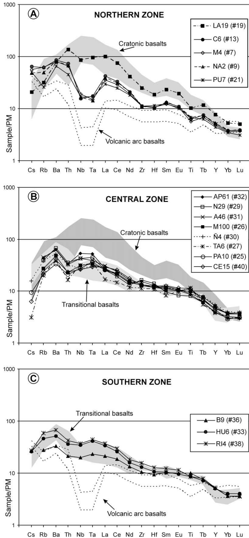
Fig. 6. Multi-element concentration patterns normalized to primitive mantle (Sun and McDonough, 1989). Following each sample number is indicated the number of the locality in Fig. 2. (A) Rocks from the Northern Zone (LA19, C6, NA2, M4 and PU7), compared with Cratonic basalts of Patagonia and Andean volcanic arc basalts. (B) Rocks from the Central Zone (M100, N29, Ñ4, AP61, A46, TA6 and PA10 also included an unpublished analysis of a Miocene lava flow, CE15), compared with basalts from Cratonic and Transitional settings of Patagonia. (C) Rocks from the Southern Zone (HU6, RI4 and B9) compared with Cratonic basalts of Patagonia and Andean volcanic arc basalts. Values of Cratonic and Transitional basalts after Stern et al. (1990, and references therein), and values of Andean volcanic arc basalts are of Llaima volcano (Hickey et al., 1986).
