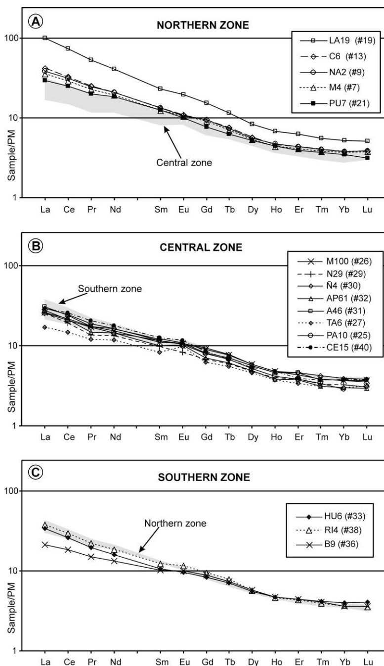
Fig. 5. REE concentrations normalized to primitive mantle (Sun and McDonough, 1989) of the rocks studied. Following each sample number is indicated the number of the locality in Fig. 2. (A) Northern Zone (LA19, C6, NA2, M4 and PU7), for comparison is included the field of variation of rocks from the Central Zone. (B) Central Zone, (M100, N29, N4, AP61, A46, TA6 and PA10) included is an unpublished analysis of a Miocene lava flow (CE15) and the field of variation of rocks from the Southern Zone. (C) Southern Zone (HU6, RI4 and B9) compared with the range of variation of rocks from the Central Zone (shaded field).
