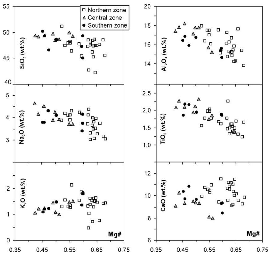
Fig. 4. SiO 2 , Al 2 O 3 , Na 2 O, TiO 2 , K 2 O and CaO (wt.%) versus Mg# variation diagrams for the studied rocks. Symbols as in Fig. 3.
