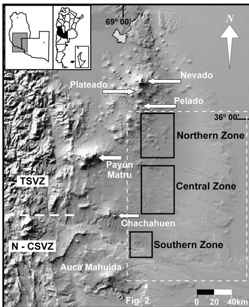
Fig. 1. Satellite image of the border zone between La Pampa, Mendoza and Neuquén provinces, with the studied zones, the Upper Tertiary arc volcanoes Nevado–Plateado–Pelado, Payún Matru and Chachahuen. Also shown is the basaltic volcanic complex Auca Mahuida.
