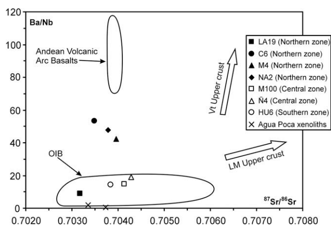
Fig. 7. Ba/Nb versus ^{87}\text{Sr}/^{86}\text{Sr} diagram for seven selected rocks of the Northern Zone (LA19, C6, M4 and NA2), Central Zone (M100 and Ñ4) and Southern Zone (HU6). For comparison are shown Agua Poca xenoliths and fields of Andean volcanic arc basalts (Antuco 37°30'S and Llaima 38°36'S volcanoes, Hickey et al., 1986) and ocean island basalts (OIB, Wilson, 1989). The arrows point to compositions of crustal rocks that form the crystalline basement of the neighboring regions: "Vt" Co La Ventana Fm. type (Cingolani and Varela, 1999), and "LM" Las Matras type (Sato et al., 2000).
