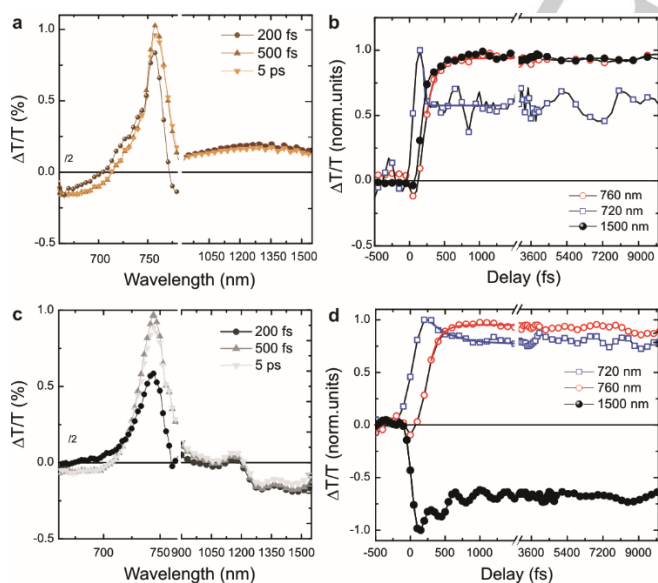
Figure 3. a, c. \Delta T/T evolution from 200 fs to 5 ps upon excitation at 620 nm of the mixed perovskite deposited on non-injecting m\text{-Al}_2\text{O}_3 and on injecting m\text{-TiO}_2 respectively. b, d. Normalized \Delta T/T dynamics at selected probe wavelengths (see legend) for \text{MA}_{(1-y)}\text{FA}_y\text{PbI}_x\text{Br}_{(3-x)} / m\text{-Al}_2\text{O}_3 and m\text{-TiO}_2 , respectively.
