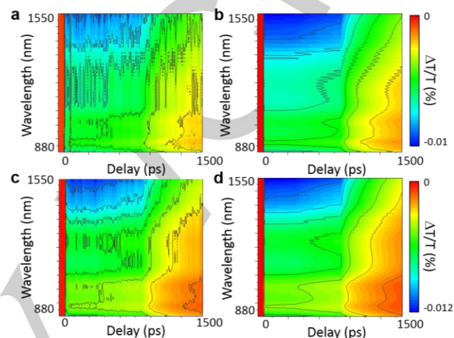
Figure 5. Comparison of the \Delta T/T(\lambda, \tau) maps (a) in the IR probed region and global fitting (b) for the Perovskite/FDT interface. Comparison of the \Delta T/T(\lambda, \tau) maps (c) in the IR probed region and global fitting (d) for the Perovskite/Spiro-OMeTAD interface. Excitation at 620 nm with a fluence of 6 \times 10^{17} photons/cm 3 .
