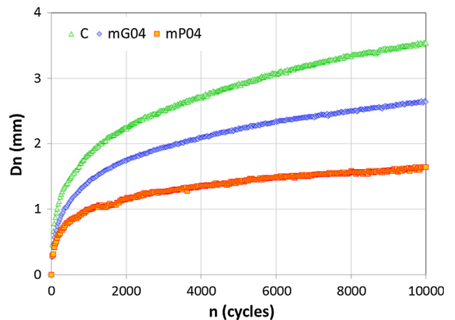
Fig. 6. Permanent deformation versus cycles for FRACs with microfibers.
