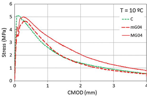
Fig. 11. Comparison of stress – CMOD curves of reference mixture without fibers (C), FRAC with micro glass fiber (mG04) and FRAC with macro glass fiber (MG04).
