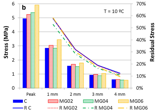
Fig. 13. Peak stress and residual stresses at different CMOD; a: T = 0 °C, b: T = 10 °C.
