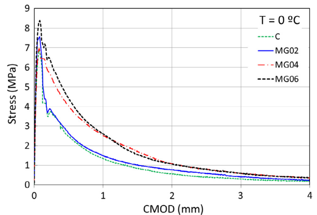
Fig. 9. Fracture test results for some samples of the studied mixtures at 0 °C.
