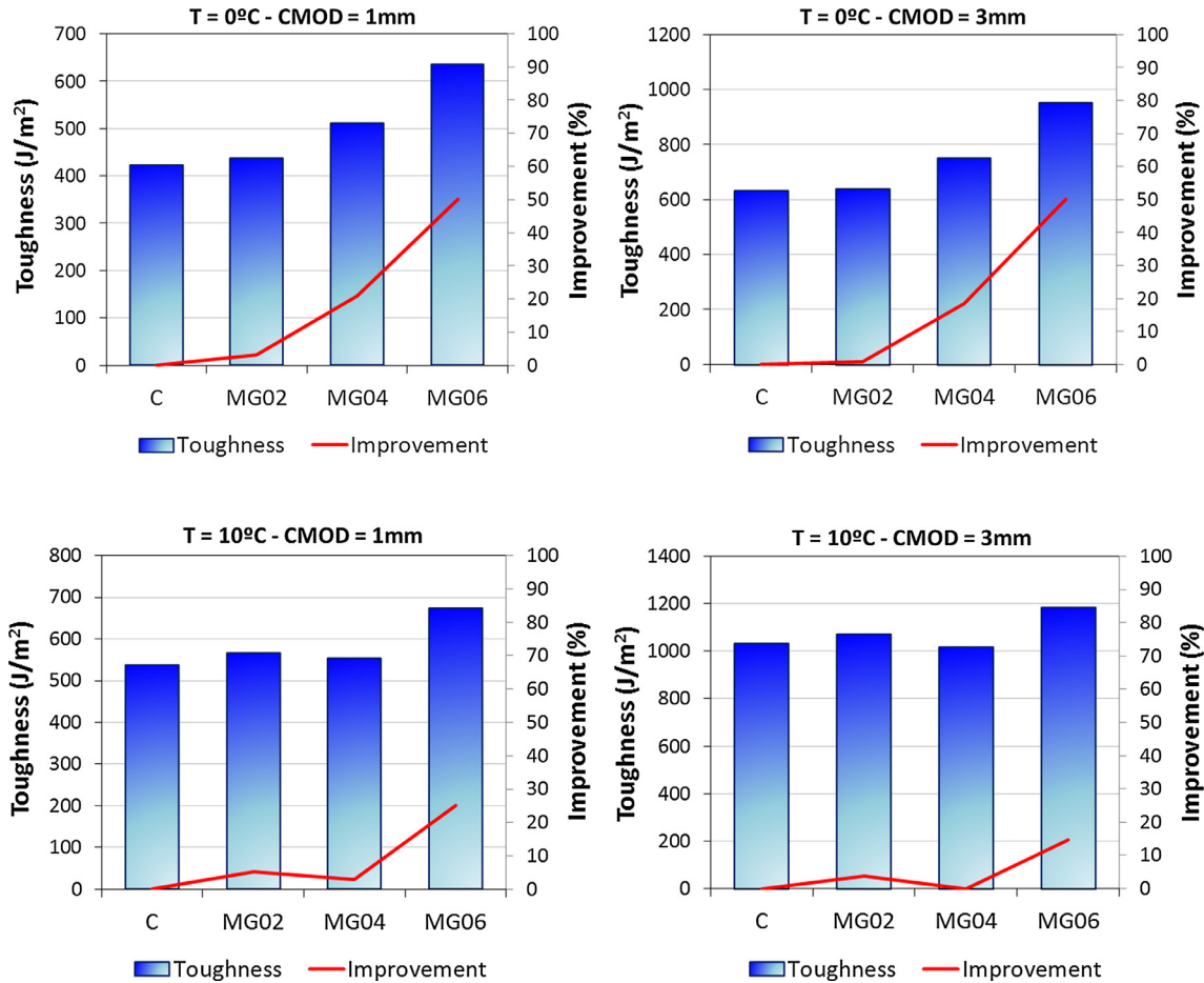
Fig. 14. Comparison of toughness of asphalt concretes obtained from bending tests.
