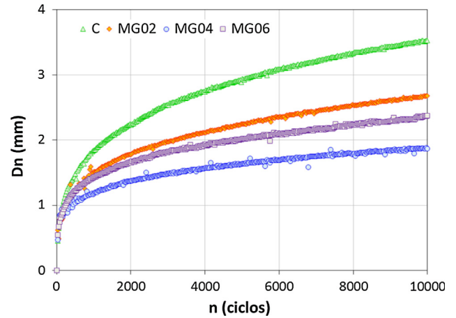
Fig. 8. Permanent deformation versus cycles for FRAC with glass macrofibers.
