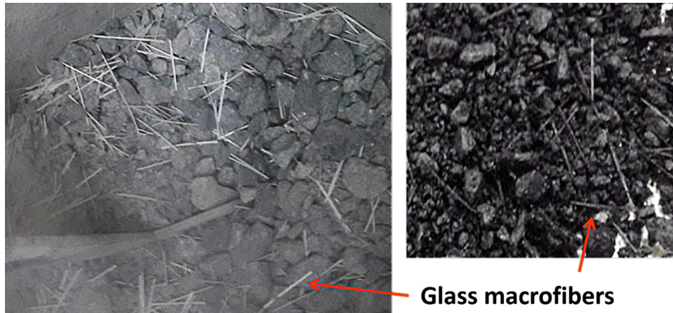
Fig. 2. FRAC mixing. Fiber incorporation and mixture aspect.
