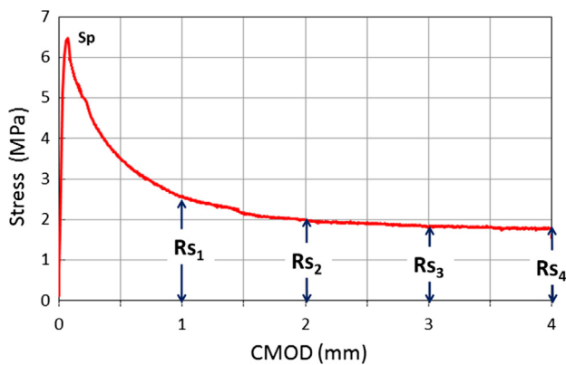
Fig. 5. Typical curve result of bending test.
