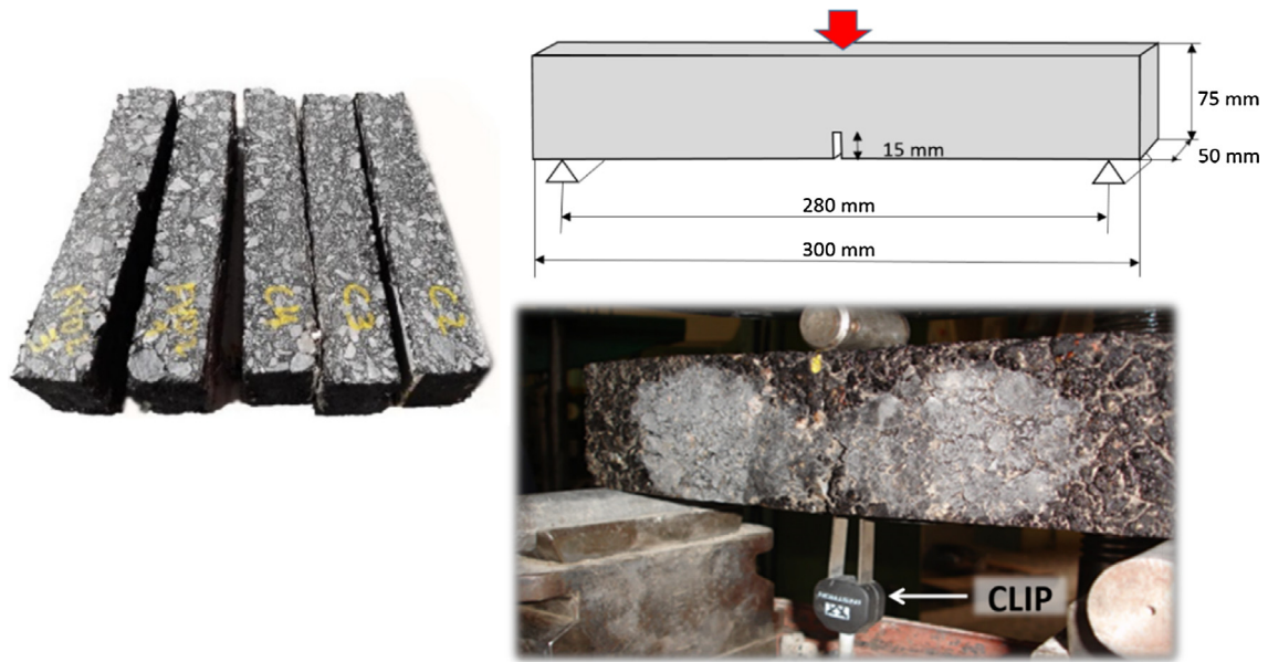
Fig. 4. Bending test of notched beam.
