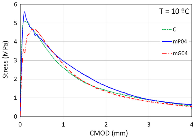
Fig. 7. Stress – CMOD curves of FRAC incorporating microfibers.
