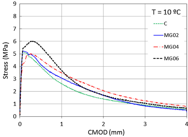
Fig. 10. Fracture test results for some samples of the studied mixtures at 10 °C.
