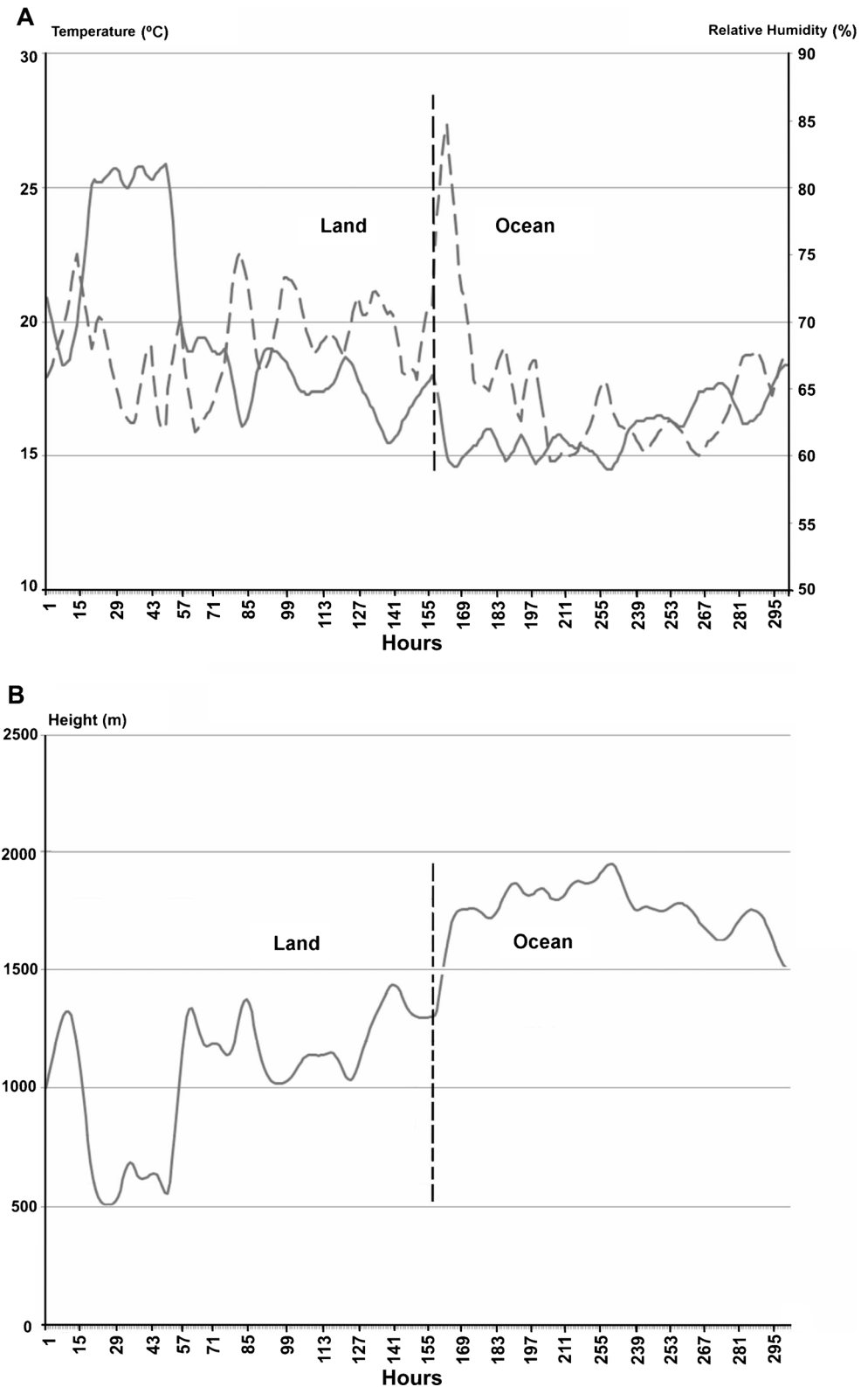
Fig. 5 a Temperature ( T_a in ^{\circ}\text{C} , full line) and relative humidity (RHa in %, dashed line) and b altitude (h in m.a.g.l.) variations in the backward trajectory arriving in Argentina. The vertical line indicates the boundary between land and ocean
