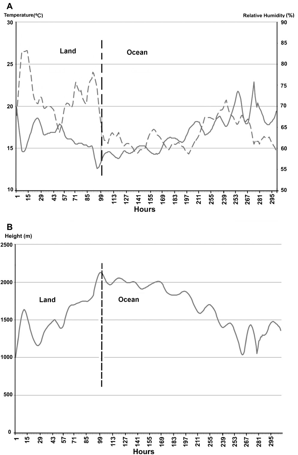
Fig. 6 a Temperature ( T_a in ^{\circ}\text{C} , full line) and relative humidity (RHa in %, dashed line) and b altitude (h in m.a.g.l.) variations in the backward trajectory arriving in Bolivia. The vertical line indicates the boundary between land and ocean
