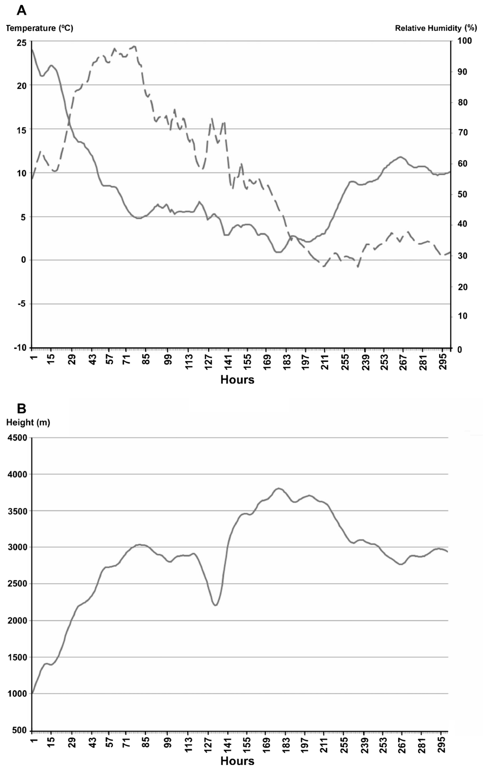
Fig. 9 a Temperature ( T_a in ^{\circ}\text{C} , full line ), and relative humidity (RHa in %, dashed line ) and b altitude (h in m.a.s.l.) variations in the forward trajectory departing from the neotropics during austral summer
