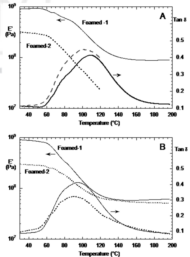
Figure 9 Thermomechanical behavior of reinforced foams with and without added water added, tested 1 year after preparation. (A) Pine wood flour composite; (B) Hemp composite.
