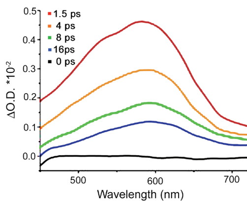
Figure 8. Femtosecond transient absorption spectroscopy of diaminobenzophenone ( 2 ; 150 fs pulse, \lambda_{\text{max}} = 258 \text{ nm} ) as a nanocrystalline suspension. ISC occurs within 5 ps to give the triplet, \lambda_{\text{max}} = 595 \text{ nm} , which decays within 62 ps.
