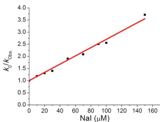
Figure 6. Stern–Volmer plot for the quenching of diacid 6 with NaI as a nanocrystalline suspension. The rate constant of quenching in this case is k_{\text{q}}(\text{I}^-) = 1.4 \times 10^5 \text{ M}^{-1} \text{ s}^{-1} . The values of k_0 and k_{\text{Obs}} correspond to the rate constants in the absence of quencher and in the presence of added quencher, respectively.
