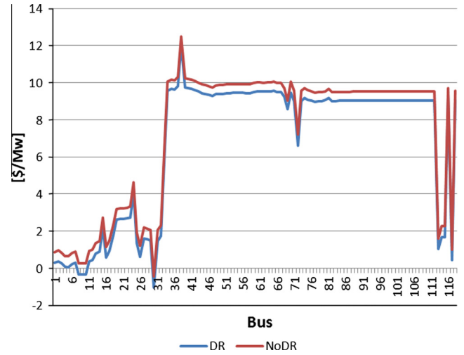
Fig. 5. Bus LMP differences for cases with network congestion at hour 16.
