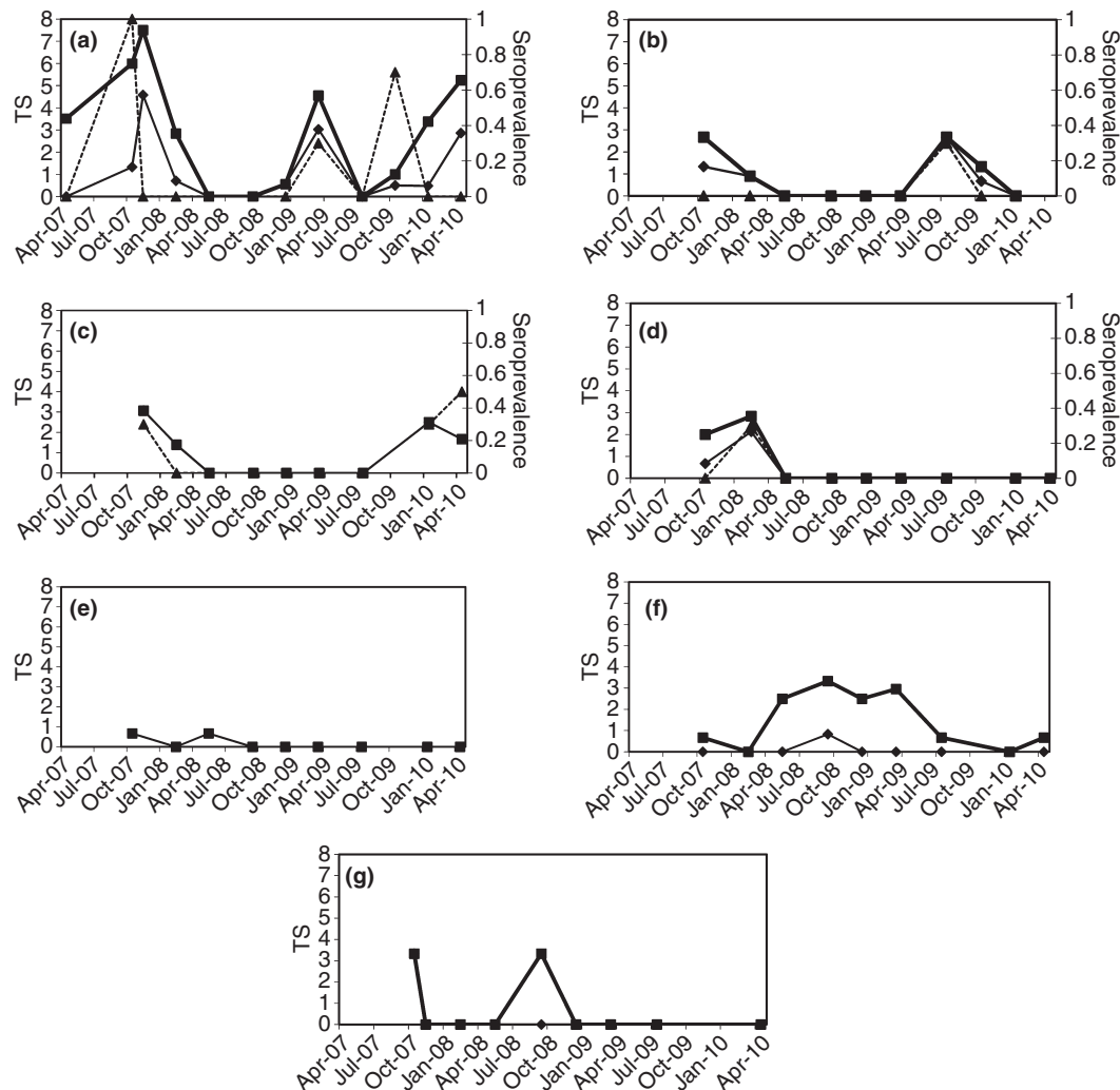
Figure 4 Total trap success (TS) (thick solid line), Oligoryzomys nigripes TS (thin solid line) and seroprevalence (dotted line) in El Palmar National Parks for (a) Camping area; (b) forest dominated by exotic trees; (c) riparian forest 1; (d) palm forest without shrubs; (e) palm forest with shrubs; (f) shrubland; (g) riparian forest 2.
