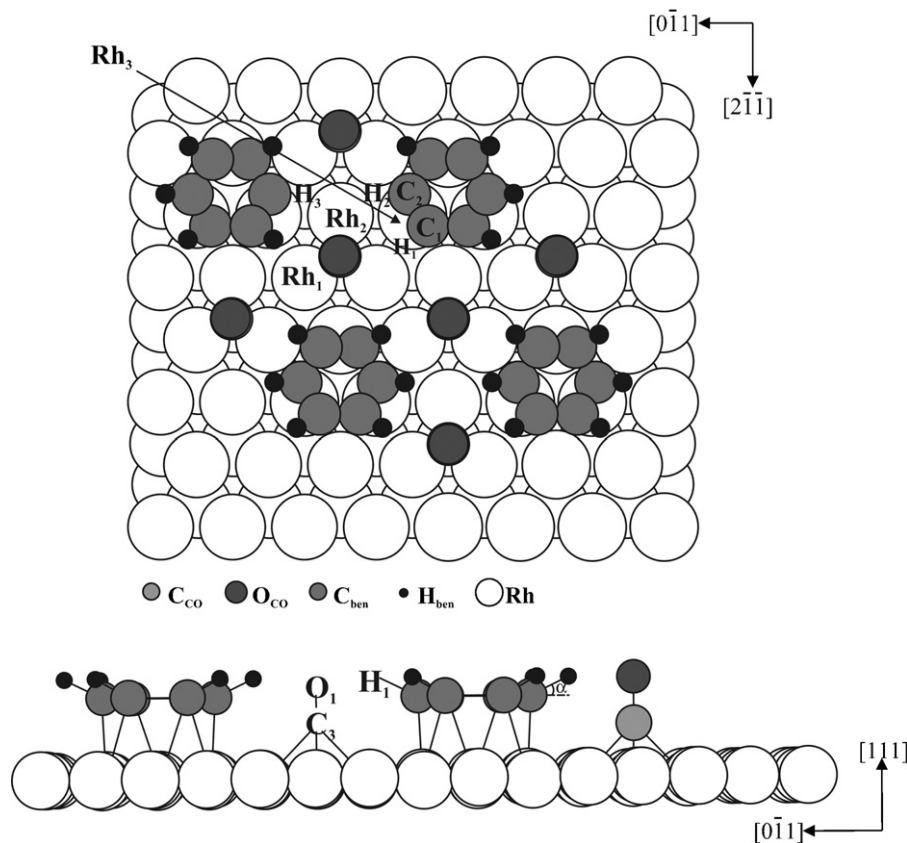
Fig. 1. Schematic top (up) and lateral (down) view of the (\text{C}_6\text{H}_6)_4-(\text{CO})_6/\text{Rh} system.
