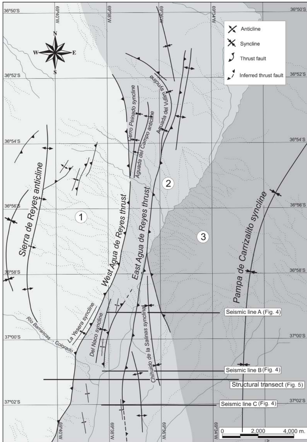
FIG. 3. Main structures described in this work. Note three different zones (1, 2, 3). Zone 1 has a broad discontinuous structure; zone 2 has longer and narrower structures with a shallower décollement; zone 3 is represented by the broad Pampa de Carrizalito syncline. Locations of seismic lines of figure 4 are indicated, as well as structural section depicted in figure 5.
