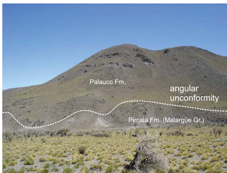
FIG. 6. Angular unconformity between Eocene rocks of the upper Malargüe Group and Late Oligocene to Early Miocene basalts of the Palauco Formation, in the northern part of the study area. This indicates the existence of a Late Eocene uplift in the region (see location in figure 1).
