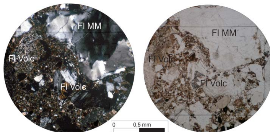
FIG. 10. Thin-sections corresponding to the e unit from Upper Miocene succession in the Pampa de Carrizalito (see figure 9 and figure 7, profile A-A', for location). Note the presence of metamorphic lithic fragments ( FI MM ), represented by polycrystalline quartz.
