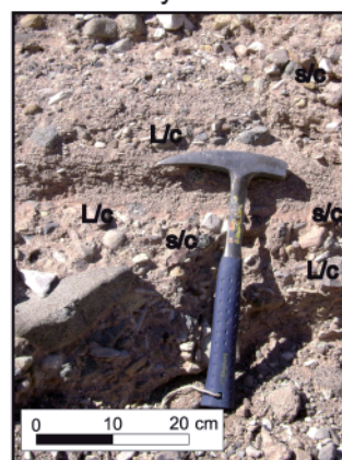
FIG. 11. Outcrop view of c, d y e, f units of Tristeza Formation accumulated in the easternmost Pampa de Carrizalito. See profile B-B' for location. They have the same sources described for the westernmost profile. Note again the appearance of clasts of different compositions resulting from the progressive unroofing of the Sierra de Reyes. V/c : Volcanic Clast; S/c : Sandstone Clast; L/c : Limestone Clast; Sh/c : Shale Clast.
