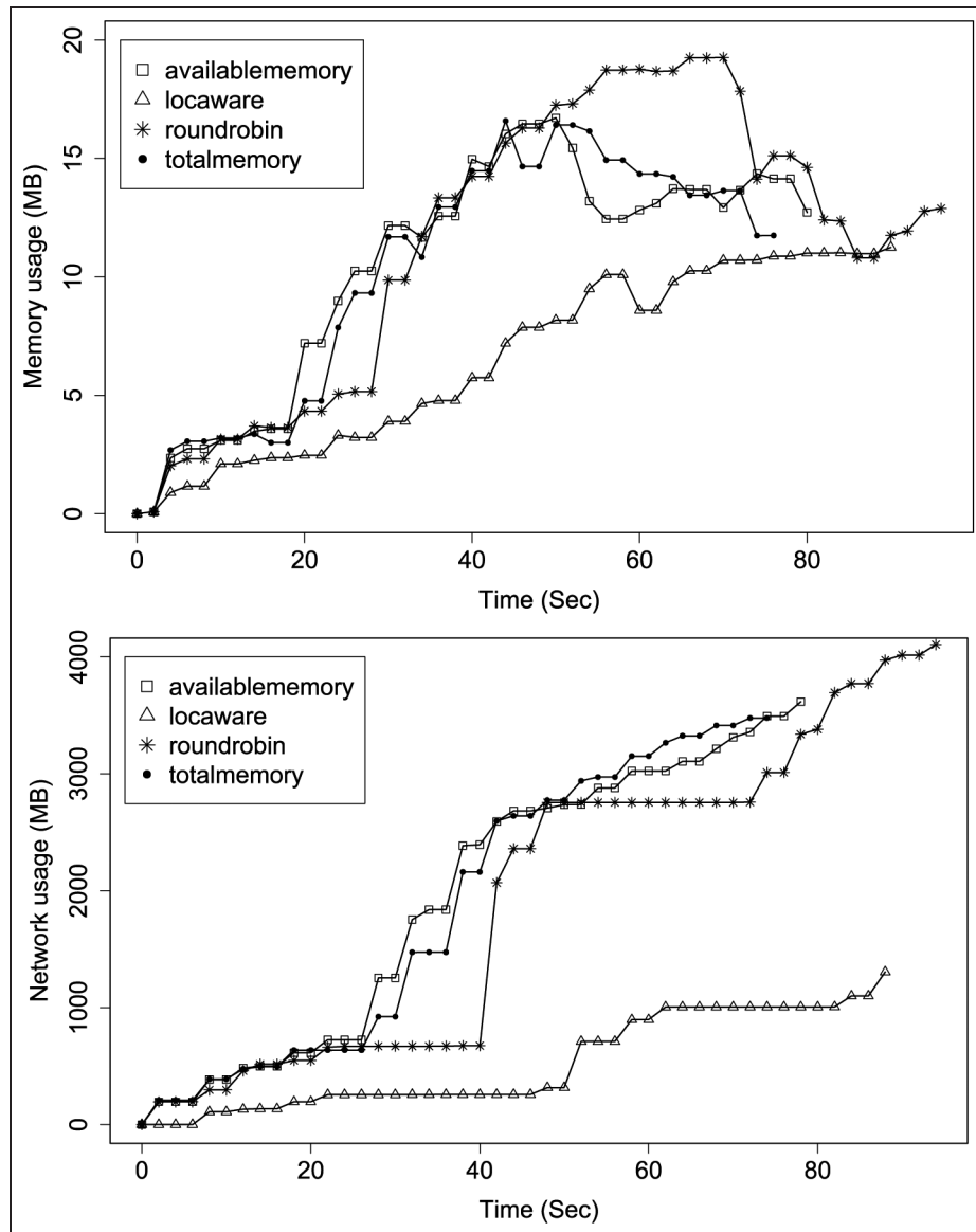
Figure 10. Cluster network and memory usage for an example user.
