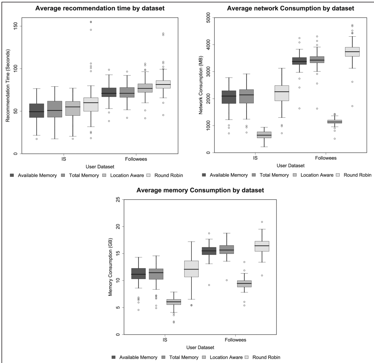
Figure 9. Average results for each testing group of users.
