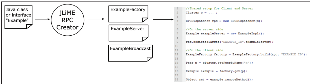
Figure 3. jLiME RPC workflow.
