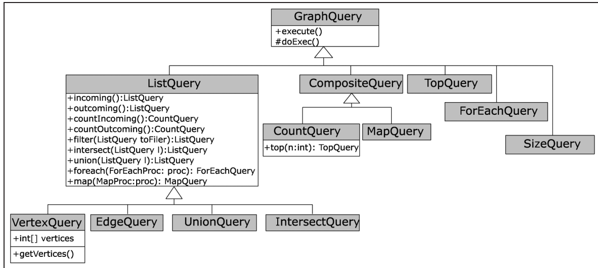
Figure 5. GraphQuery hierarchy.
