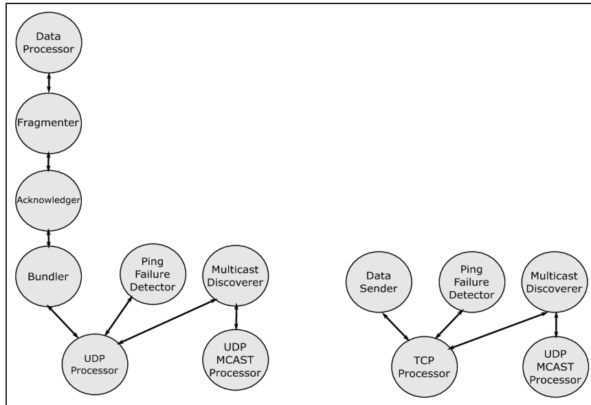
Figure 11. UDP and TCP stacks in jLiME.
