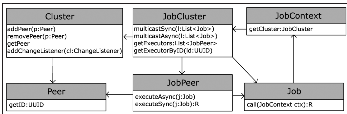
Figure 4. jLiME design: main abstractions.
