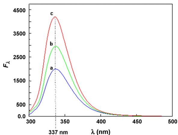
Fig. 4. Fluorescence emission spectra of solutions 2.4 \mu\text{mol L}^{-1} of 5HIA at pH 2.00 and 25.0^\circ\text{C} : (a) buffer solution, (b) with 10 \text{ mmol L}^{-1} of βCD , and (c) with 10 \text{ mmol L}^{-1} of HPCD .
