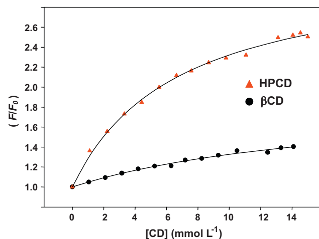
Fig. 5. Relative fluorescence of solutions 2.4 \mu\text{mol L}^{-1} of 5HIA as a function of CD concentrations at pH 6.994 and 25.0^\circ\text{C} : (●) βCD , (▲) HPCD .
