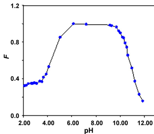
Fig. 3. Profile of fluorescence versus pH for solutions 2.4 \mu\text{mol L}^{-1} of 5HIA at 25.0 \text{ }^\circ\text{C} .
