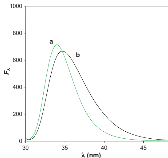
Fig. 2. Fluorescence emission spectra of reference solutions 2.4 \mu\text{mol L}^{-1} at pH 6.994 and 25.0 \text{ }^\circ\text{C} : (a) 5HT and (b) 5HIA .
