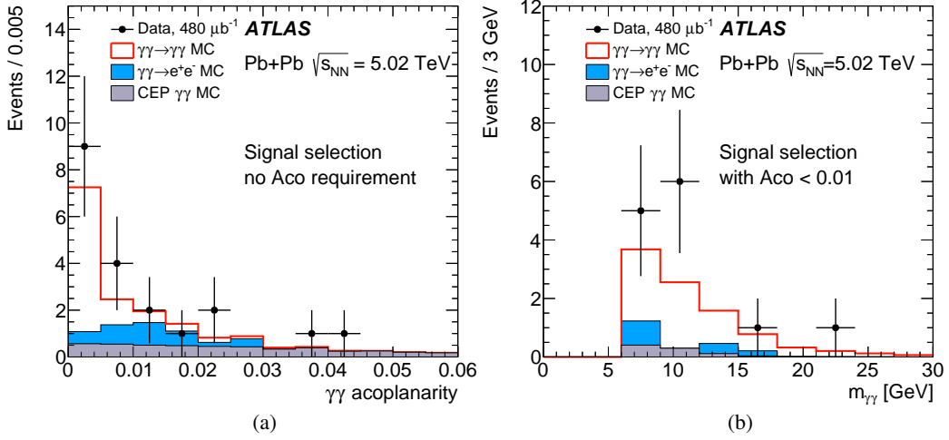
Figure 3: Kinematic distributions for \gamma\gamma \rightarrow \gamma\gamma event candidates. (a) Diphoton acoplanarity before applying \text{Aco} < 0.01 requirement. (b) Diphoton invariant mass after applying \text{Aco} < 0.01 requirement. Data (points) are compared to MC predictions (histograms). The statistical uncertainties on the data are shown as vertical bars.
