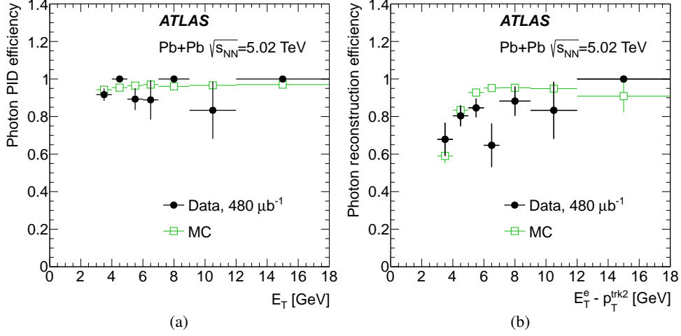
Figure 2: Photon identification and reconstruction efficiencies. (a) Photon PID efficiency as a function of photon E_T extracted from FSR event candidates. (b) Photon reconstruction efficiency as a function of photon E_T (approximated with E_T^e - p_T^{trk2} ) extracted from \gamma\gamma \rightarrow e^+e^- events with a hard-bremsstrahlung photon. Data (closed markers) are compared with MC simulations (open markers). The statistical uncertainties arising from the finite size of the data and simulation samples are indicated by vertical bars.
