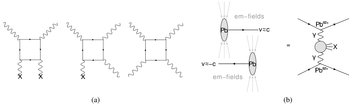
Figure 1: Diagrams illustrating the QED LbyL interaction processes and the equivalent photon approximation. (a) Diagrams for Delbrück scattering (left), photon splitting (middle) and elastic LbyL scattering (right). Each cross denotes external field legs, e.g., an atomic Coulomb field or a strong background magnetic field. (b) Illustration of an ultra-peripheral collision of two lead ions. Electromagnetic interaction between the ions can be described as an exchange of photons that can couple to form a given final-state X. The flux of photons is determined from the Fourier transform of the electromagnetic field of the ion, taking into account the nuclear electromagnetic form factors.
