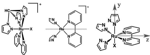
Fig. 1 Left: Sketches of the [\text{Ru}(\text{tpm})(\text{bpy})\text{X}]^+ complexes studied in this work, RubNCS + ( X = \text{NCS}^- ) and RubCN + ( X = \text{CN}^- ). Center: The dotted line indicates the reflection plane that bisects the bpy ligand, determining the C_s symmetry. Right: Axis denomination for RubNCS + and RubCN + . The x axis is normal to the page.
