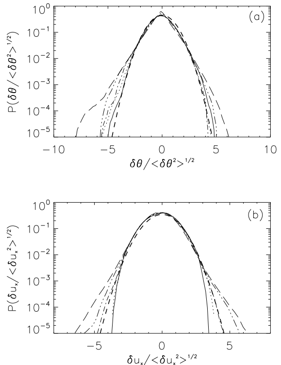
FIG. 7: Probability density functions in run B3, for five different horizontal spatial increments l = 1.6 (solid), 0.8 (dashed), 0.4 (dash-dotted), 0.2 (dash-triple-dotted), and 0.1 (long dashes), and for (a) the passive scalar, and (b) the x -component of the velocity field. A Gaussian curve with unit variance is indicated by the dotted curve. As intervals are decreased, curves depart more and more from the Gaussian distribution developing stronger tails.
