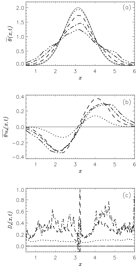
FIG. 9: (a) Averaged horizontal concentration \bar{\theta} in run B1 x (no rotation, helical) at times t = 0 (solid), 0.5 (dotted), 1 (dashed), 1.25 (dash-dotted), and 1.5 (dash-triple-dotted). (b) Horizontal flux at the same times. (c) \mathcal{D}_x(x, t) at the same times.
