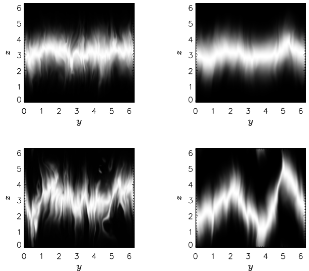
FIG. 17: Passive scalar concentration in a vertical slice of runs A3_z (left) and B3_z (right) at time t = 0.5 (top row), and at time t = 1.5 (bottom row).
