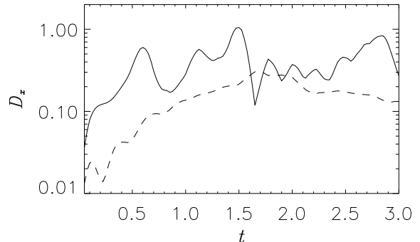
FIG. 13: Horizontal turbulent diffusion as a function of time for runs A3 x (solid) and B3 x (dashed) (Ro = 0.01, respectively without and with helicity).
