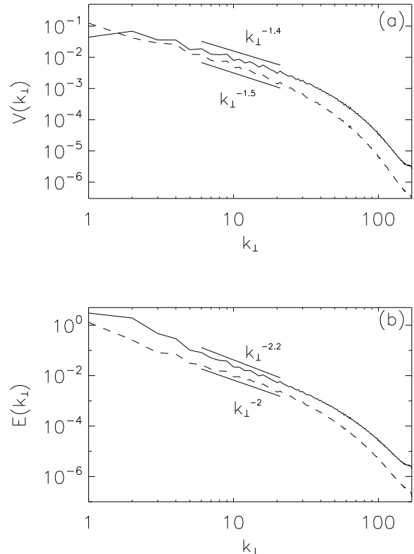
FIG. 1: (a) Reduced perpendicular passive scalar variance spectrum for run B3 (rotating and helical, solid) and for run A3 (rotating and non-helical, dashed). (b) Reduced perpendicular energy spectrum for run B3 (solid) and for run A3 (dashed).
