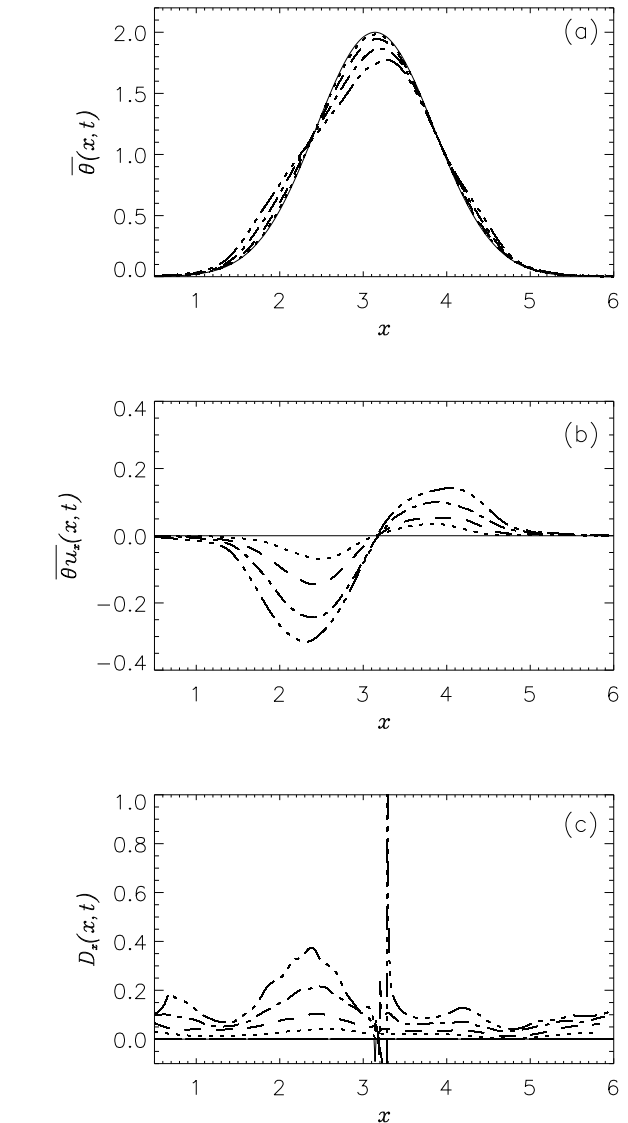
FIG. 11: (a) Averaged horizontal concentration \bar{\theta} in run B3 x , at times t = 0 (solid), 0.25 (dotted), 0.5 (dashed), 0.75 (dash-dotted), and 1 (dash-triple-dotted). (b) Horizontal flux at the same times. (c) \mathcal{D}_x(x, t) at the same times.
