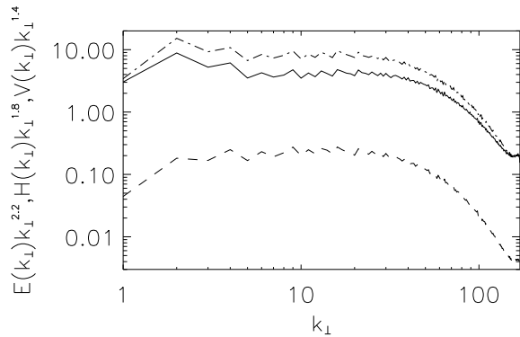
FIG. 2: Reduced perpendicular energy spectrum compensated by k_{\perp}^{-2.2} (solid), reduced perpendicular passive scalar spectrum compensated by k_{\perp}^{-1.4} (dashed), and reduced perpendicular helicity spectrum compensated by k_{\perp}^{-1.8} (dash-dotted) in run B3 (with rotation and helicity).
