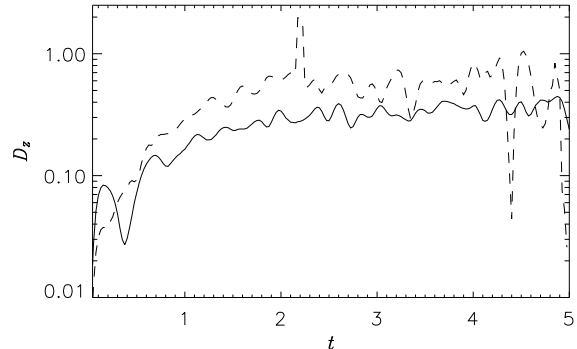
FIG. 15: Vertical turbulent diffusion as a function of time for runs A3_z (solid) and B3_z (dashed). The former run has no net helicity, while the latter has helical forcing.
