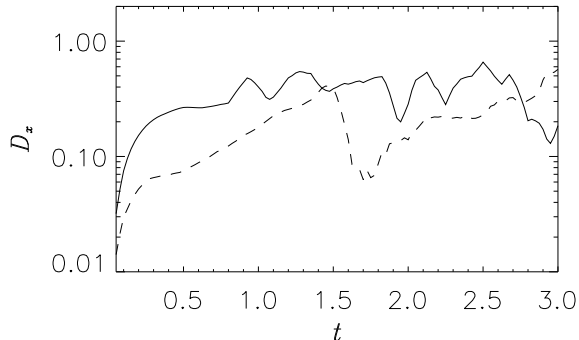
FIG. 12: Horizontal turbulent diffusion as a function of time for runs A2 x (solid) and B2 x (dashed) (Ro = 0.02, respectively without and with helicity).
