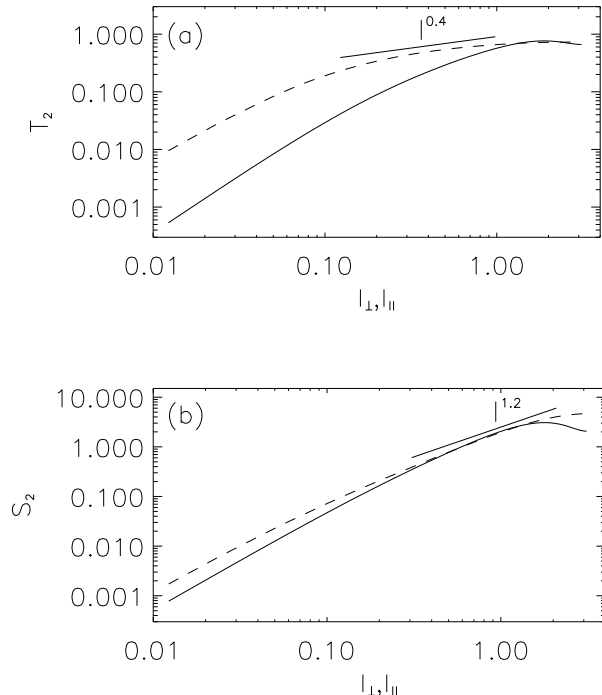
FIG. 4: Axisymmetric second order structure functions for run B3 (helical with rotation) for (a) the passive scalar, and (b) the velocity field. In both panels solid lines correspond to the parallel structure functions, while dashed lines correspond to the perpendicular structure functions. Slopes indicated as references correspond to the time average of the scaling exponents, obtained from a best fit in the inertial range of the structure functions at different times.
