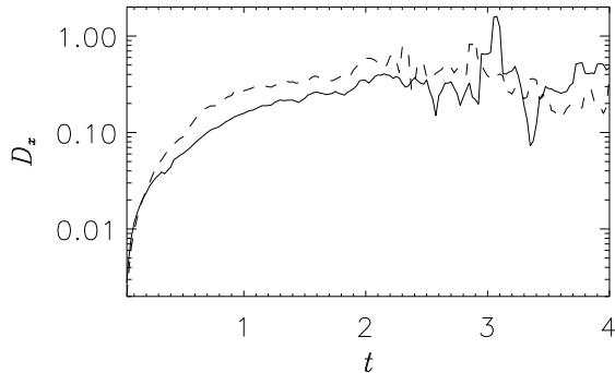
FIG. 10: Horizontal turbulent diffusion as a function of time for runs A1 x (solid, no rotation and no helicity) and B1 x (dashed, no rotation but with helical forcing).
