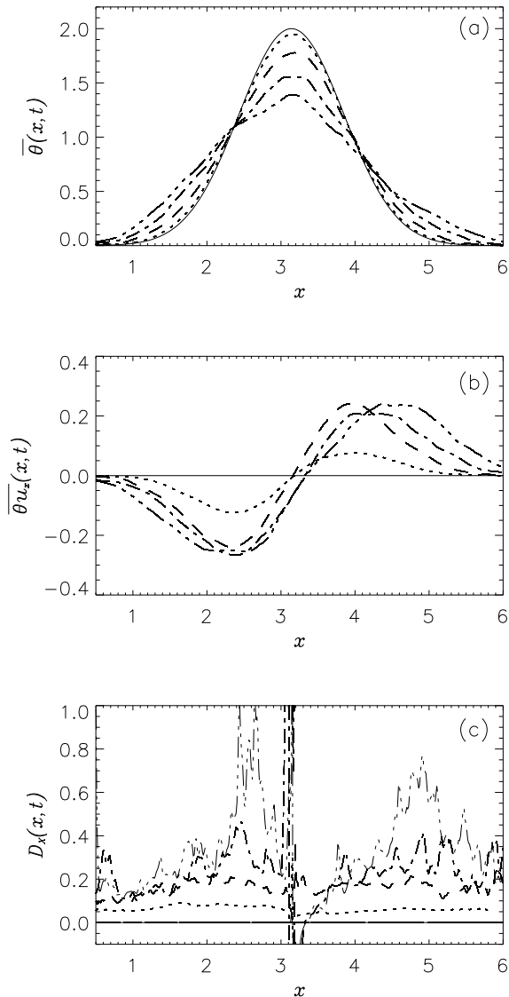
FIG. 8: (a) Averaged horizontal concentration \bar{\theta} in run A1 x (no rotation, no helicity) at times t = 0 (solid), 0.5 (dotted), 1 (dashed), 1.25 (dash-dotted), and 1.5 (dash-triple-dotted). (b) Horizontal flux at the same times. (c) \mathcal{D}_x(x, t) at the same times.
