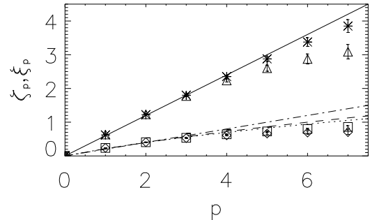
FIG. 5: Scaling exponents (with error bars) as a function of the order p in simulations of helical rotating turbulence, for the velocity field (triangles for run B2 and stars for run B3, both with helicity and with decreasing Rossby number), and for the passive scalar (diamonds for run B2 and squares for run B3). The solid line corresponds to the linear scaling expected for the velocity field exponents in the absence of intermittency, while the dash-dotted line corresponds to non-intermittent scaling for the passive scalar exponents. The dotted and dashed lines correspond to Kraichnan's model with \zeta_2 = 0.4 and respectively with d = 2 and with d = 3 .
