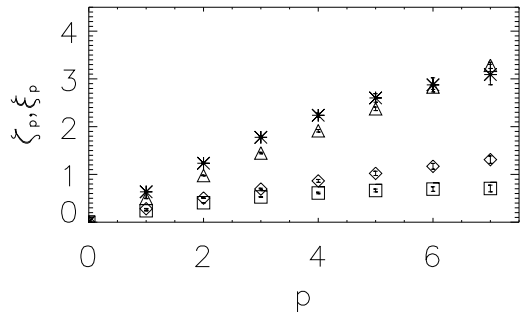
FIG. 6: Scaling exponents (with error bars) as a function of the order p in simulations of rotating turbulence with and without helicity, for the velocity (triangles for run A3 without helicity, and stars for run B3 with helicity), and for the passive scalar (diamonds for run A3, and squares for run B3).
