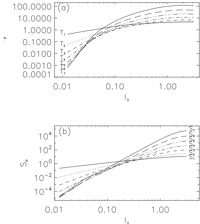
FIG. 3: Averaged axisymmetric structure functions (only for l_{\perp} increments) up to seventh order in run B3 (rotating and helical) for (a) the passive scalar, and (b) the velocity field.
