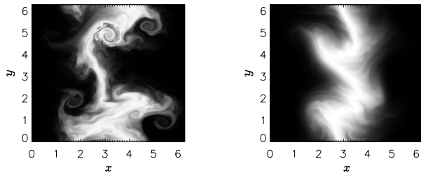
FIG. 16: Passive scalar concentration in a horizontal slice of runs A3_x (left) and B3_x (right) at time t = 1 . Note how the initial concentration (Gaussian, centered around x = \pi , and independent of the y -coordinate) gets distorted and diffused.
