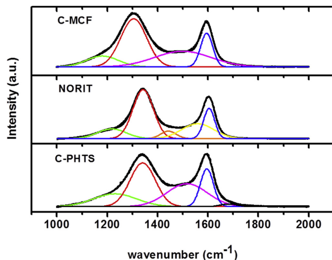
Fig. 5. RAMAN spectra (fitting included to four or five components) of the carbons studied in this work.
