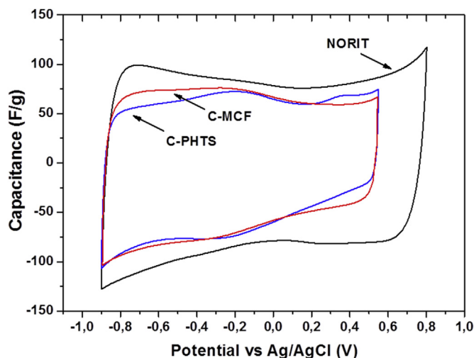
Fig. 7. First voltammetric cycle of the carbons studied in this work in 0.5 M K_2SO_4(aq) . Voltage steps = 20 mV s^{-1} . Counter electrode: Pt. Reference electrode: Ag/AgCl.
