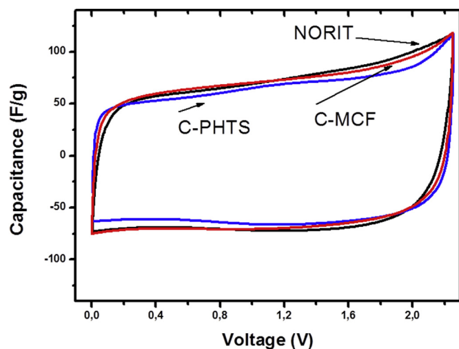
Fig. 13. Fifth voltammetric cycle of the symmetric capacitors based on carbons (NORIT, C-MCF, C-PHTS) in 1.5 M NET4BF4 ( CH3CN ). Voltage steps = 20 mV s -1 .
