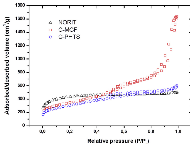
Fig. 3. Nitrogen adsorption/desorption isotherms for the template mesoporous carbons prepared in this work and NORIT carbon.
