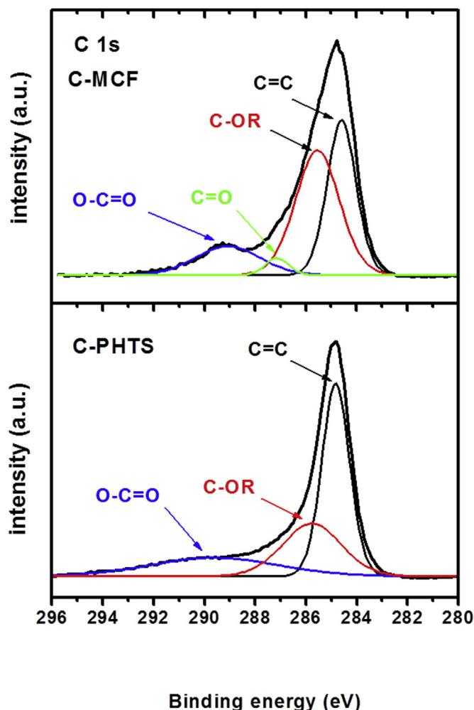
Fig. 6. XPS spectra (fitting included to three or four components) of the TMCs studied in this work.
