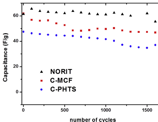
Fig. 11. Capacitance versus number of galvanostatic cycle ( 1 = 0.5 \text{ A g}^{-1} ) of the symmetric capacitors with NORIT and TMC-based electrodes.
