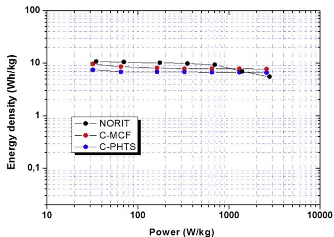
Fig. 12. Ragone plots for the symmetric capacitors with NORIT and TMC-based electrodes.
