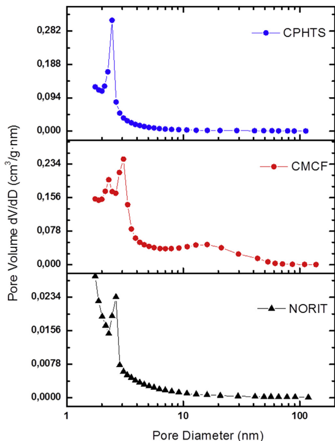
Fig. 4. Pores distribution in the TMC and NORIT materials, calculated from the desorption branch by using the BJH method.
