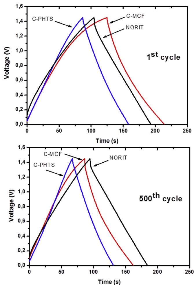
Fig. 9. First and 500th galvanostatic cycle ( I = 0.5\text{ A g}^{-1} ) of the symmetric capacitor based on NORIT and TMC-based electrodes.
