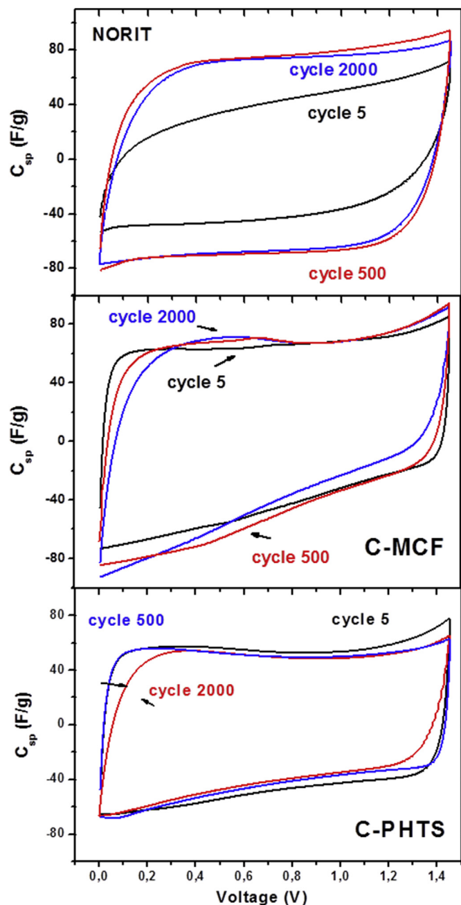
Fig. 10. Cyclic voltammograms corresponding to symmetric capacitors based on carbon electrodes after 5, 500 and 2000 cycles under 0.5 \text{ A g}^{-1} .
