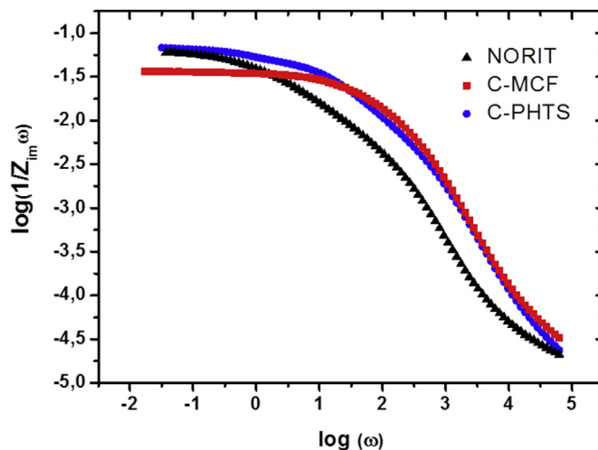
Fig. 8. Bode diagram for the TMCs and NORIT studied in this work.
