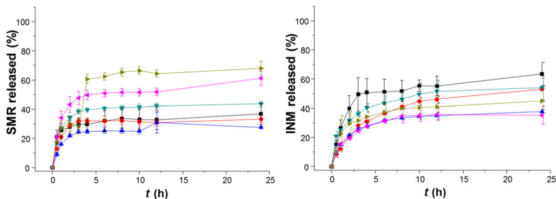
Figure 5. In vitro release profiles from a cellulose acetate membrane of (a) SMR and (b) INM from PBS pH 7,4 (■); ME 1 (●); ME 2 (▲); ME 3 (▼); ME 4 (◆); or ME 5 (▷) (each value represents the average \pm SD of n \geq 3 ).
