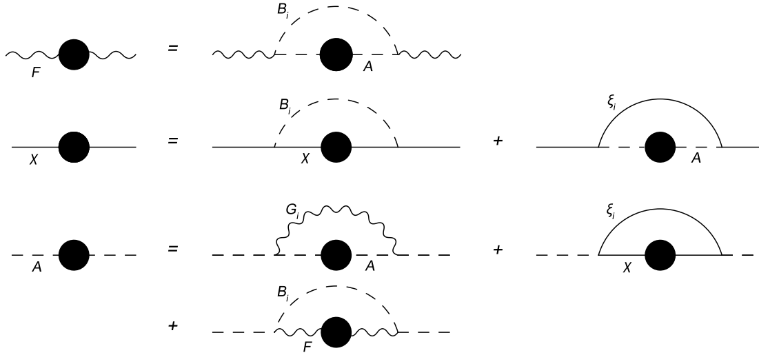
Figure 1: Schwinger-Dyson equations
