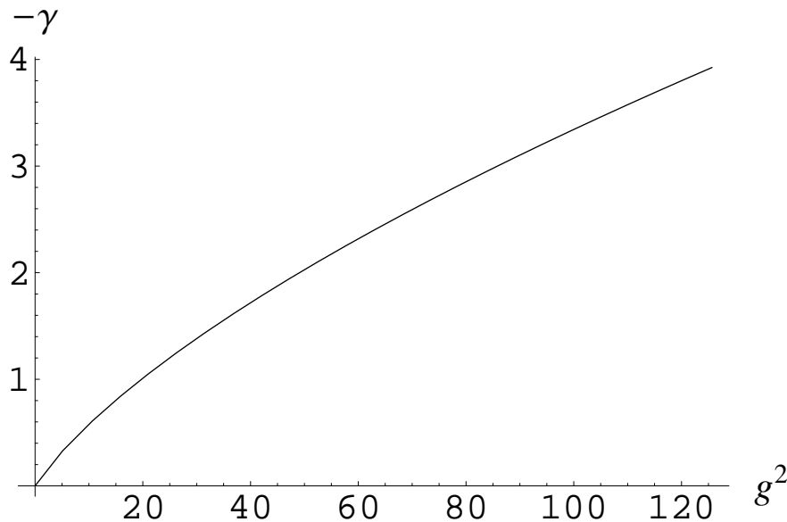
Figure 2: Anomalous dimension as a function of g^2
