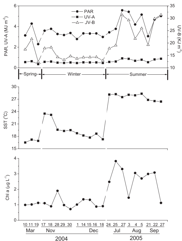
Figure 4. The solar dose (PAR, UV-A and UV-B) during incubation periods (1030–1330 h) (A), and surface seawater temperature (SST) (B) and Chl a concentrations (C) during the experimental period.
