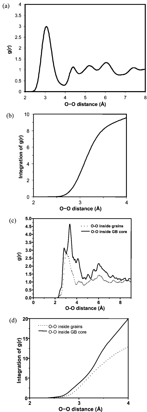
Figure 13. Radial O–O distribution function g(r) and its integration for 12.5% Y-doped \text{BaZrO}_3 without grain boundaries (a, b) and with grain boundaries (c, d).
