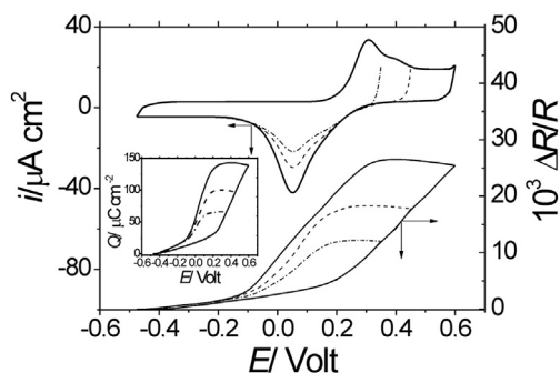
Fig. 1. Voltammetric ( I - E ) and relative surface resistance ( \Delta R/R - E ) responses of a 30 nm gold film electrode in contact with a 0.2 M Na(OH) solution. Inset: Charge vs. potential ( Q - E ) dependence for the same gold film electrode obtained by integration of the I - E response. Potential scan rate: 0.010 \text{ V s}^{-1} .
