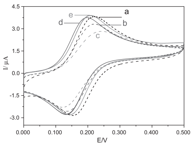
Fig. 2. Cyclic voltammograms obtained at 0.100 \text{ Vs}^{-1} on: (a) Au (---), (b) Au/MPS (— — —), (c) Au/MPS/QCHI (— · — · —), and Au/MPS/(QCHI-NP) with (d) 60 (—), (e) 120 min (—) of NP adsorption time. Experimental conditions: 5.0 \times 10^{-4} \text{ mol dm}^{-3} FcOH solution. Supporting electrolyte 0.500 \text{ mol dm}^{-3} NaClO 4 . Potential vs. (Ag/AgCl/3 M NaCl)/V.
