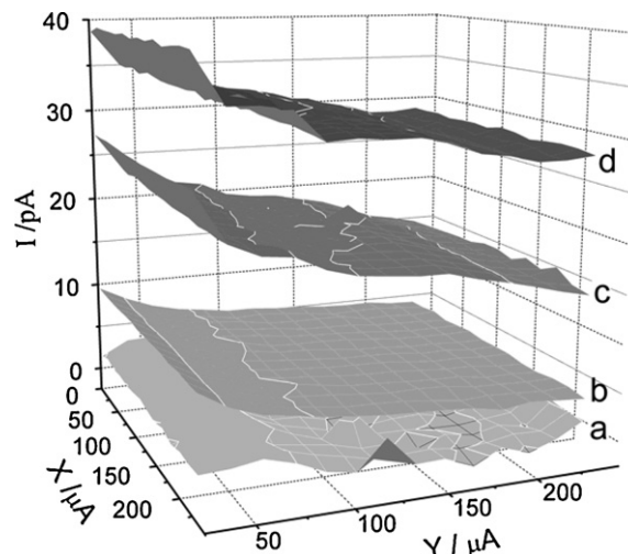
Fig. 5. Surface-plot images obtained in SG-TC mode at Au/MPS/(QCHI-GOD) 1 (plot a and c), and Au/MPS/(QCHI-NP) 1 /(QCHI-GOD) 1 (plot b and d), electrodes. Images c and d were obtained in 0.050 mol dm -3 glucose solution while images a and b were acquired in phosphate buffer pH 7.40. Experimental conditions: E_T = 0.700 V vs. (Ag/AgCl/3 M NaCl) and E_s at o.c.p. Image parameters: 250 \mu\text{m} \times 250 \mu\text{m} , 20 \mu\text{m s}^{-1} UME scan rate.
