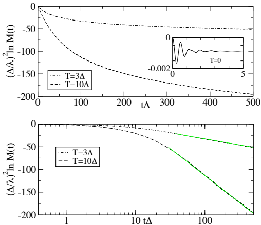
FIG. 15: (Color online) (\Delta/\lambda)^2 \ln M(t) as a function of time for h = 2h_c . For low T , since \Gamma_2(E) is gapped, the decoherence is very weak and shows oscillations (inset). As T increases, the coherence decays asymptotically as a power law.
