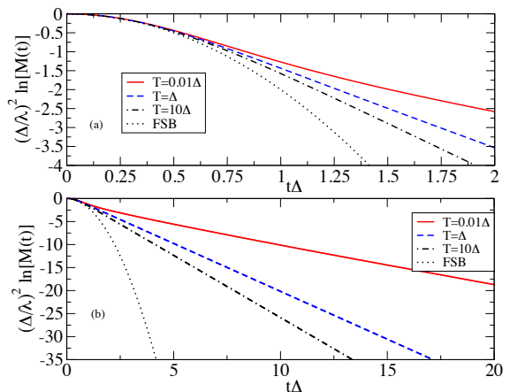
FIG. 6: (Color online) (\Delta/\lambda)^2 \ln M(t) for the SK bath and the comparison with the free spin-bath (FSB); (a) for short times, where it can be seen that at T = \Delta , there's a change of the curvature in \ln M(t) ; (b) for long times.
