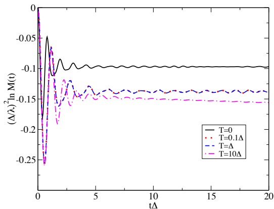
FIG. 18: (Color online) \Delta\lambda^2 \ln M(t) for N=9 and field h=2h_c for different T . For T=0 , since \Gamma_2(E) is gapped, the decoherence is partial but asymptotic Markovian decoherence is recovered at finite T .
