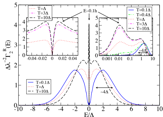
FIG. 9: (Color online) \Delta\lambda^{-2}\Gamma_2^R(E) for different T , with N = 9 and magnetic field set to h = 0.1h_c . Note the completely different behavior from the case h = 0 (Fig. 5, at small T , \Gamma_2(E) is gapped (right inset, \Gamma_2(E) in a logarithmical scale). For higher T (left inset), \Gamma_2(E) is linear at low energies. We note that the T = 0 curve is indistinguishable from the one at T = 0.1\Delta .
