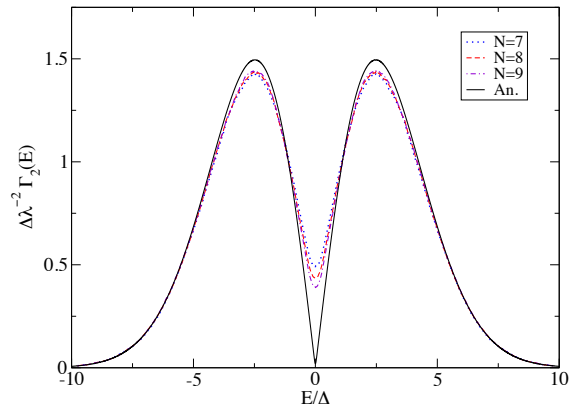
FIG. 1: (Color online) \Delta\lambda^{-2}\Gamma_2(E) as a function of E for T = 0.01\Delta and different N . Note that as N increases, the numerical results approach the analytical result (An.). A similar result is found for the SK long range system.
