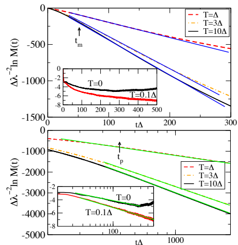
FIG. 11: (Color online) (\Delta/\lambda)^2 \ln M(t) with h = 0.1h_c . The upper graph (linear scale), shows an intermediate time Markovian regime ( t > t \simeq t_m ), while the lower graph (logarithmic scale) shows a final power law regime t > t \simeq t_p ). Insets: \ln M(t) for low T .
