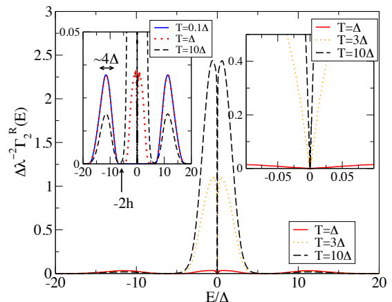
FIG. 10: (Color online) \Delta\lambda^{-2}\Gamma_2^R(E) for different T , with fixed N = 9 and field h = 2h_c (the T = 0 curve is not plotted here since is indistinguishable from that of T = 0.1\Delta ). Right inset: behavior for low E . Left inset: high frequency peaks. The missing spectral weight is carried by the \delta(E) term described in the text.
