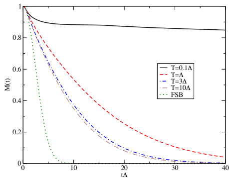
FIG. 13: (Color online) Coherence of the central spin as a function of time, for a bath of N = 10 spins for h = 0.1h_c and a bath-qubit coupling \lambda = 0.2\Delta . The free spin case (FSB) is also plotted for reference.
