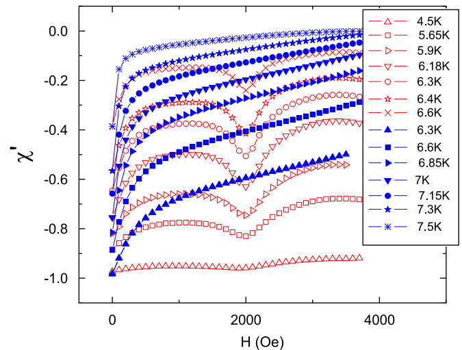
Fig. 3. \chi_{ac}(H) (ZFC) for both samples at different temperatures, Nb (full) and Nb_p sample (open symbols). Nb_p sample shows matching effects for H_1 = 2000 \text{ Oe} .
