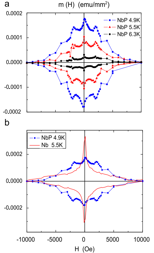
Fig. 5. (a) M(H) at different temperatures for the porous sample where matching effects are observed for H_1 = N * 2000 Oe. (b) M(H) at t = 0.67 for Nb_p and Nb films.
