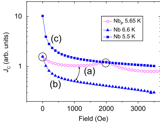
Fig. 4. J_C(H, T) calculated for a circular disk in critical state in a transverse magnetic field from \chi_{ac}(H, T) data, both for the continuous (full) and the porous (open symbols) films. (See text.)
