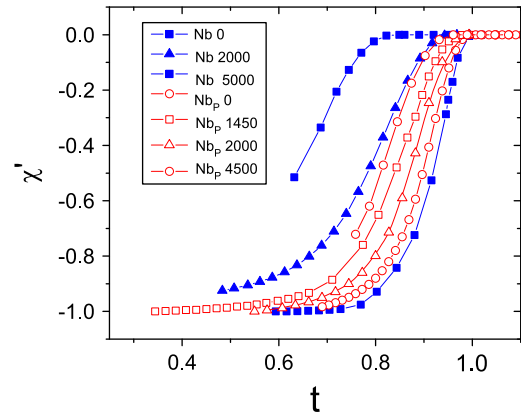
Fig. 2. \chi_{ac}(T) for the continuous Nb film, Nb (full symbols), and for the porous Nb film, Nb_p (open symbols), as a function of reduced temperature t = T/T_{C0} , for different values of applied H .
