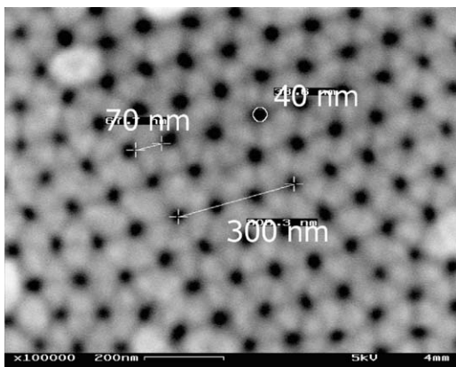
Fig. 1. SEM image of the 100 nm thick porous Nb film. Distance between pores D = 100 \text{ nm} , pore diameter d = 40 \text{ nm} , width of superconducting stripe between pores is \sim 60 \text{ nm} .
