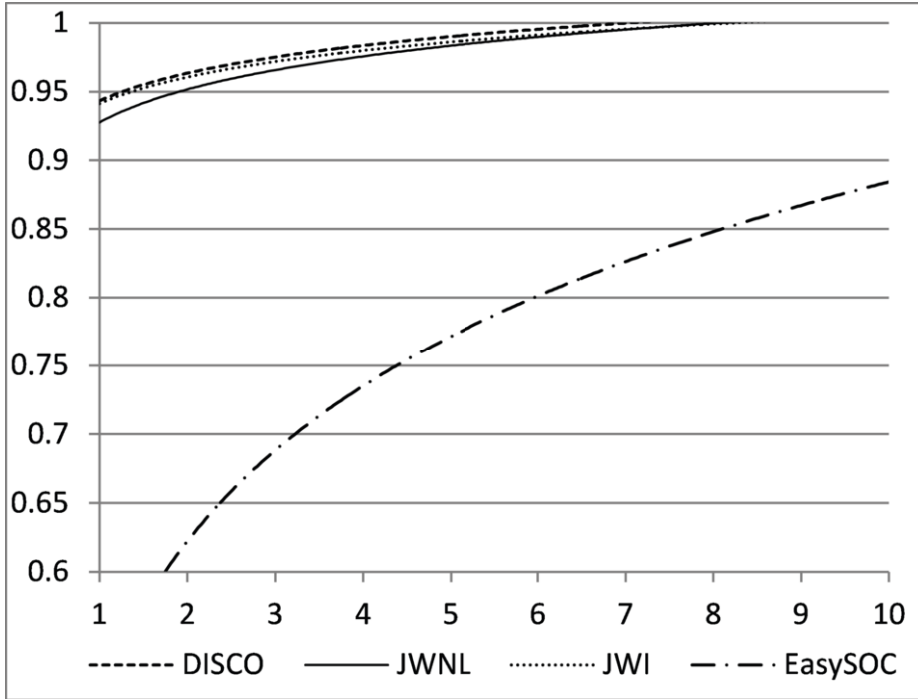
(a) Precision-at-n
