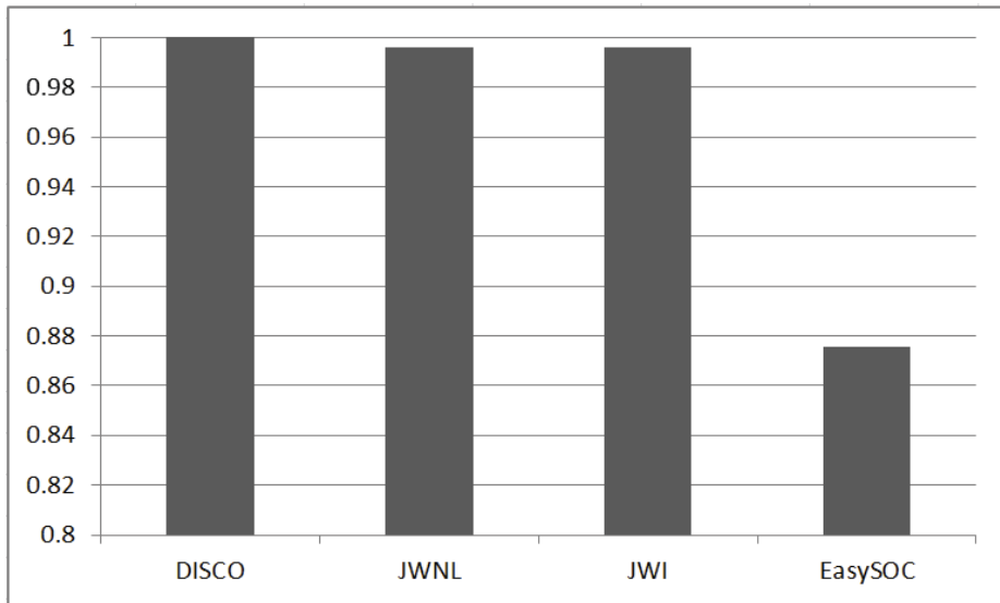
(b) Recall
