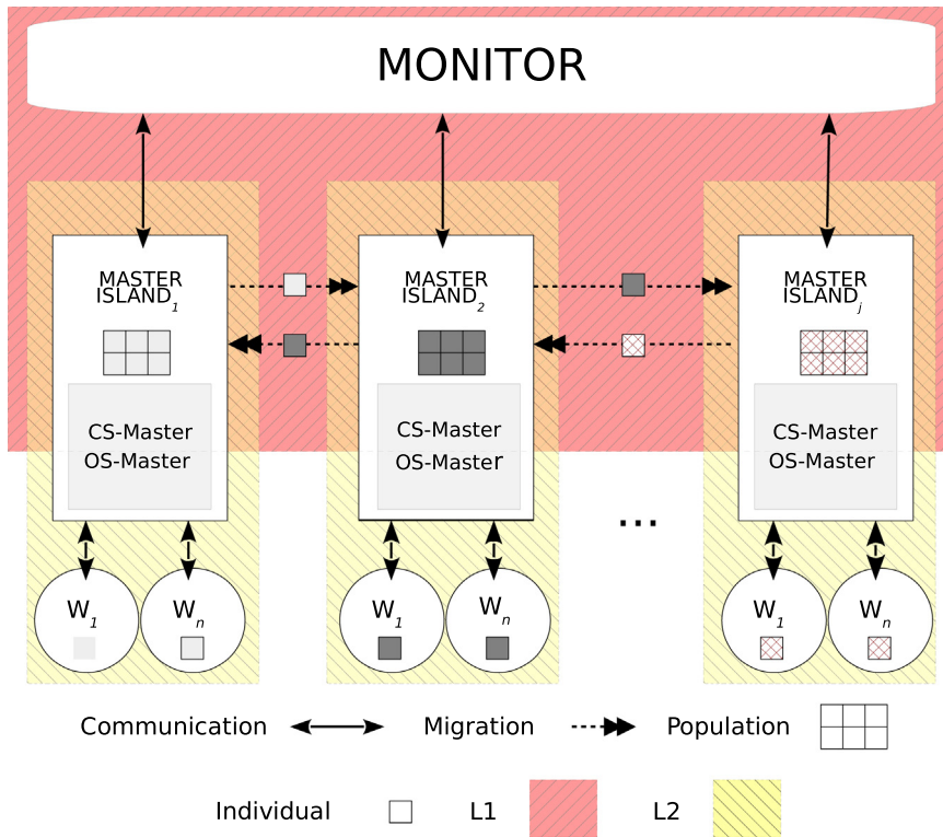
Fig. 8. ESS-IM communication model and population treatment representation. CS-Master : Master Calibration Stage, OS-Master : Master Optimization Stage.
