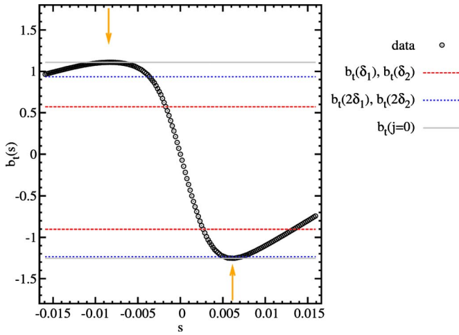
FIG. 20. (Color online) Tangential magnetic field upstream of a particular X-point (black open circles) with different estimates for the upstream magnetic field (horizontal lines): b_{up} evaluated using Eq. (22) (red dashed-lines), Eq. (23) (blue dotted-lines), and Eq. (24) (gray full-lines). The arrows indicate the points in which j(s)=0 .
