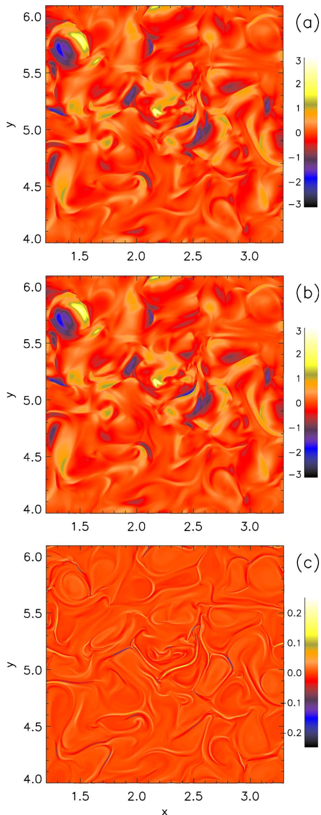
FIG. 5. (Color online) Contour plot of the out-of plane electric field contributions: (a) total electric field E_z , (b) advective term -(\mathbf{v} \times \mathbf{b})_z , and (c) diffusive term R_\mu^{-1} j term.
