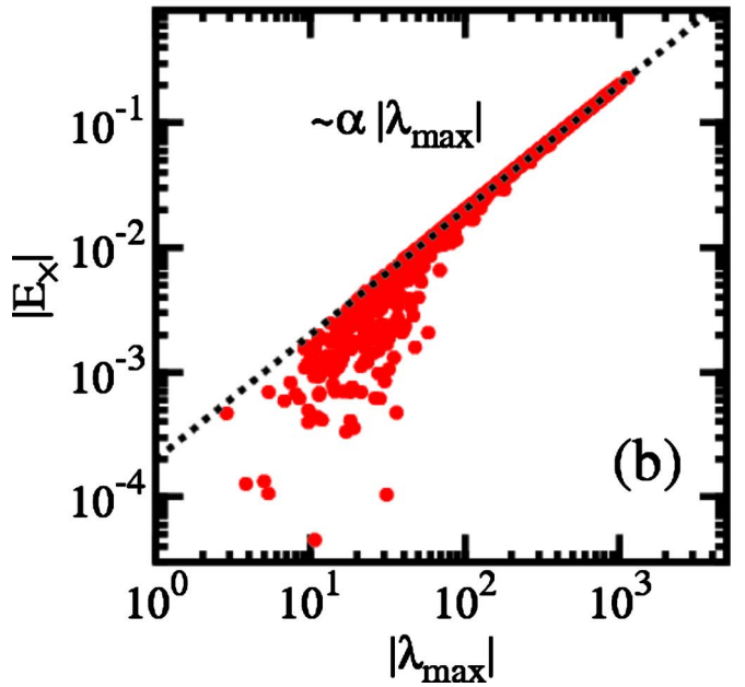
FIG. 9. (Color online) Panel (a): scatter plot of the bigger eigenvalue \lambda_{\max} vs the ratio of eigenvalues \lambda_R . In panel (b) a numerical test that verify Eqs. (9) and (12) is shown. The slope \alpha of the fit (black dotted) is very close to the value of the resistivity R_{\mu}^{-1} .
