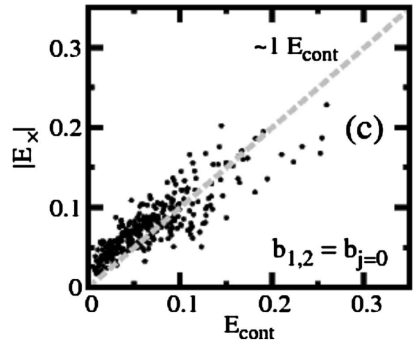
FIG. 21. Scatter plots of the electric field E_\times (in the fast reconnecting sites) vs the steady state function E_{cont} (in absolute value) defined in Eq. (21). We computed E_{cont} by using three different estimations of b_{1,2} , namely, by using Eq. (22) (a), Eq. (23) (b), and Eq. (24) (c).
