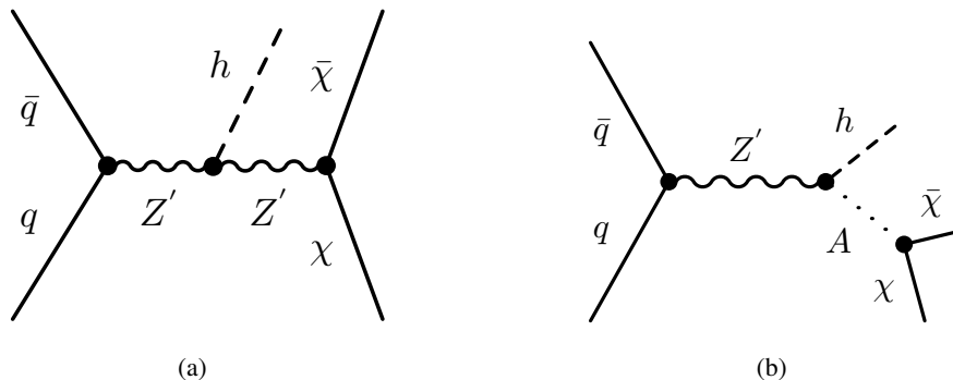
Figure 1: Diagrams showing the simplified models where (a) a Z' decays to a pair of DM candidates \chi\bar{\chi} after emitting a Higgs boson h , and where (b) a Z' decays to a Higgs boson h and the pseudoscalar A of a two-Higgs-doublet model, and the latter decays to a pair of DM candidates \chi\bar{\chi} .
