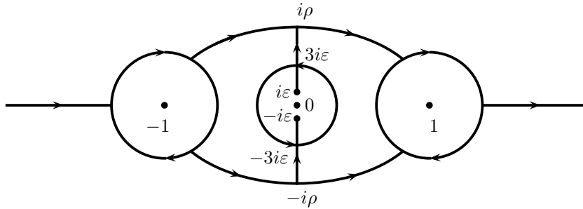
Figure 5: Contour \Sigma_R
