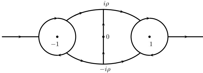
Figure 4: Contour \Sigma_Q
