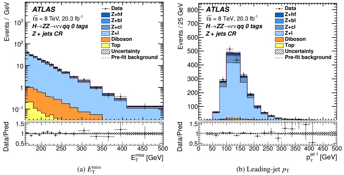
Figure 10: The distributions of (a) missing transverse momentum E_T^{\text{miss}} and (b) leading-jet p_T from the untagged ( Z \rightarrow \mu\mu ) + jets control sample of the H \rightarrow ZZ \rightarrow \nu\bar{\nu}q\bar{q} search. The dashed line shows the total background used as input to the fit. The contribution labelled as ‘Top’ includes both the t\bar{t} and single-top processes. The bottom panes show the ratio of the observed data to the predicted background.
