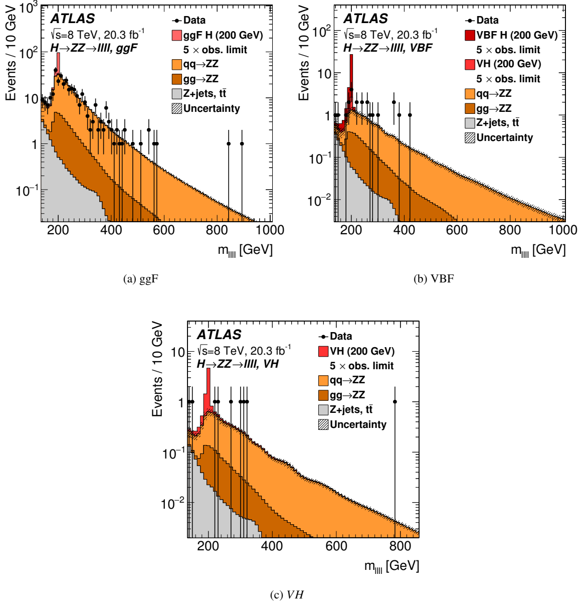
Figure 1: The distributions used in the likelihood fit of the four-lepton invariant mass m_{\ell\ell\ell\ell} for the H \rightarrow ZZ \rightarrow \ell^+\ell^-\ell^+\ell^- search in the (a) ggF, (b) VBF, and (c) VH channels. The ‘Z+jets, t\bar{t} ’ entry includes all backgrounds other than ZZ, as measured from data. No events are observed beyond the upper limit of the plots. The simulated m_H = 200 GeV signal is normalized to a cross-section corresponding to five times the observed limit given in Section 11. Both the VBF and VH signal modes are shown in (b) as there is significant contamination of VH events in the VBF category.
