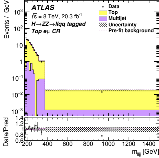
Figure 8: The distribution of m_{\ell\ell jj} in the e\mu top-quark control region of the H \rightarrow ZZ \rightarrow \ell^+\ell^-q\bar{q} search in the tagged ggF channel. The dashed line shows the total background used as input to the fit. The contribution labelled as ‘Top’ includes both the t\bar{t} and single-top processes. The bottom pane shows the ratio of the observed data to the predicted background.
