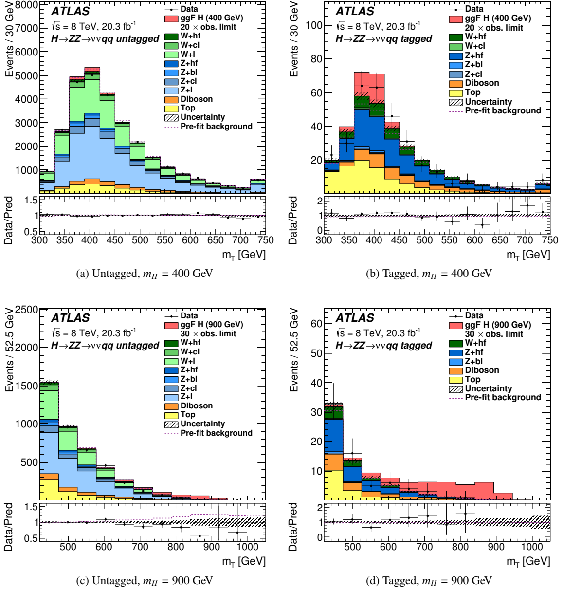
Figure 9: The distributions of m_T , the transverse mass of the Z(\nu\nu)Z(jj) system, used in the likelihood fit for the H \rightarrow ZZ \rightarrow \nu\bar{\nu}q\bar{q} search in the (a, c) untagged and (b, d) tagged channels, for Higgs boson mass hypotheses of (a, b) m_H = 400 GeV and (c, d) m_H = 900 GeV. The dashed line shows the total background used as input to the fit. For the m_H = 400 GeV hypothesis (a, b) the simulated signal is normalized to a cross-section corresponding to twenty times the observed limit given in Section 11, while for the m_H = 900 GeV hypothesis (c, d) it is normalized to thirty times the observed limit. The contribution labelled as ‘Top’ includes both the t\bar{t} and single-top processes. The bottom panes show the ratio of the observed data to the predicted background.
