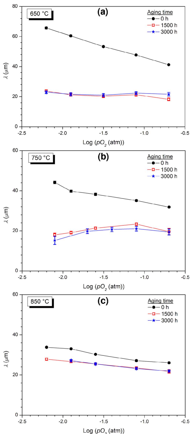
Figure 16. Dependence of the characteristic length \lambda on pO_2 at (a) 650 °C, (b) 750 °C and (c) 850 °C for LSM-YSZ cathodes after being aged at 900°C in humidified air.
