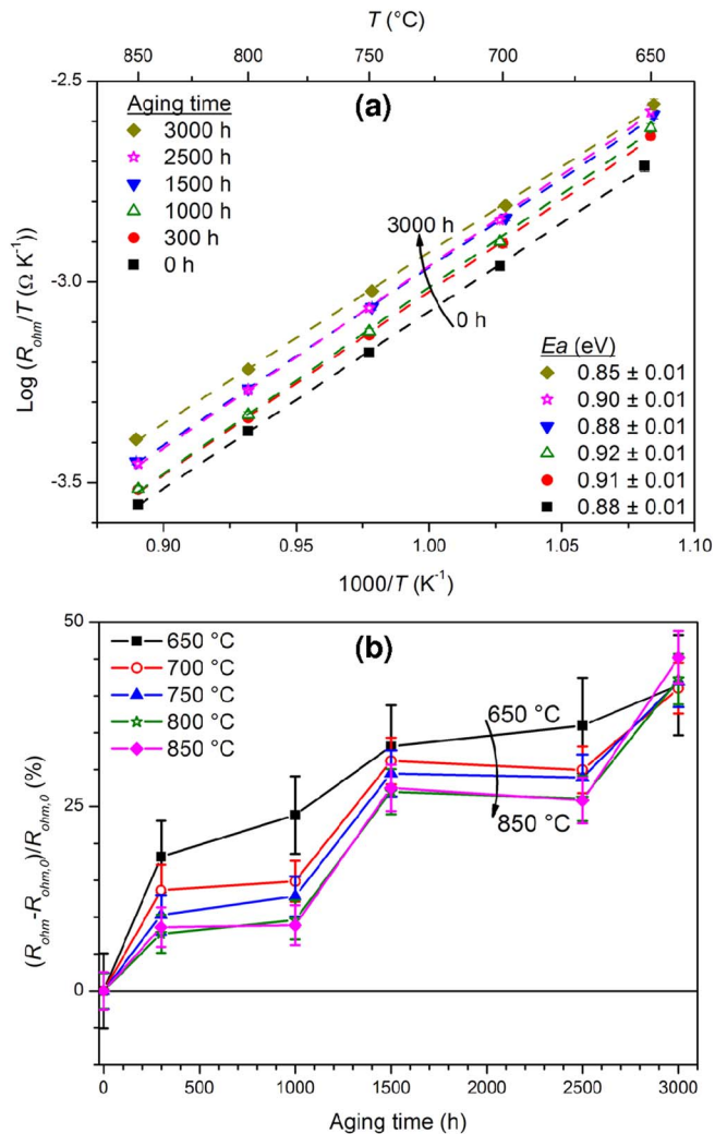
Figure 9. (a) Arrhenius plot and (b) relative percentage variation of R_{ohm} values for LSM-YSZ cathodes after being aged at 900 °C in humidified air. The arrows represent the direction of increasing aging time in (a) and of increasing temperature in (b).
