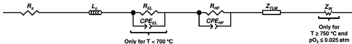
Figure 6. Equivalent circuit used to fit the spectra.
