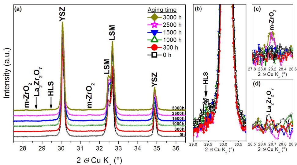
Figure 2. (a) Overview and (b,c,d) detail of XRD diffraction patterns collected at room temperature for LSM-YSZ cathodes after being aged at 900 °C in humidified air. HLS: Hump on the left shoulder (see text).
