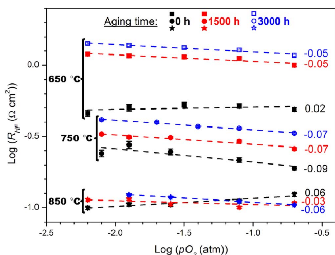
Figure 11. Dependence of R_{HF} on pO_2 at different temperatures for LSM-YSZ cathodes after being aged at 900°C in humidified air.
