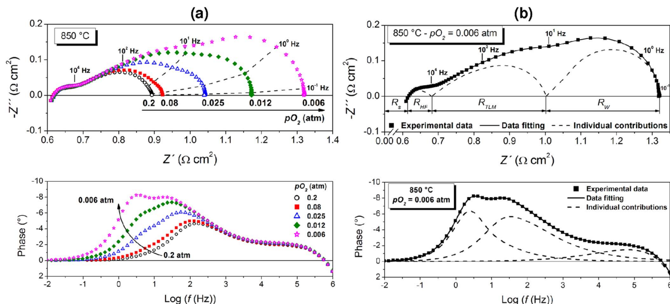
Figure 7. (a) Nyquist and Bode plots of impedance spectra for the reference sample (0 h) recorded at 850°C under different oxygen partial pressures. (b) Fitting of the impedance spectra recorded under pO_2 = 0.006 atm.
