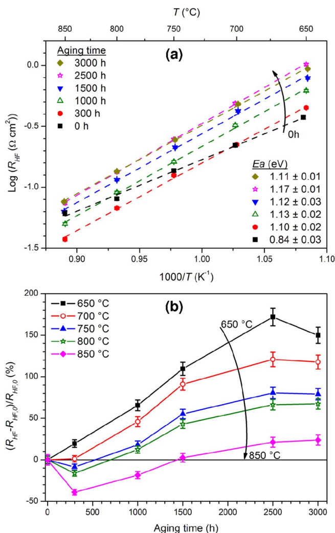
Figure 10. (a) Arrhenius plot and (b) relative percentage variation of R_{HF} values for LSM-YSZ cathodes after being aged at 900°C in humidified air. The arrows represent the direction of increasing aging time in (a) and of increasing temperature in (b).
