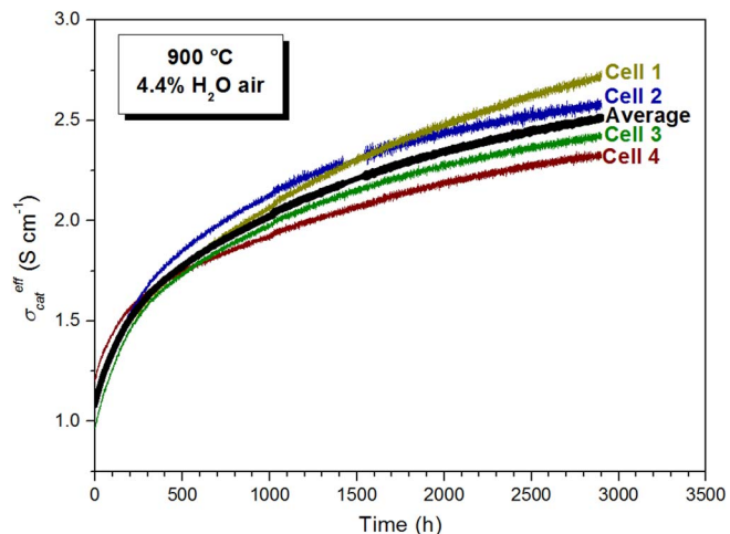
Figure 4. Conductivity data of four nominally identical LSM-YSZ cathodes measured at 900^\circ\text{C} in air containing 4.4% \text{H}_2\text{O} . The average values of the four cathodes are also shown.
