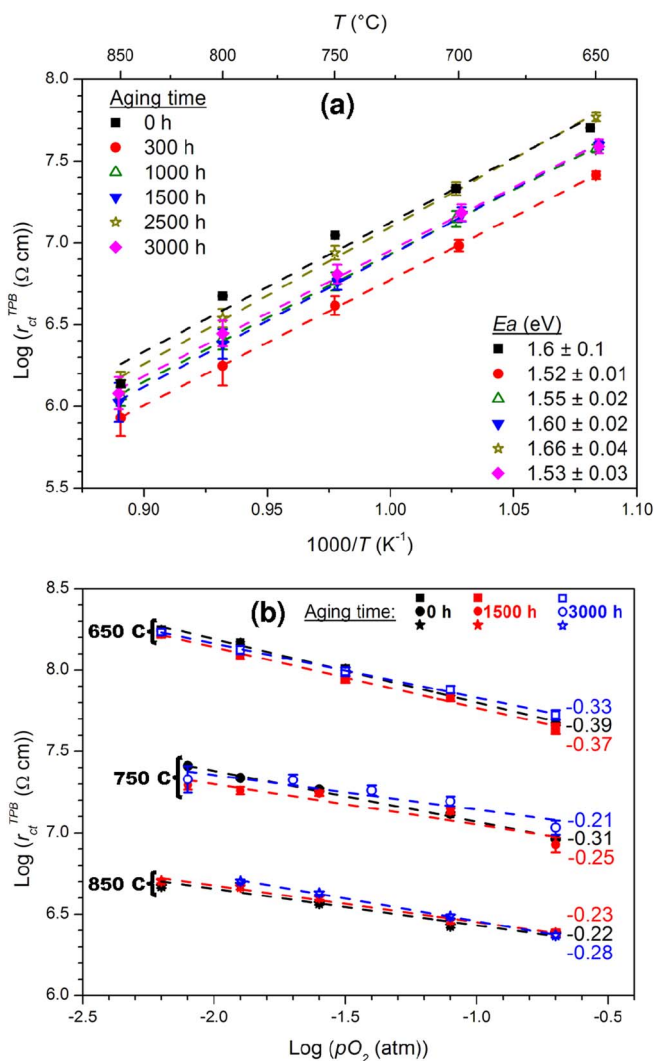
Figure 14. (a) Arrhenius plot and (b) dependence on pO_2 of the TPB specific charge transfer resistance values for LSM-YSZ cathodes after being aged at 900°C in humidified air.
