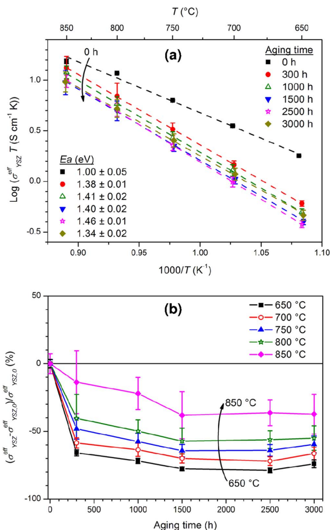
Figure 12. (a) Arrhenius plot and (b) relative percentage variation of conductivity values of the YSZ network for LSM-YSZ cathodes after being aged at 900°C in humidified air. The arrows represent the direction of increasing aging time in (a) and of increasing temperature in (b).
