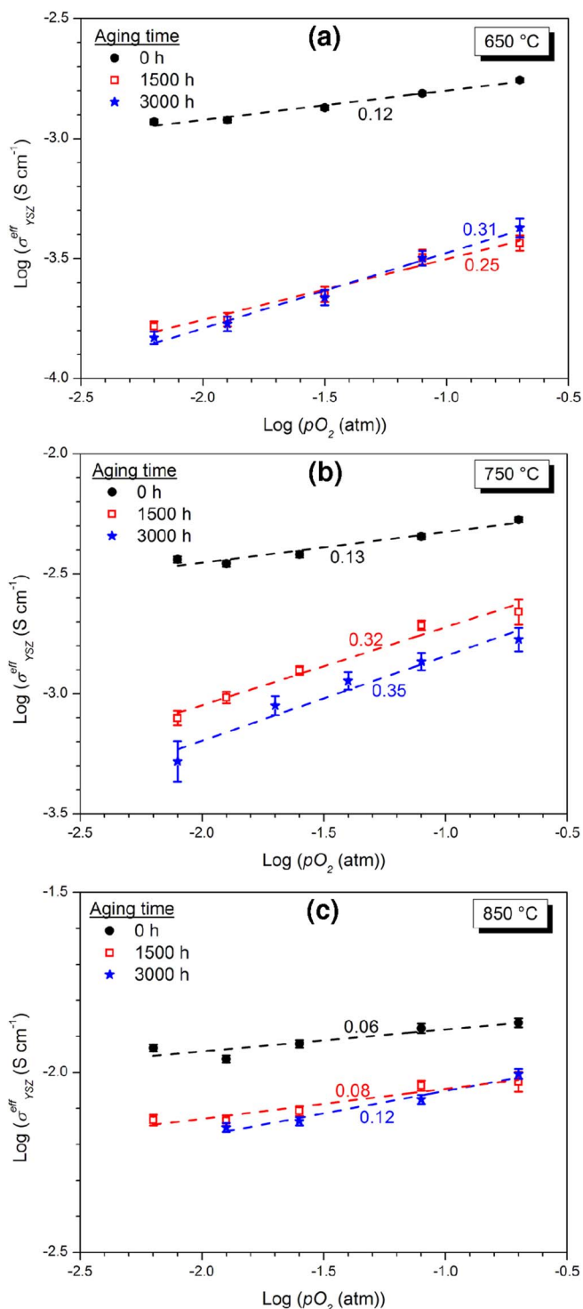
Figure 13. Dependence on pO_2 of conductivity values of the YSZ network at (a) 650°C, (b) 750°C and (c) 850°C for LSM-YSZ cathodes after being aged at 900°C in humidified air.
