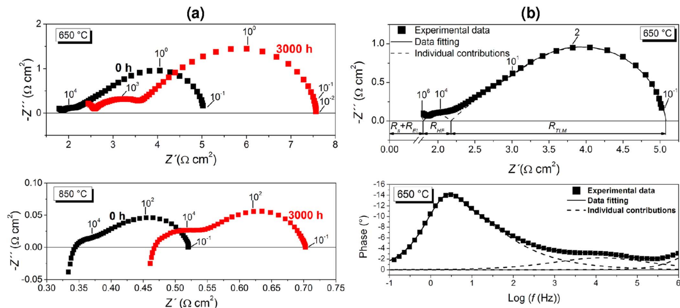
Figure 5. (a) Nyquist plot of impedance spectra for the reference and the 3000 h aged samples recorded in dry air at 650^\circ\text{C} (top) and 850^\circ\text{C} (bottom). The numbers indicate the frequency in Hertz. (b) Nyquist and Bode plots showing the fitting of the impedance spectra recorded at 650^\circ\text{C} for the reference sample (0 h).
