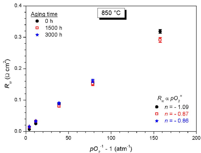
Figure 17. Dependence on pO_2 of R_w values at 850^\circ\text{C} for LSM-YSZ cathodes after being aged at 900^\circ\text{C} in humidified air.
