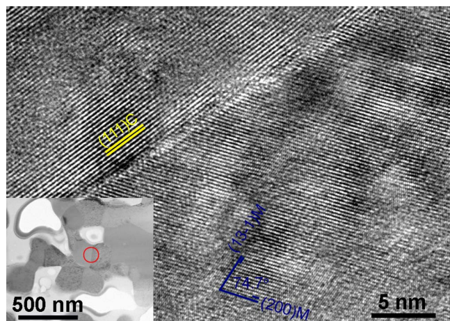
Figure 3. HR-TEM image of the circled area (of the inset, low-magnification TEM image) in the 3000 h aged sample.
