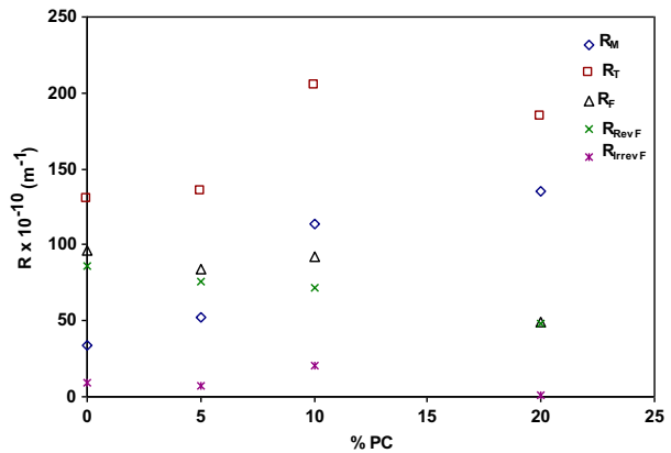
Fig. 5. Membrane resistances as a function of PC/PVDF content.
