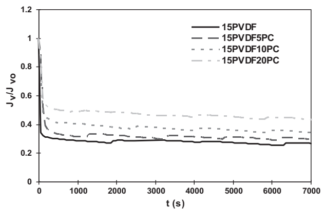
Fig. 6. J_v/J_{v0} vs. time for the synthesized membranes.
