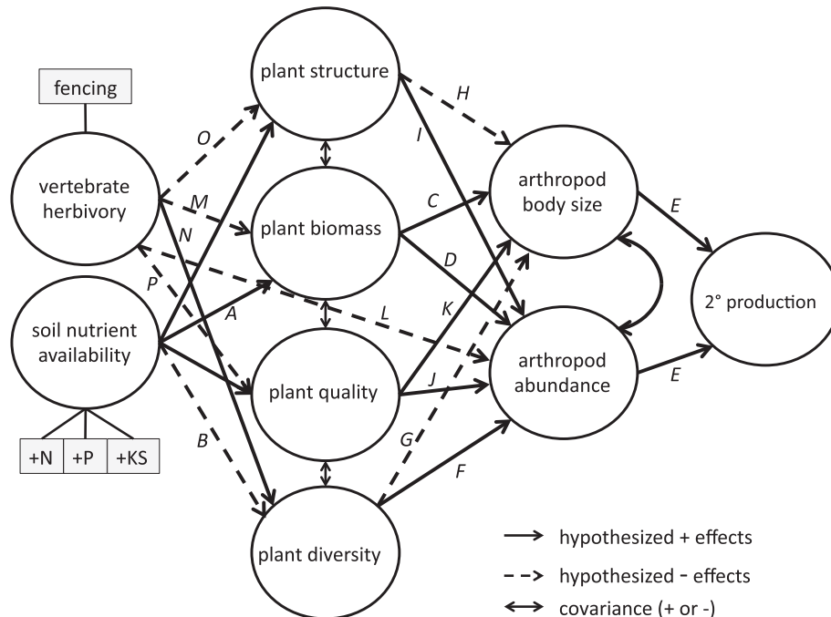
FIG. 1. Metamodel used as basis for evaluating links between soil nutrient availability, mammalian herbivory, and consumer biomass. Hypothesized sign of influence is indicated. Gray boxes indicate factors manipulated in the experiment to alter the connected variable. Double-headed arrow indicates covariance between arthropod body size and number; similar covariances among all plant response variables were included in the analysis but not displayed in the metamodel for clarity. Letters indicating paths correspond to hypotheses discussed in the main text.
