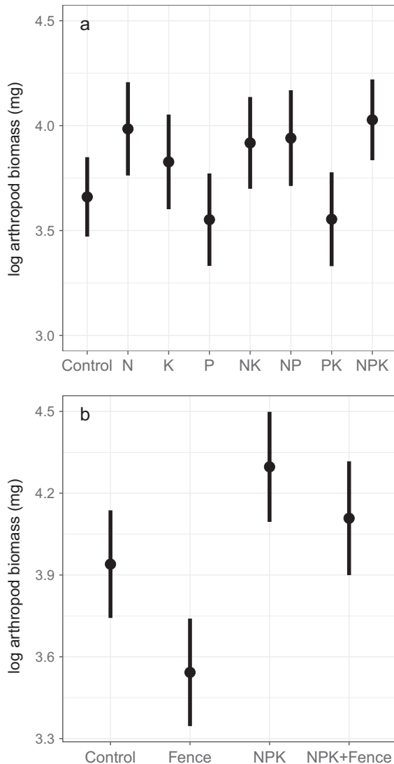
FIG. 2. Effects of (a) soil nutrient availability and (b) mammalian herbivore removal and their interaction on arthropod biomass. Points are modeled estimates of mean log biomass per meter squared, error bars represent standard error of model estimates.
