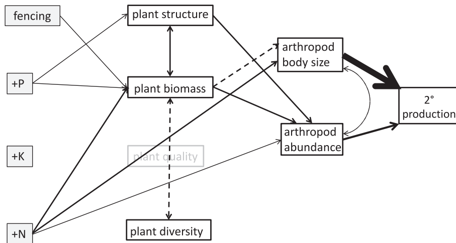
FIG. 3. Path analysis of the response of arthropod biomass to manipulations of soil nutrients and mammalian herbivory. Overall model Fisher's C = 12.68 , k = 16 , P = 0.696 . Paths with effects significantly different from zero using corrected P -values are drawn in width in proportion to their strength as either positive (solid line) or negative (dashed line) in sign. Double-headed arrows represent modeled covariances. Effect sizes of all paths and their significance are presented in Table 2. Variables are all per-plot, as follows: +N,+P,+K,+fence = indicator of treatment; plant diversity = Inverse Simpson's diversity index of plant community; plant biomass = live plant biomass in \text{g}/\text{m}^2 ; plant structure = mass of thatch in \text{g}/\text{m}^2 ; arthropod abundance = number of arthropods; arthropod body size = per capita mean mass of arthropods; 2° production = total arthropod biomass.
