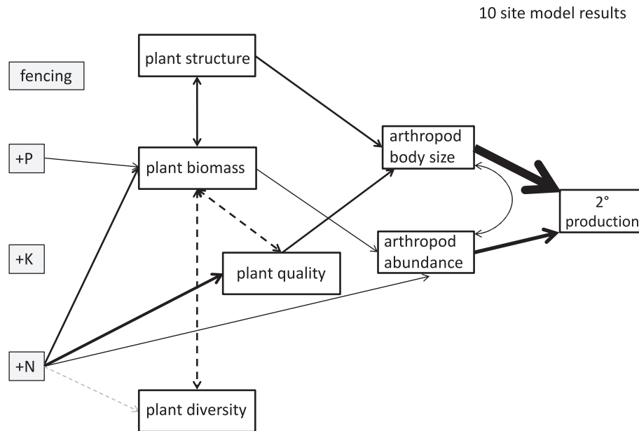
FIG. 4. Path analysis of the response of arthropod biomass to manipulations of soil nutrients and mammalian herbivory, including data for plant biochemical composition. Overall model Fisher's C = 41.67 , k = 34 , P = 0.172 . Paths with effects significantly different from zero using corrected P -values are drawn in width in proportion to their strength as either positive (solid line) or negative (dashed line) in sign. Double-headed arrows represent modeled covariances. Effect sizes of all paths and their significance are presented in Table 4. Variables are all per-plot, as follows: +N,+P,+K,+fencing = indicator of treatment; plant diversity = Inverse Simpson's diversity index of plant community; plant biomass = live plant biomass in \text{g/m}^2 ; plant structure = mass of thatch in \text{g/m}^2 ; plant quality = negative mean foliar C:N ratio of dominant plant species; arthropod abundance = number of arthropods; arthropod body size = per capita mean mass of arthropods; 2° production = total arthropod biomass.
