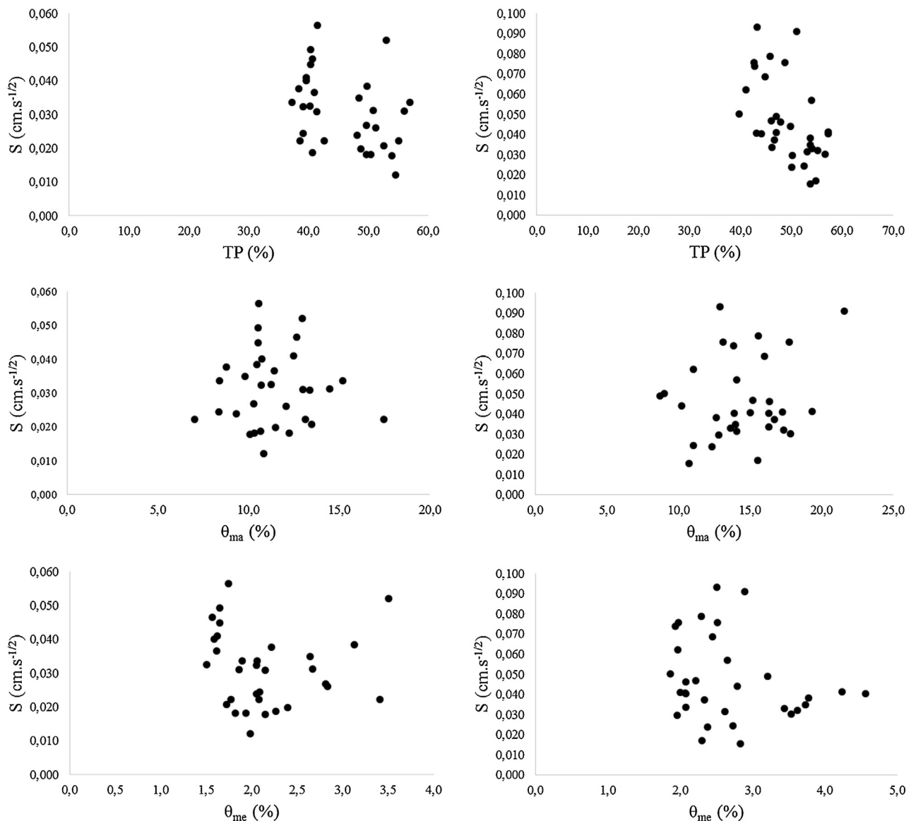
Fig. 3. Dependence of S on different pore size fractions: TP (Total porosity), macroporosity, \theta_{ma} (diameter > 60 \mu\text{m} ) and mesopores, \theta_{me} (30 \mu\text{m} < diameter < 60 \mu\text{m} ), for both treatments: NT (No Tillage, left) and CT (Conventional Tillage, right).
