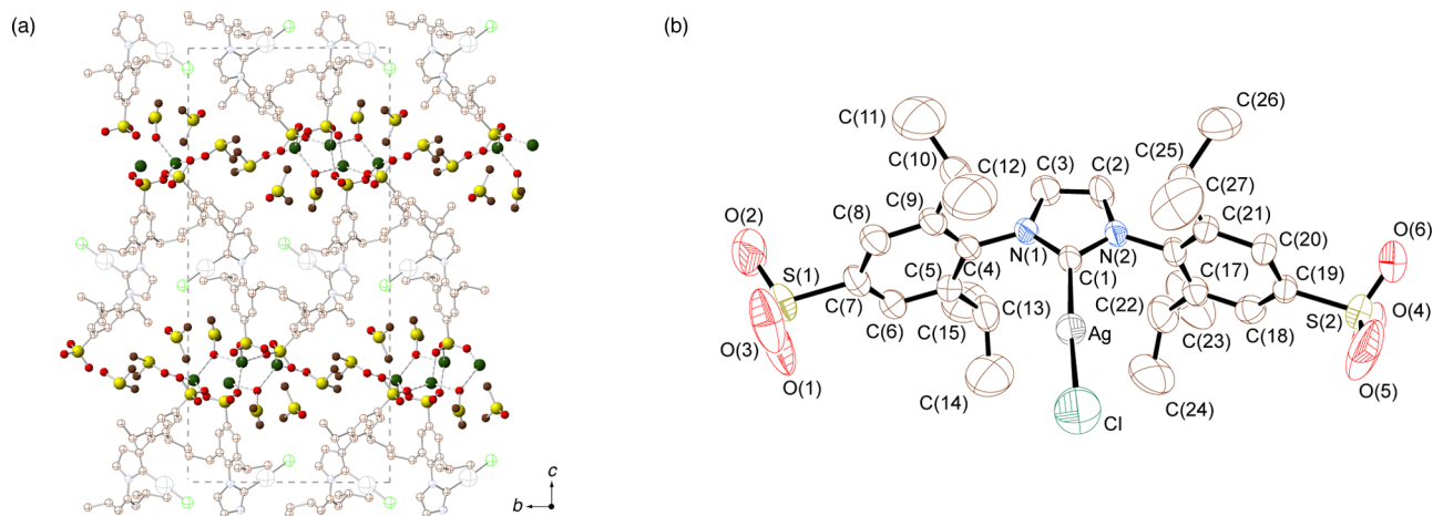
Figure 5. (a) View of the crystal structure of 3e along the crystallographic a axis highlighting the interactions of Na + ions with the sulfonate groups of the [AgCl(NHC)] 2- moieties and with the dmsol molecules. (b) ORTEP diagram (50% probability ellipsoids) of the organometallic moiety of 3e (H and Na atoms omitted for clarity). Selected bond lengths (Å) and angles (deg): Ag–C(1), 2.063(7); Ag–Cl, 2.298(3); C(1)–N(2), 1.354(8); C(1)–N(1), 1.344(8); C(2)–N(2), 1.359(9); C(3)–N(1), 1.377(9); C(2)–C(3), 1.351(10); C(1)–Ag–Cl, 176.6(2); N(1)–C(1)–N(2), 104.3(5).
