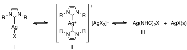
Scheme 3. Equilibria Involving Different Structures Found for Silver(I) NHC Complexes
