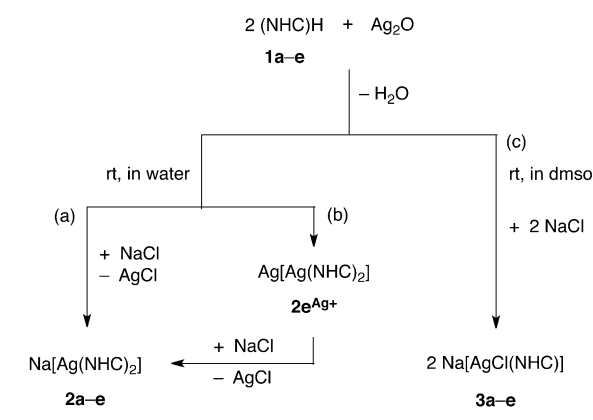
Scheme 1. Formation of Bis- ( 2 ) and Mono(carbene) ( 3 ) Complexes of Silver(I) with Sulfonated NHC Ligands
