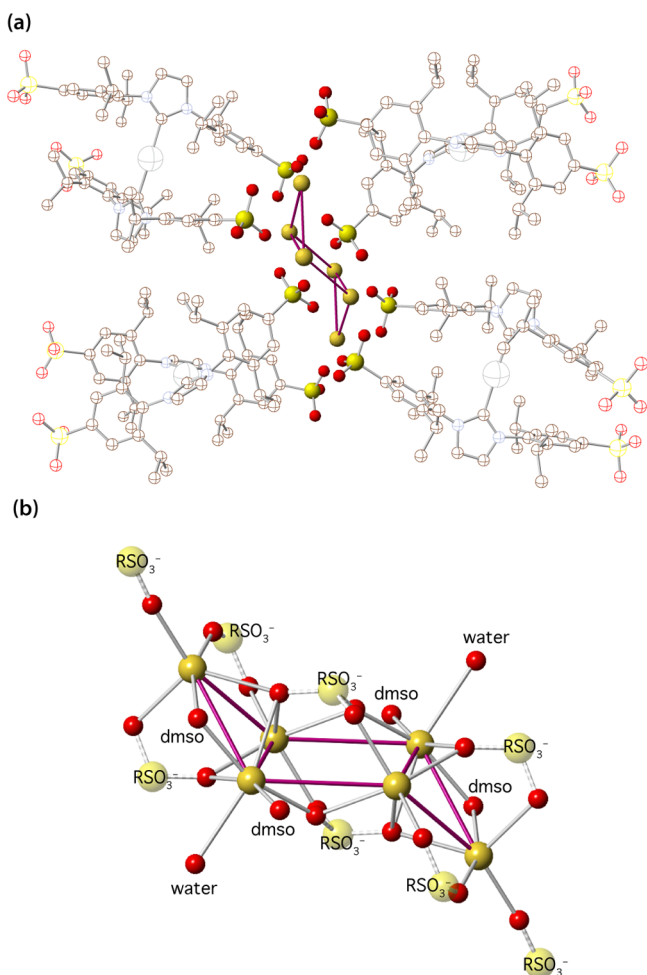
Figure 4. (a) Packing diagram showing the arrangement of [Ag(NHC) 2 ] 3- moieties in 2e·5Me 2 SO·H 2 O around a chairlike hexanuclear cluster of sodium ions. Solvent molecules have been omitted for clarity. (b) Detail of the hexanuclear cluster of sodium ions and its coordination sphere formed by oxygen atoms from sulfonate groups, dmsol, and water.
