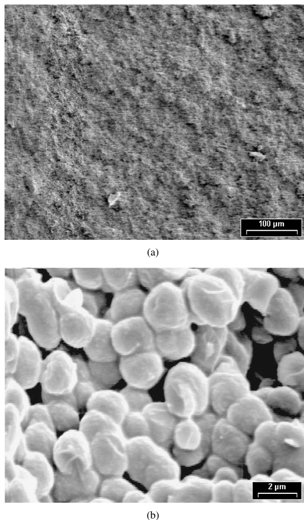
Figure 4 SEM of fracture surfaces. (a) DVERL-S/10%CTBN at 200 \times and (b) DVERL-S/100%CTBN at 7800 \times .
