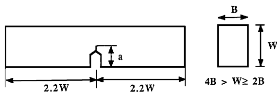
Figure 1 Schematic of the fracture specimen geometry.
