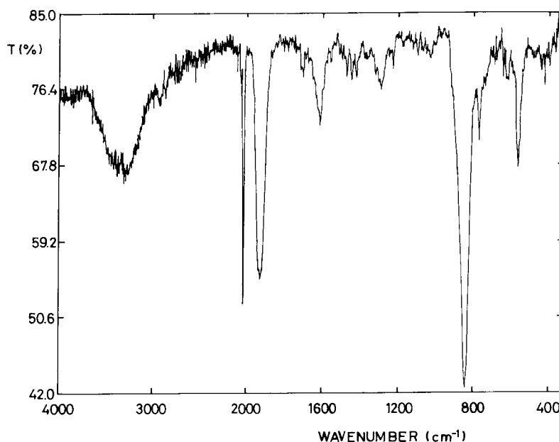
FIGURE 1 IR spectrum of [(\text{bpy})(\text{CO})_3\text{Re}^{\text{I}}(4,4'\text{-bpy})\text{Ru}^{\text{II}}(\text{NH}_3)_5](\text{PF}_6)_3 \cdot 4\text{H}_2\text{O} (KBr pellet).
