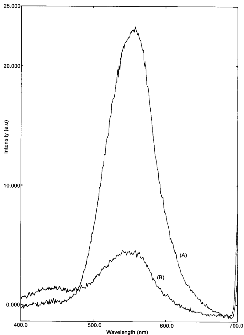
FIGURE 6 Emission spectra, in MeCN, at 22°C, of (A): [(bpy)(CO)_3Re^I(4,4'-bpy)]^+ and (B): [(bpy)(CO)_3Re^I(4,4'-bpy)Ru^{III}(NH_3)_5]^{4+} ( \lambda_{ex} = 350 nm).
