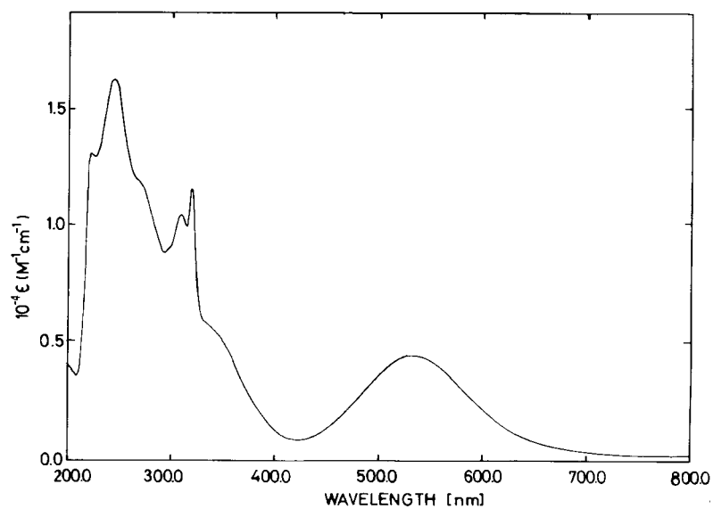
FIGURE 3 UV-visible spectrum of [(\text{bpy})(\text{CO})_3\text{Re}^{\text{I}}(4,4'\text{-bpy})\text{Ru}^{\text{II}}(\text{NH}_3)_5]^{3+} in MeCN.
