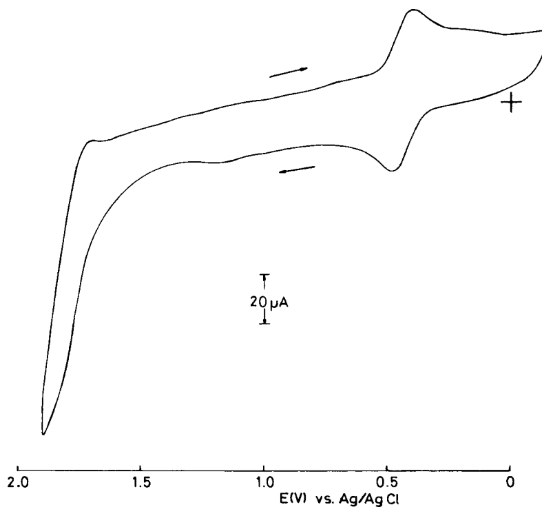
FIGURE 5 Cyclic voltammogram of complex (I) in MeCN, 0.1 M TBAH, \nu = 200 \text{ mV/s} .
