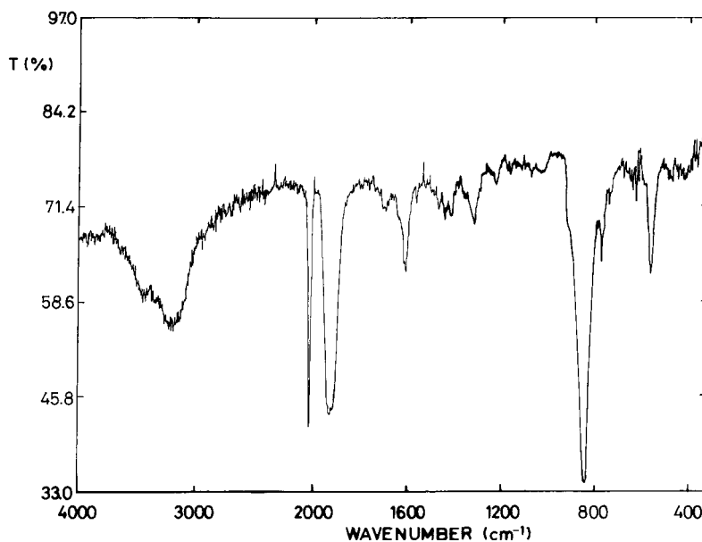
FIGURE 2 IR spectrum of [(bpy)(CO)_3Re^I(4,4'-bpy)Ru^{III}(NH_3)_5](PF_6)_4 (KBr pellet).
