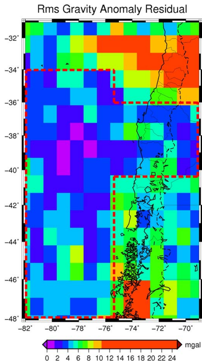
Fig. A.3. Root mean square of the gravity anomaly residual on 1 \times 1 tiles. Red dashed line indicates the most reliable areas to apply the EGM2008 model.
