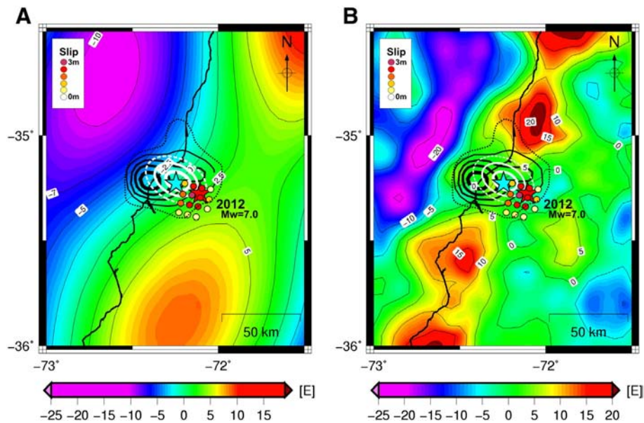
Fig. C.1. Slip model for the Constitucion 2012 Mw = 7.0 aftershock of Maule 2010 (Ruiz et al., 2013) superimposed to GOCE (A) and to EGM2008 model (B). The red and blue stars are the epicenters of the 2012 earthquake computed using the P1 and P2 waves, respectively. Slip distribution obtained from teleseismic records (color dots), together with InSAR images and GPS data (thick black line contours slip from 1 m to 0 m thin black dotted line) and from GPS and strong motion records (thick white line contours slip from 2.14 m to 0 m thin white dotted line 0 m).
