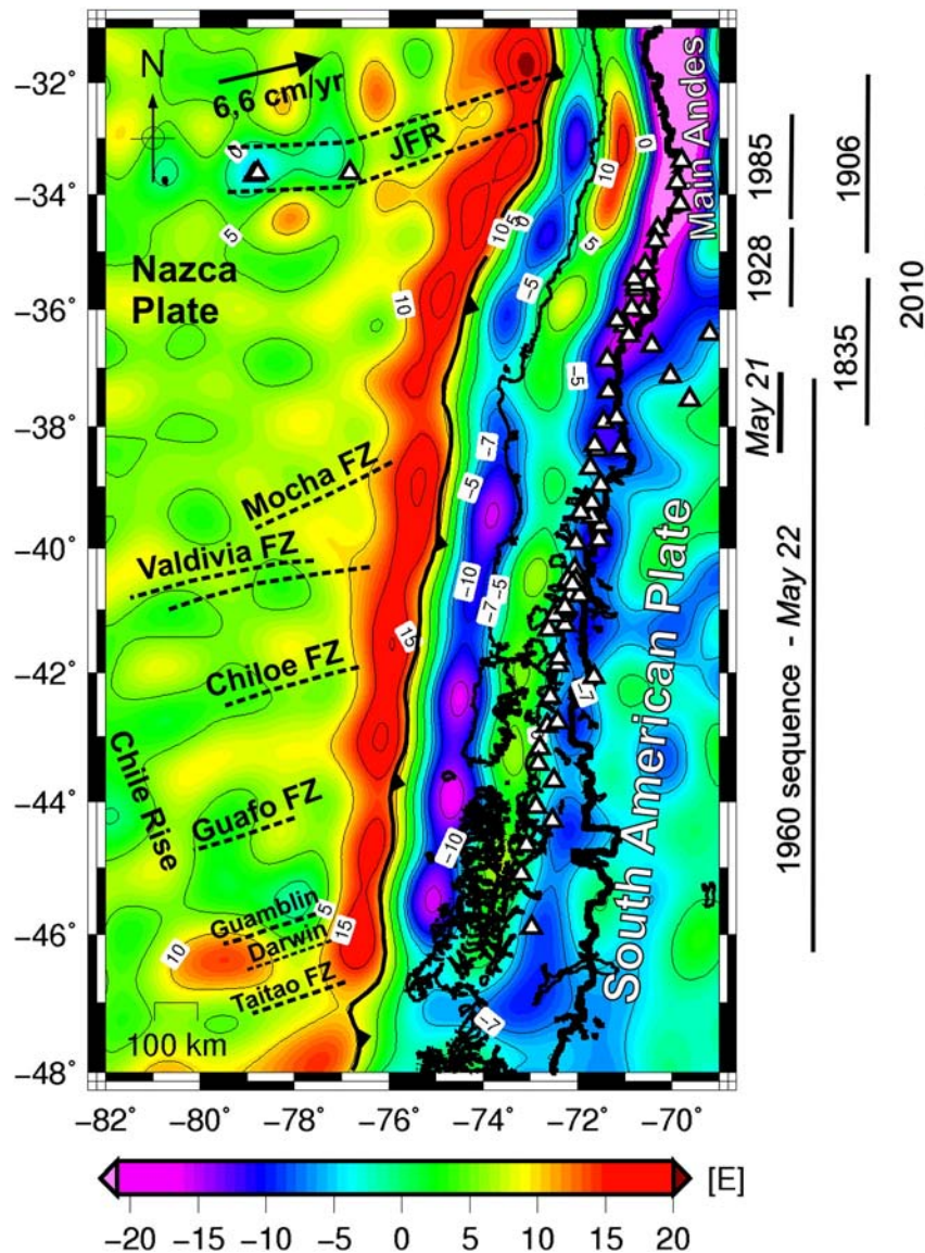
Fig. 2. Topography corrected Vertical Gravity Gradient ( T_{zz} ) obtained from GOCE (Pail et al., 2011) and Nazca plate Hof's (dashed lines). To the right the dimensions of the approximate rupture areas of the largest earthquakes along the Chile margin are indicated: Valparaíso-1985 , M_w = 8.0 : Barrientos (1988, 1995); Mendoza et al. (1994). Valparaíso-1906 , M_s = 8.4 : Beck et al. (1998). Talca-1928 , M_s = 8.0 : Beck et al. (1998); Campos et al. (2002); Ruegg et al. (2009). 1835 Concepción-Constitución seismic gap , M_w = 8.5 : Campos et al. (2002); Darwin (1840, 1876); FitzRoy (1839); McCann et al. (1979). Maule-2010 , M_w = 8.8 : Lay et al. (2010); Lorito et al. (2011); Moreno et al. (2012); Vigny et al. (2011); among others. Concepción May 21-1960 , M_w = 8.2 : Cifuentes (1989); Engdahl and Villaseñor (2002); Plafker and Savage (1970). Valdivia May 22-1960 , M_w = 9.5 : Moreno et al. (2009); Plafker and Savage (1970); Ruegg et al. (2009). Triangles indicate the current position of the active volcanic arc (Siebert and Simkin, 2002). Coastal line: thin black line, National borders: thick black line.
