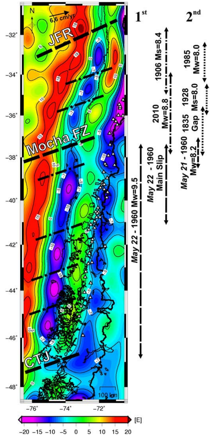
Fig. 8. Different orders of barriers/attenuators proposed that segment the southern Chilean subduction zone, based on T_{zz} from GOCE satellite data constrained by the available rupture zones for large megathrust earthquakes ( M_w \geq 8.0 ).
