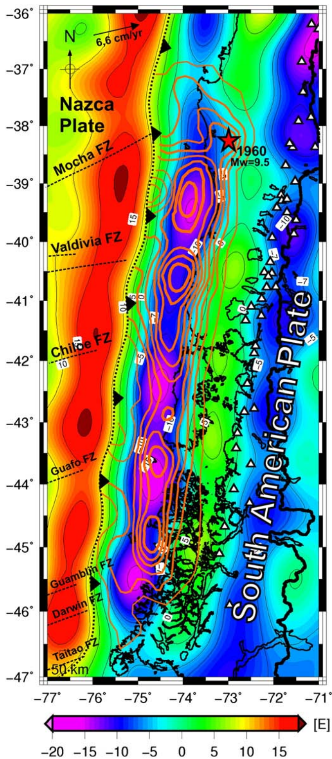
Fig. 5. Fault slip distribution contours predicted by the precise 3D FEM model of Moreno et al. (2009) superimposed to GOCE Vertical Gravity Gradient in the zone of the Valdivia 1960 earthquake. The northern -10 Eötvös contour coincides with slip distribution pattern. South of 42^{\circ}\text{S} the correspondence is not so clear, showing a shift between the Tzz lows and the slip model. As mentioned in the text, Moreno et al. (2009) reported that south of Isla de Chiloé ( 42^{\circ}\text{S} ) data used for the inversion are not as reliable as in the northern zone.
