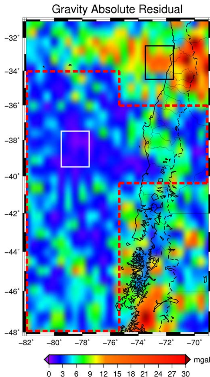
Fig. A.1. Absolute difference between the gravity anomaly from EGM08 and GOCE. The black square in the vicinity of the JFR shows an area with erroneous data. The white square shows an area over the Nazca Plate (Near Mocha FZ) with better quality data. Red dashed line indicates the most reliable areas to apply the EGM2008 model. Argentinian/Chilean border indicated by dotted and dashed line; coastal border indicated by black line.
