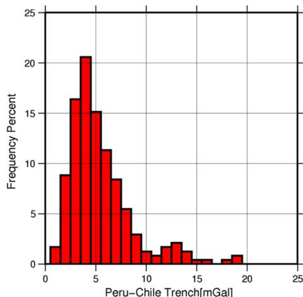
Fig. A.4. Histogram of the rms deviations on 1 \times 1 tiles.
