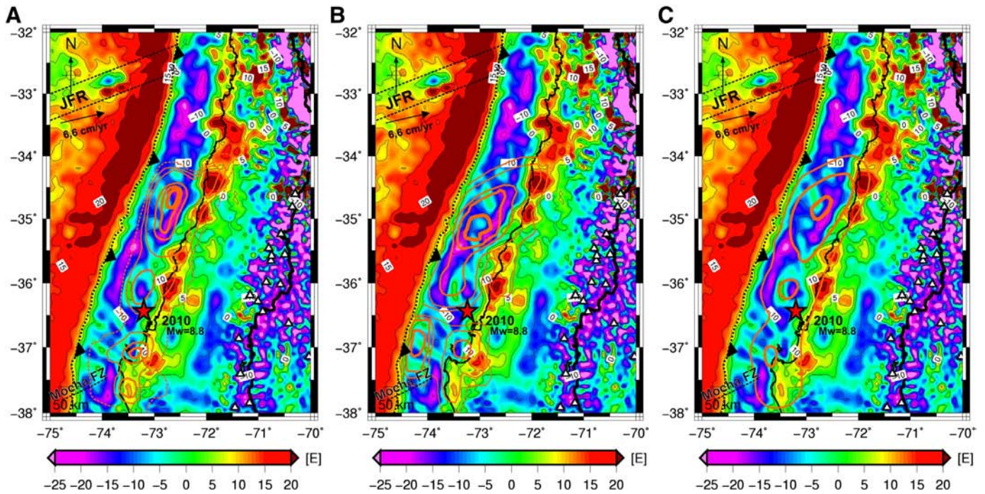
Fig. B.1. EGM2008 Vertical Gravity Gradient in the zone of the Maule 2010 earthquake, superimposed with fault slip distribution contours obtained by the joint inversion of: A: INSAR, near and far cGPS (Tong et al., 2010). B: Survey GPS, near field and far field cGPS data, land-level variation and INSAR (Vigny et al., 2011). C: Survey and continuous near and far field GPS data, INSAR, and land-level changes (Moreno et al., 2012). Note the agreement between the maximum displacements and lower Tzz values. The maximum slip for the southern patch (at the Arauco peninsula) coincides with a low Tzz value.
