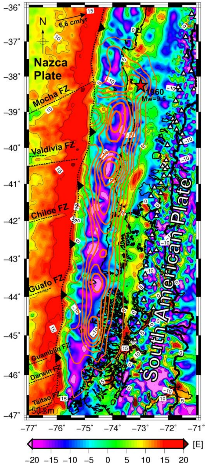
Fig. D.1. EGM2008 Vertical Gravity Gradient in the zone of the Valdivia 1960 earthquake, superimposed with fault slip distribution contours predicted by the precise 3D FEM model from Moreno et al. (2009).
