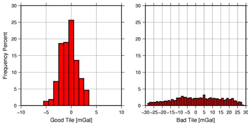
Fig. A.2. Histogram of the residual gravity anomaly between EGM08 and GOCE (up to degree and order N = 250 ). Left (Good tile): white square of Fig. A.1. Right (Bad tile): black square of Fig. A.1.
