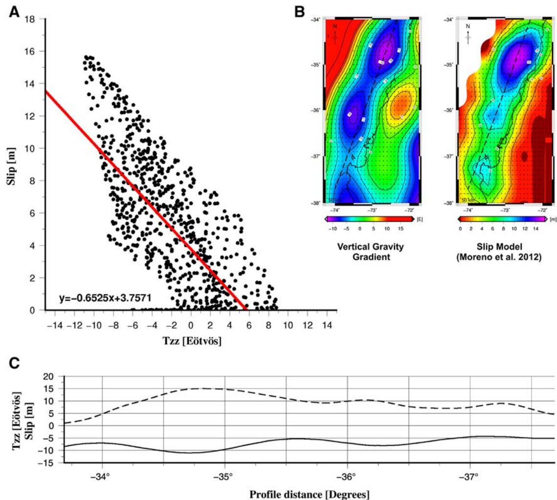
Fig. 7. A) Plot of T_{zz} field versus slip model both sampled over a regular grid (B) and profile along T_{zz} and slip distribution. In both representations an inverse relationship between both quantities is observed (high slip over negative T_{zz} ).
