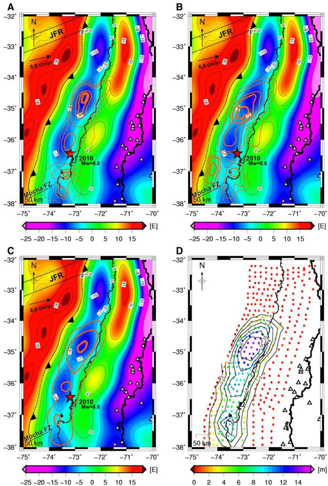
Fig. 6. GOCE vertical gravity gradient in the zone of the Maule 2010 earthquake, superimposed to fault slip distribution contours obtained by A: (Tong et al., 2010). B: (Vigny et al., 2011). C: (Moreno et al., 2012). Note the correlation between the northern patch for the slip models and the lobes with low T_{zz} values. D: Coseismic slip model for the 2010 Maule earthquake (Moreno et al. (2012)).
