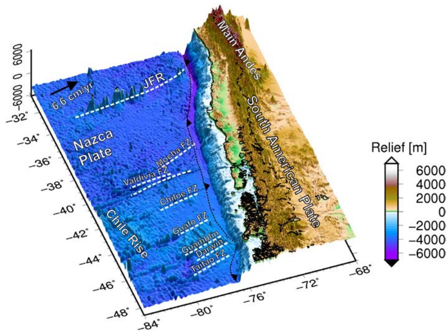
Fig. 1. Morphology of the oceanic Nazca plate highlighting the main topographical features that are subducted at the Chilean trench (Amante and Eakins, 2009). Note the differences in sediment thickness north and south of the Mocha Fz, and the JFR. Nazca/South America convergence rate is approximately 6.6 cm/yr with a convergence angle of 78°N (DeMets et al., 2010; Kendrick et al., 2003). Chilean/Argentinian border is indicated by dotted and dashed line; coast line by black line; dotted line indicates Chilean trench.
