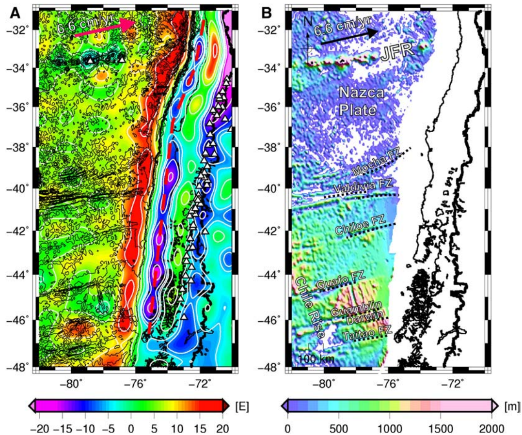
Fig. 3. (A): Relation between the variable relief of the oceanic floor and the segmentation of the Tzz signal. Black contours delineate bathymetry, while white contours show the Tzz segmentation. Red arrow indicates the convergence direction between Nazca and South American plates. Red dashed line shows the Tzz profile location of Fig. 4. (B): Positive relief of the oceanic Nazca plate relative to the mean seafloor depth of approximately -4000 m. (For interpretation of the references to color in this figure legend, the reader is referred to the web version of this article.)
