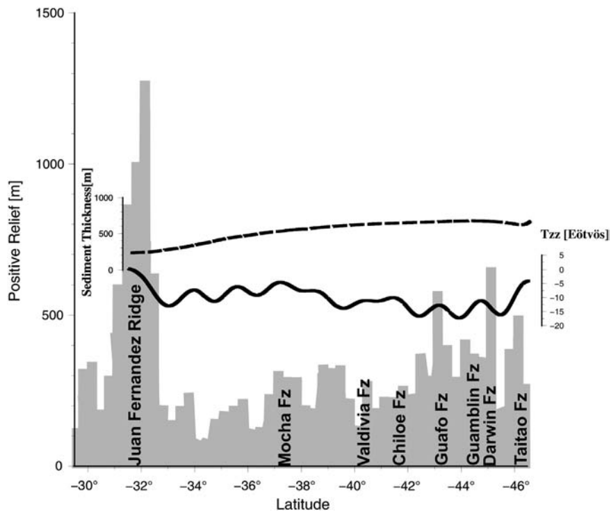
Fig. 4. Latitudinal cross section of the inferred subducted seafloor relief through the Nazca plate beneath the accretionary prism (gray shaded). Superimposed is the Tzz signal (black line). Note the general correlation that exists between bathymetry and Tzz. The observed little shift is a consequence of the obliquity between bathymetry profiles and Tzz (see Fig. 3) related to the convergence direction and because the Tzz signal has a long wavelength characteristic. Black dashed line delineates the sediment thickness from Whittaker et al. (2013).
