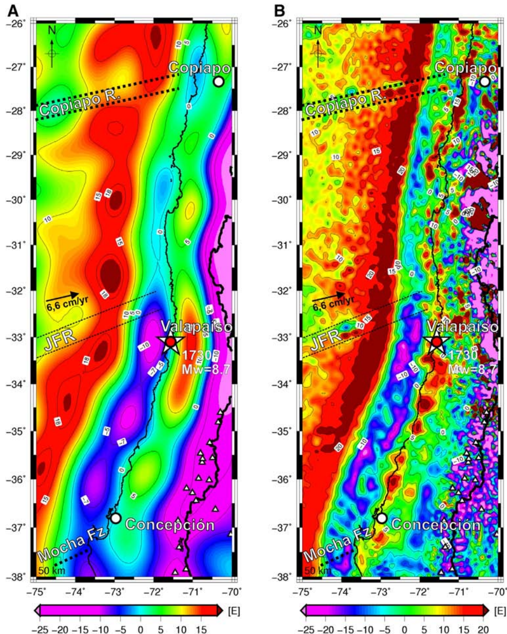
Fig. E.1. Tzz from GOCE (A) and from EGM2008 model (B) depicts important differences north of the JFR over the seismogenic zone. This reflects a decrease in sediment thickness north of JFR and no trench sediment infill at all north of Copiapo as explained by many authors (e.g. Bangs and Cande, 1997; Flueh et al., 1998; Laursen et al., 2002; Schweller et al., 1981; Völker et al., 2006; von Huene et al., 1997).
