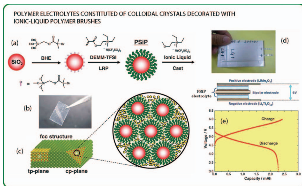
FIGURE 14 (a) Preparation process for novel PSiP/IL-solid electrolyte with three-dimensionally assembling PSiPs. (b) Photograph of produced solid film. (c) Analyzed structure of PSiP array in the solid state. (d) Photograph and illustrated bipolar-cell structure. (e) charge/discharge curve of a lithium-ion battery using PSiP/IL solid electrolyte. From Sato et al., Adv. Mater. , 2011, 23, 4868, © Wiley-VCH Verlag GmbH & Co. KGaA, reproduced by permission.
