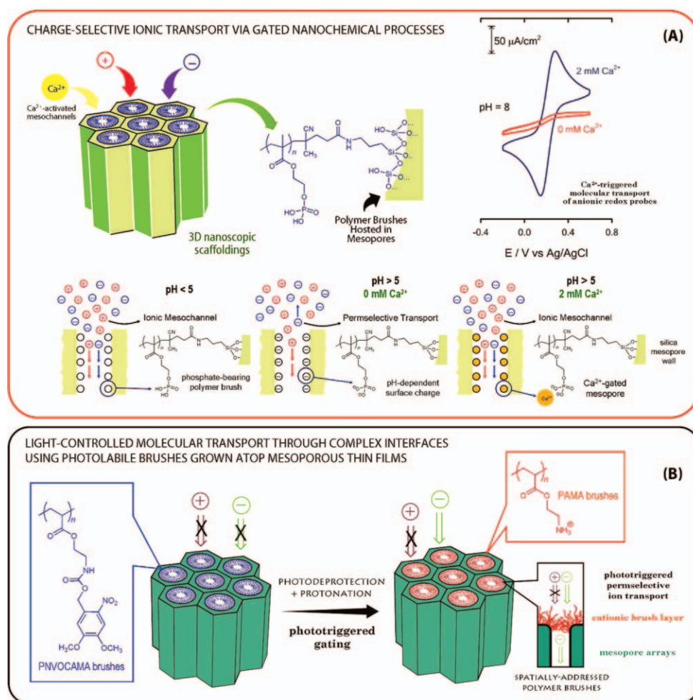
FIGURE 11 (A) Schematic depiction of the ionic transport processes taking place in mesoporous thin films modified with phosphate-bearing polymer brushes (PMEP) under different pH conditions and in the presence or in the absence of Ca 2+ ions. Cyclic voltammograms (on the right) describe the molecular transport through PMEPP-modified mesoporous thin films in the absence and in the presence of Ca 2+ using Fe(CN) 6 3- as a redox probe. From Brunsen et al., Langmuir , 2012, 28, 3583, © American Chemical Society, reproduced by permission. (B) Schematic representation describing the modification of mesoporous silica films with photolabile polymer brushes and their subsequent “uncaging” to build up a permselective polycationic barrier in the outer region of the film. From Brunsen et al., Chem Commun. , 2012, 48, 1422, © Royal Society of Chemistry, reproduced by permission.
