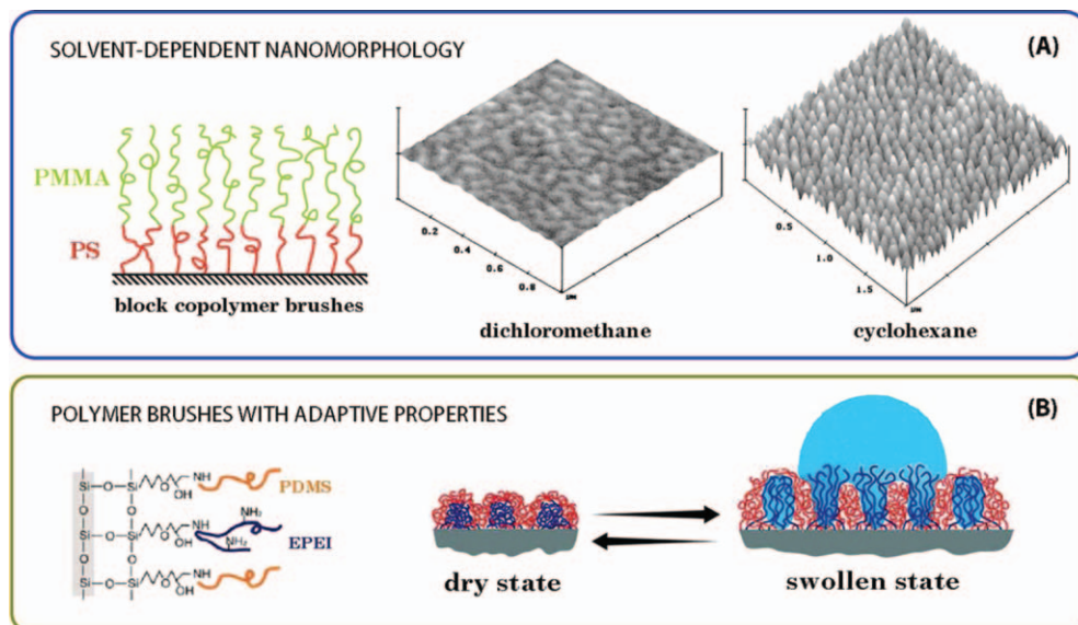
FIGURE 6 (A) Solvent-selective reorganization of poly(methyl methacrylate)/poly(styrene) block copolymer brushes (PMMA- b -PS) attached to surfaces through the PS chain end. After cyclohexane/dichloromethane treatment the PS blocks preferentially come to the surface due to favorable solvent-PS interactions. From Boyes et al., Surf. Sci. 2004, 570, 1-12, © Elsevier B.V., reproduced by permission. (B) Schematic depiction of the reversible film reorganization/segregation of hybrid polymer brushes constituted of highly branched ethoxylated polyethylenimine (EPEI) and poly(dimethylsiloxane) (PDMS) in air and under water conditions. From Motornov et al., Langmuir 2007, 23, 13-19, © American Chemical Society, reproduced by permission.
