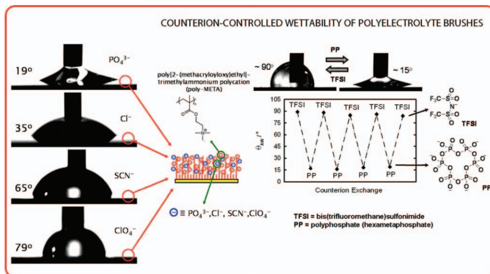
FIGURE 7 (Left) Wetting modulation of PMETA brushes grown on Au surfaces (thickness \sim 20 nm) in the presence of different counterions. (Right) Change in the wetting characteristics of PMETA brushes after exchanging the two contrasting counterions: TFSI and PP. From Azzaroni et al., Adv. Mater. 2007, 19, 151–154, © Wiley-VCH Verlag GmbH & Co. KGaA, reproduced by permission.
