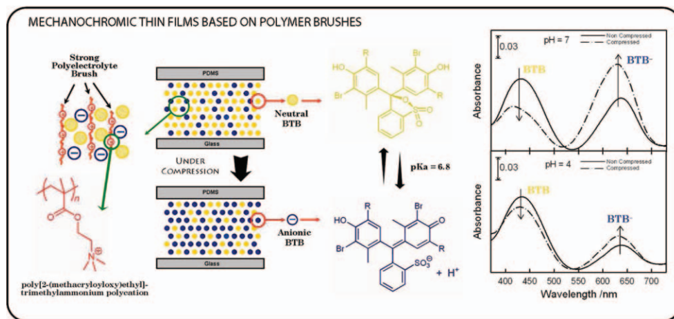
FIGURE 18 (Left) Simplified depiction of the variation in the population of neutral and anionic bromothymol blue (BTB) species inside PMETAC brush films upon compression. Also depicted in the schematic representation are the chemical structures corresponding to the cationic polyelectrolyte brush and the neutral and anionic form of the BTB dye. (Right) UV/Vis spectra corresponding to the compression experiments for BTB-loaded PMETAC brushes in a hydrated environment at different pH values: (a) pH 7 and (b) pH 4. Dotted and solid lines refer to spectra taken under compression and with no compression, respectively. The arrows indicate the direction of changes upon compression. From Azzaroni et al., Angew. Chem. Int. Ed. , 2006, 45, 7440, © Wiley-VCH Verlag GmbH & Co. KGaA, reproduced by permission.
