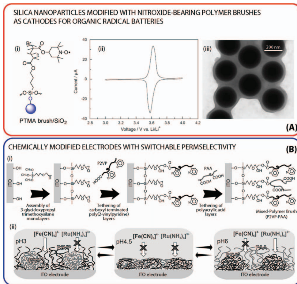
FIGURE 13 (A) Scheme of poly(2,2,6,6-tetramethylpiperidin-1-oxyl-4-yl methacrylate), (PTMA) brush on silica nanoparticles. (ii) Cyclic voltammogram for the PTMA brush/silica nanoparticles composite electrode in 1.0 M LiClO 4 . (iii) TEM micrographs of PTMA brush/silica nanoparticles. From Lee et al., J. Power Sources , 2011, 196, 8098, © Elsevier B.V., reproduced by permission. (B) (i) Stepwise modification of the ITO electrodes to yield the mixed polymer brush composed of P2VP and PAA. (B) Simplified scheme describing the polymer brush permeability for the differently charged redox probes controlled by the solution pH value: (a) the positively charged protonated P2VP domains allow the electrode access for the negatively charged redox species; (b) the neutral hydrophobic polymer thin-film inhibits the electrode access for all ionic species; (c) the negatively charged dissociated PAA domains allow the electrode access for the positively charged redox species. From Katz et al., Electroanalysis 2010, 22, 35, © Wiley-VCH Verlag GmbH & Co. KGaA, reproduced by permission.
