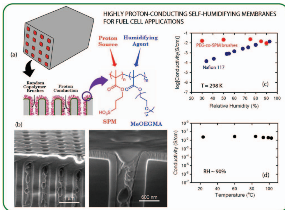
FIGURE 15 (a) Chemical structure of the random copolymer brush and simplified illustration of the ordered two-dimensional macroporous silicon membrane modified with the polymer brushes. (b) Scanning electron micrographs corresponding to the silicon membrane modified with polySPM-co-MeOEGMA brushes. (c) Conductivity versus relative humidity plots corresponding to the silicon membrane modified with polySPM-co-MeOEGMA brushes and Nafion 117 membrane. (d) Conductivity versus temperature plot corresponding to the silicon membrane modified with polySPM-co-MeOEGMA brushes. From Azzaroni et al., Angew. Chem. Int. Ed. , 2009, 48, 3124, © Wiley-VCH Verlag GmbH & Co. KGaA, reproduced by permission.
