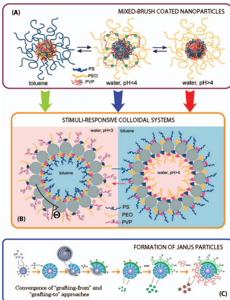
FIGURE 4 (A) Schematic representation of responsive particles generated through the grafting of mixed copolymer brushes on the surface of silica nanoparticles. (B) Cartoon describing the structure of oil-in-water and water-in-oil emulsions stabilized by responsive hairy nanoparticles. Panels (A) and (B) were From Motornov et al., Adv. Funct. Mater. , 2007, 17, 2307-2314, © Wiley-VCH Verlag GmbH & Co. KGaA, reproduced by permission. (C) Scheme of the preparation of bicomponent Janus particles by grafting from and grafting to approaches. From Berger et al., Macromolecules , 2008, 41, 9669-9676, © American Chemical Society, reproduced by permission.
