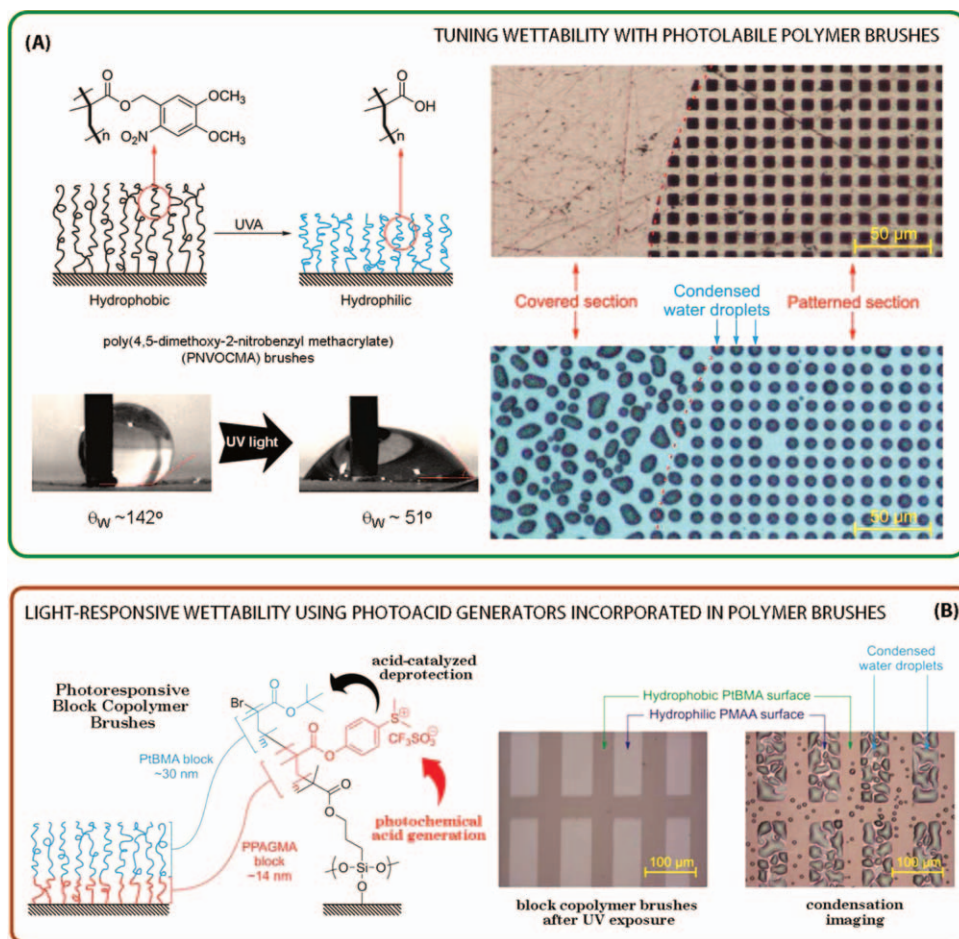
FIGURE 8 (A) Chemical and wettability changes occurring when PNVOCMA brushes are converted to PMAA brushes upon exposure to UV light. The figure also depicts a condensation picture, taken by optical microscopy, of a PNVOCMA brush after patterned deprotection. From Brown et al., Langmuir 2009, 25, 1744, © American Chemical Society, reproduced by permission. (B) (Left) Simple schematic of PPAGMA- b -PtBMA brush. (Right) PPAGMA- b -PtBMA polymer brush after patterned UV exposure and the subsequent condensation imaging of the same sample revealing the hydrophilicity of the exposed regions. From Brown et al., Soft Matter 2009, 5, 2738, © Royal Society of Chemistry, reproduced by permission.
