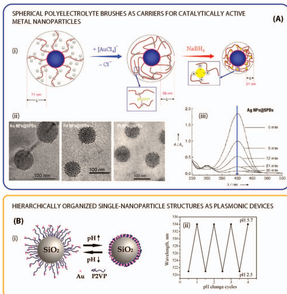
FIGURE 12 (A) (i) Schematic representation of the generation of gold nanoparticles inside spherical brushes (SPBs). (ii) Cryo-TEM images of different metal NPs encapsulated in spherical polyelectrolyte brush particles. From Ballauff et al., Macromol. Rapid Commun. , 2009, 30, 806 and Macromol. Symp. 2007, 254, 42, © Wiley-VCH Verlag GmbH & Co. KGaA, reproduced by permission. (iii) Reduction of 4-nitrophenol by \text{NaBH}_4 in the presence of AgNPs@SPB. UV/Vis spectra of solutions of 4-nitrophenol measured at different times. From Ballauff et al., Angew. Chem. Int. Ed. , 2006, 45, 813, © Wiley-VCH Verlag GmbH & Co. KGaA, reproduced by permission. (B) (i) Schematic representation of the pH-responsive behavior of a AuNPs@P2VP-SiO 2 . (ii) Maximum wavelength of the surface plasmon peak as a function of pH change in the cycle between 2.5 and 5.7. From Minko et al., Langmuir , 2008, 24, 8976, © American Chemical Society, reproduced by permission.
