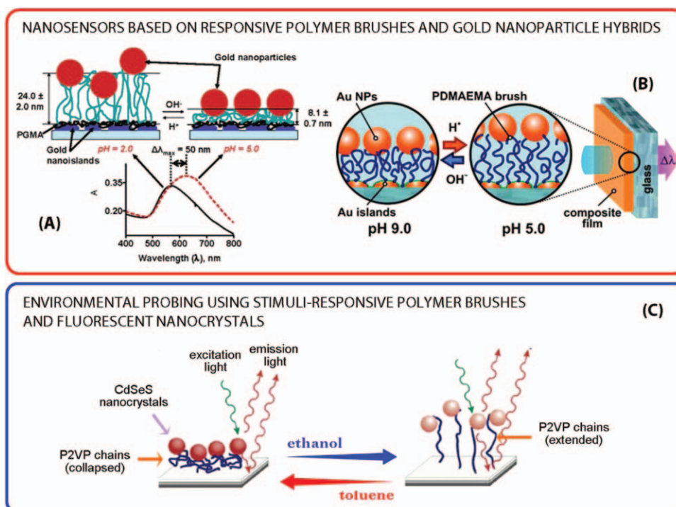
FIGURE 10 (A) Simplified scheme of the reversible pH change-induced swelling of gold nanoparticle-coated poly(2-vinylpyridine) (P2VP) polymer brushes and the corresponding SPR spectra AuNP/P2VP brushes at pH 2.0 and 5.0. From Tokareva et al., J. Am. Chem. Soc. , 2004, 126, 15950, © American Chemical Society, reproduced by permission. (B) Plasmonic sensing platform constituted of responsive ultrathin PDMAEMA brushes, Au nanoislands and Au NPs. From Tokarev et al., ACS Appl. Mater. Interfaces , 2011, 3, 143, © American Chemical Society, reproduced by permission. (C) Schematic of the polymeric sensor. Hydrophobic nanocrystals are adsorbed on a stimuli-responsive polymer layer that was previously grafted onto a reflecting substrate. The nanocrystal– surface distance depends on the conformation of the polymer chains and changes in different solvents. The change in height is then reported by a variation in the detected fluorescence intensity. From Ionov et al., Adv. Mater. 2006, 18, 1453, © Wiley-VCH Verlag GmbH & Co. KGaA, reproduced by permission.
