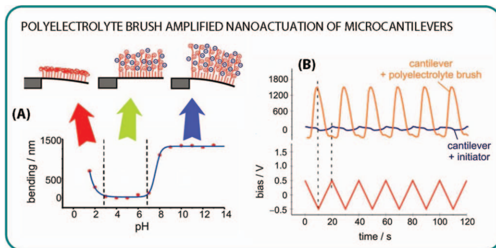
FIGURE 17 (A) Observed bending of single-side PMP brush-modified cantilever with changing pH and schematic illustration of brush conformation in different regimes. From Zhou et al., J. Am. Chem. Soc. 2006, 128, 5326, © American Chemical Society, reproduced by permission. (B) Actuation of PMETAC brush-modified cantilever in response to the applied bias. The actuation directly follows the applied bias without apparent lag; initiator-only cantilevers show a very small response to changes in electric field. From Zhou et al., Nano Lett. , 2008, 8, 725, © American Chemical Society, reproduced by permission.
