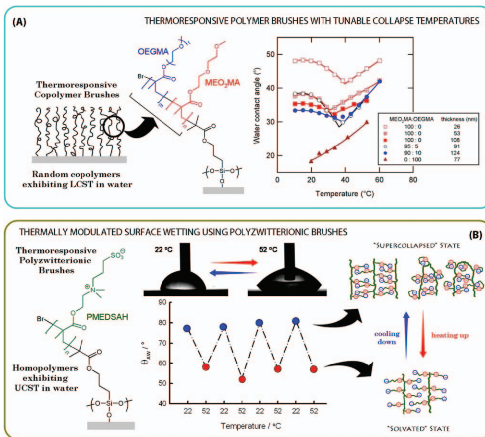
FIGURE 5 (A) (left) Simple schematic of copolymer brushes and chemical structure of P(MEO 2 MA-co-OEGMA) brushes – (right) equilibrium water contact angles of P(MEO 2 MA-co-OEGMA) brushes as a function of temperature. From Jonas et al., Macromolecules 2007, 40, 4403–4405, © American Chemical Society, reproduced by permission. (B) (left) Chemical structure of PMEDSAH brushes—(center) change of the wetting characteristics of thick, supercollapsed PMEDSAH brushes (thickness ~180 nm) after increasing the temperature from 22 °C to 52 °C and the corresponding representation of the contact angle in water as a function of temperature—(right) simple schematic of the conformational states in different temperature regimes: “supercollapsed” state (inter-chain and intrachain associations) at T < UCST and “solvated” state (nonassociated brush) at T > UCST . From Azzaroni et al., Angew. Chem. Int. Ed. 2006, 45, 1770–1774, © Wiley-VCH Verlag GmbH & Co. KGaA, reproduced by permission.
