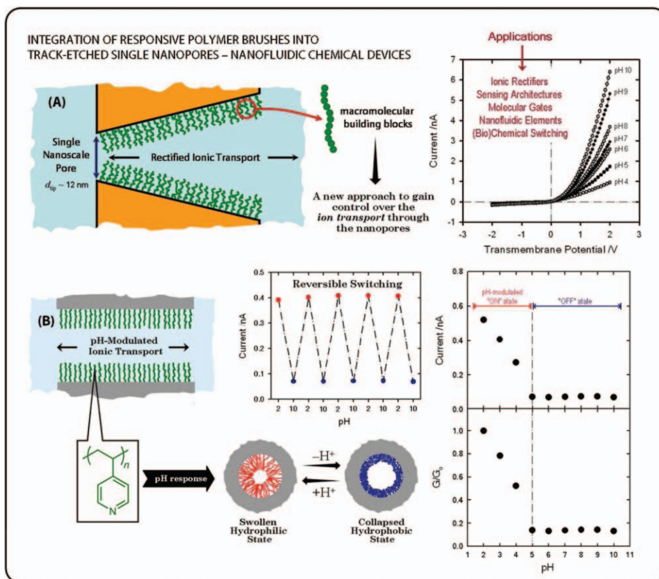
FIGURE 16 (A) (left) Schematic depiction of a conical nanopore modified with polymer brushes—(right) I–V curves corresponding to a single conical nanopore modified with poly 2-(methacryloyloxy) ethyl phosphate brushes measured at different pH values (using 0.1 M KCl as electrolyte). From Azzaroni et al., Chem Comm. 2010, 46, 1908, © Royal Society of Chemistry, reproduced by permission. (B) Simplified description of the cylindrical nanochannel modified with poly(4-vinyl pyridine) brushes, reversible variation of the transmembrane ionic current passing through the PVP brush-modified nanochannel upon alternating the environmental pH between 2 and 10, and representation of the transmembrane ionic current and the normalized nanochannel conductance as a function of the environmental pH for a PVP brush-modified cylindrical nanochannel. From Azzaroni et al., Nano Lett. 2009, 9, 2788, © American Chemical Society, reproduced by permission.
