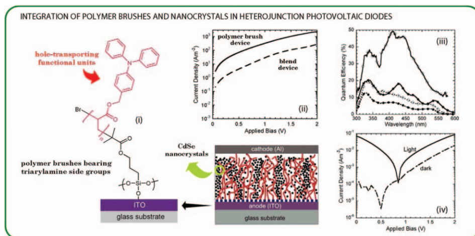
FIGURE 9 (A) (i) Chemical structure poly(triphenylamine acrylate) (PTPAA) brushes grafted from ITO electrodes. The figure also includes a simplified cartoon describing the inferred structure for CdSe nanocrystal infiltrated polymer brush photovoltaic device. (ii) Current-voltage characteristics for diodes fabricated with ITO anodes and Al cathodes with active layers of PTPAA brushes (45 nm) infiltrated with 2.6 nm diameter CdSe nanocrystals (solid line), PTPAA/CdSe nanocrystals blend 1:8 by weight (70 nm thick) (dashed line). (iii) Photovoltaic action spectra for a CdSe nanocrystal (2.6 nm diameter) infiltrated PTPAA brush (45 nm thick) device (open diamonds) and for PTPAA/CdSe nanocrystal blend device 1:8 by weight (solid circles), with external quantum efficiency (dotted lines) and internal quantum efficiency (solid lines). (iv) Current-voltage characteristics for a device comprising a 20 nm thick PTPAA brush film grown from a modified PEDOT:PSS coated ITO slide, infiltrated with 2.8 nm diameter CdSe nanocrystals and capped with an aluminum cathode, in the dark (dashed line) and under 400 nm incident illumination (solid line). From Snaith et al., Nano Lett. 2005, 5, 1653-1657, © American Chemical Society, reproduced by permission.
