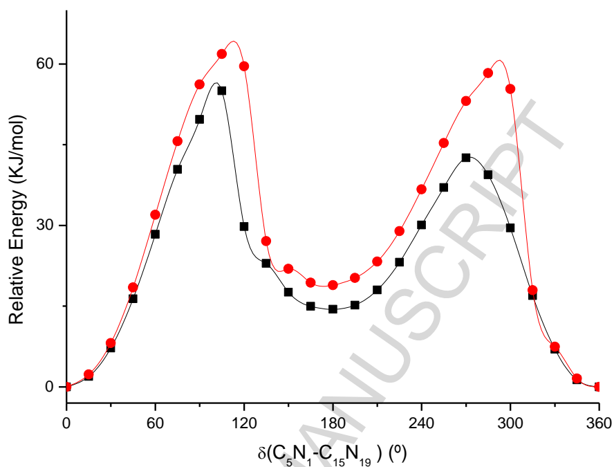
Figure 1. Calculated [B3LYP/6-31+G(d,p)] potential function for internal rotation around the \text{C}_5\text{N}_1-\text{C}_{15}\text{N}_{19} dihedral angle for MPTN (—■—) and FMPTN (—●—) compounds. For atom numbering see Scheme 1.
