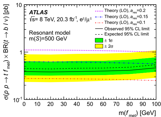
Fig. 6 Observed and expected limits on the cross section times branching ratio ( left ) for the resonant model with m(S) = 500 GeV and ( right ) for the non-resonant model, as a function of the mass of f_{\text{met}} and v_{\text{met}} ,
