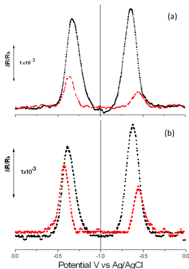
Figure 8. \delta R/R vs potential curves of Ru\alpha at 575 nm (a) and Ru\beta at 564 nm (b) in DMF:H_2O containing 0.1 M TBAPF 6 . These runs were recorded as a function of potentials in degassed (black trace) and CO_2 saturated solutions (red trace). The working electrode was a mirror-polished Pt disc subjected to a sine potential wave (11 Hz, 50 mV r.p.p. ) superimposed on a 2 mV/s potential scan.
