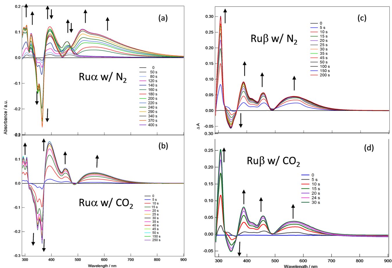
Figure 6. Transient \Delta A spectra of \text{Ru}\alpha ( 22\ \mu\text{M} ) during photolysis in \text{N}_2 (a) and in \text{CO}_2 (b) saturated DMF:TEA ( 0.25\ \text{M} )/ \text{H}_2\text{O} ( 1\ \text{M} ) solutions and \text{Ru}\beta ( 22\ \mu\text{M} ) during photolysis in \text{N}_2 (c) and in \text{CO}_2 (d) saturated DMF/TEA ( 0.25\ \text{M} )/ \text{H}_2\text{O} ( 1\ \text{M} ) solutions. Peaks pointing down indicate bands disappearing while those pointing up correspond to new bands appearing due to photolysis.
