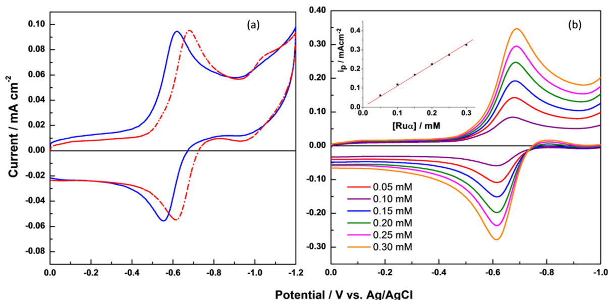
Figure 3. (a) Comparison of the cyclic voltammetric behavior of Ru \alpha (red dash line) and Ru \beta (blue solid line) in N 2 saturated DMF:H 2 O (1 M) solutions. Working electrode: glassy carbon disk (1 mm diameter), scan rate = 50 mV/s, complex concentration = 20 \mu M, supporting electrolyte = 0.1 M TBAPF 6 . (b) Effect of concentration on the voltammetric behavior of the first electroreduction process of Ru \alpha in solutions saturated with N 2 . The increase of the cathodic current peak with the complex concentration follows a linear relationship (shown in the inset plot).
