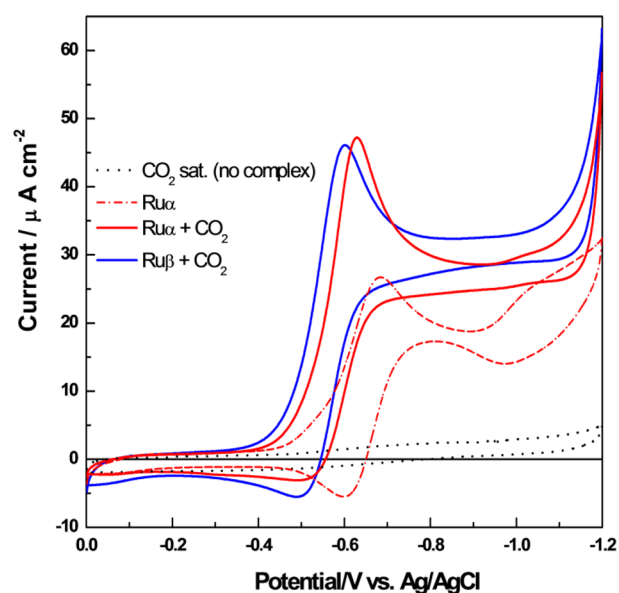
Figure 4. Comparison of the voltammetric behavior of Ru \alpha (red solid line) and Ru \beta (blue solid line) in DMF:H 2 O (1 M) solutions saturated with CO 2 . Voltammograms of Ru \alpha before saturation with CO 2 (red dash line) and that without Ru complex but with CO 2 (black dot line) are included as reference. All voltammograms were run at 5 mV/s with a glassy carbon working electrode.
