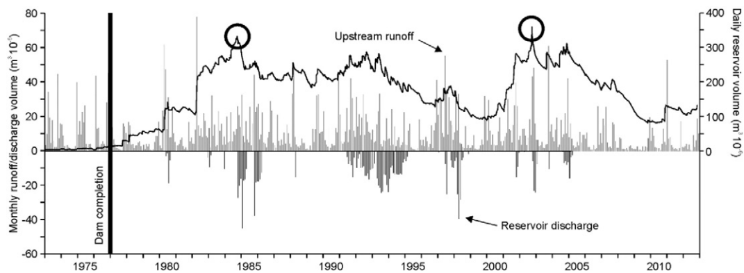
Fig. 2. Monthly runoff volume upstream from the dam and monthly volumes of reservoir discharge over the period 1973–2012. Upstream runoff volumes were estimated from rainfall using the GR2M model (Makhlouf and Michel, 1994). Monthly volumes of reservoir discharge over the period 1973–1988 were calculated by solving the reservoir water balance equation (missing data). Daily reservoir volumes were illustrated to provide an idea of the hydrological magnitude of the dam relative to that of the river. Circles indicate episodes of overflow spills.
