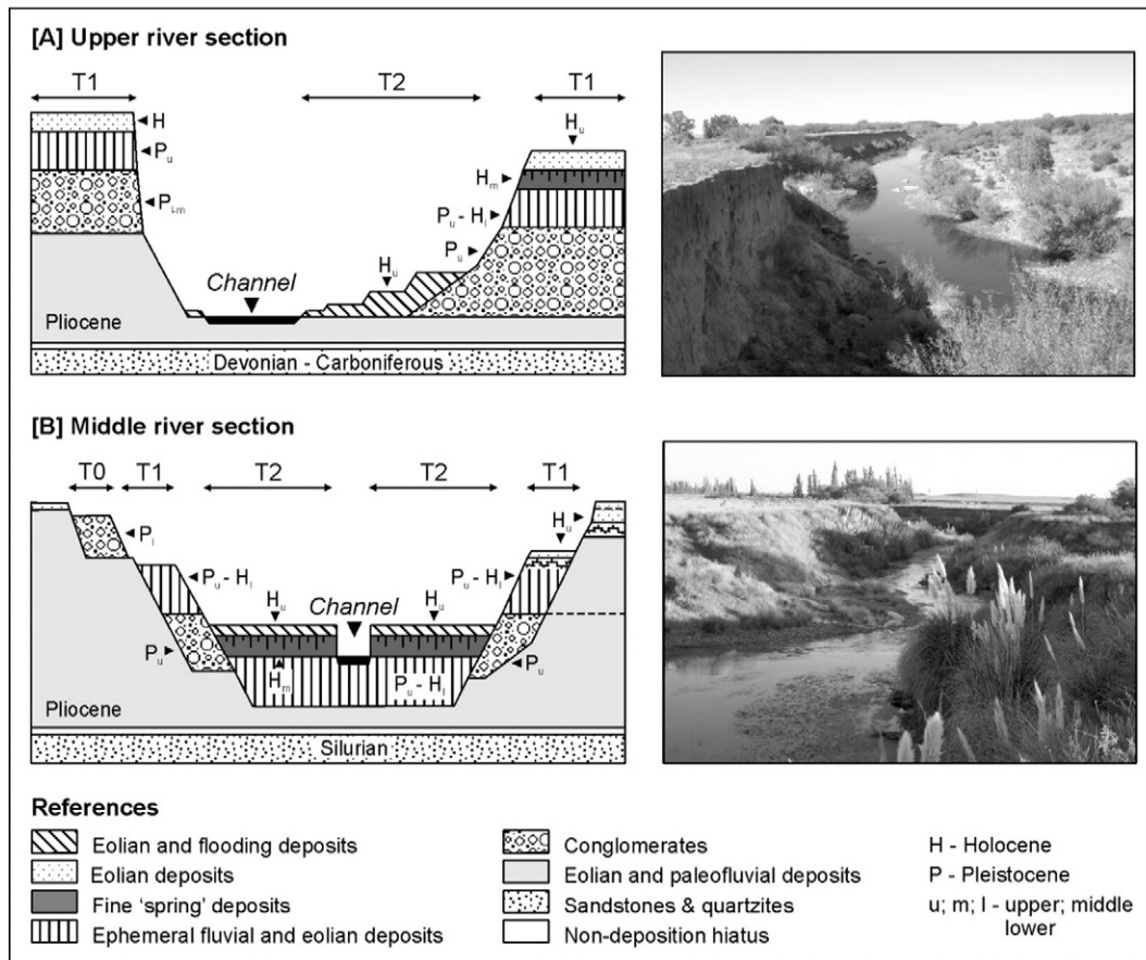
Fig. 3. Schematic cross sections of the Sauce Grande River showing typical geomorphic and geologic characteristics within the upper and middle river sections. Geologic features were modified from Borromei (1991) ; Zavala and Quattrocchio (2001) , and Quattrocchio et al. (2008) . Not to scale.
