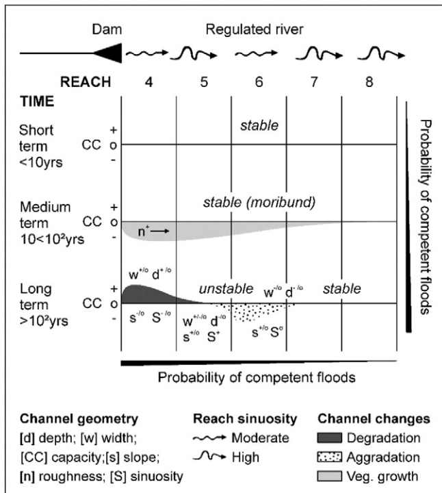
Fig. 11. Adjustment of the channel morphology to extreme flow regulation below water-storage reservoirs in drylands. The model of adjustment (modified from Petts, 1979) considers the potential for change relative to the frequency and intensity of competent floods with time and distance from dam closure. The direction of change is indicated by [o] no significant change, [+] increase, and [–] decrease.
