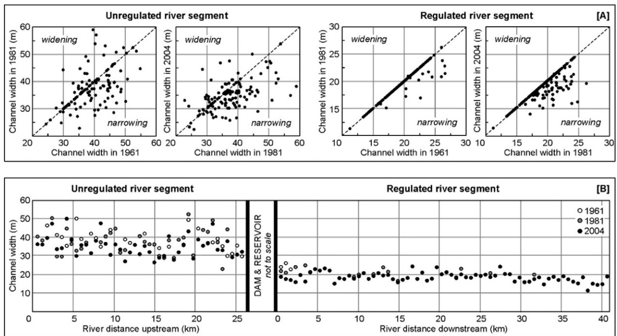
Fig. 6. [A] Scatterplots comparing the river channel width between consecutive time steps, and [B] river channel width as a function of time and distance downstream. Channel width was calculated as a function of channel area divided by 200-m length along each river segment. The hashed central line in [A] indicates a situation of no change between consecutive time steps. Data in [B] were reduced to improve readability (1 point every 600 m of channel length). The error margin for an exceedance probability of 10% is 4.8 m.
