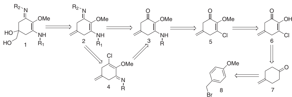
Fig. 14: Retrosynthesis proposed in the WO0239974A1 patent.
