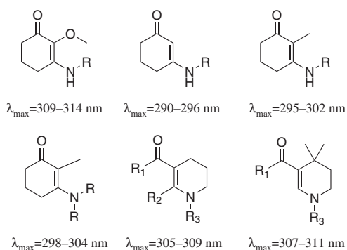
Fig. 13: Substituent effect in second and third generation of MAA analogues.
