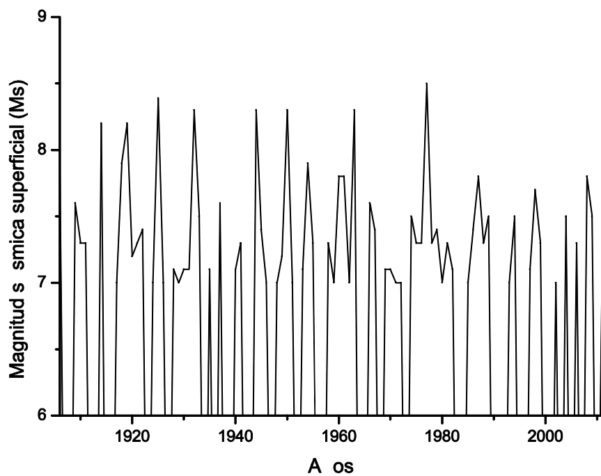
Figura 1. Magnitud sísmica superficial de terremotos de Chile (valor medio anual) desde 1906 a 2011. Figure 1. Chile earthquakes surface seismic magnitude (annual average) since 1906 to 2011.
